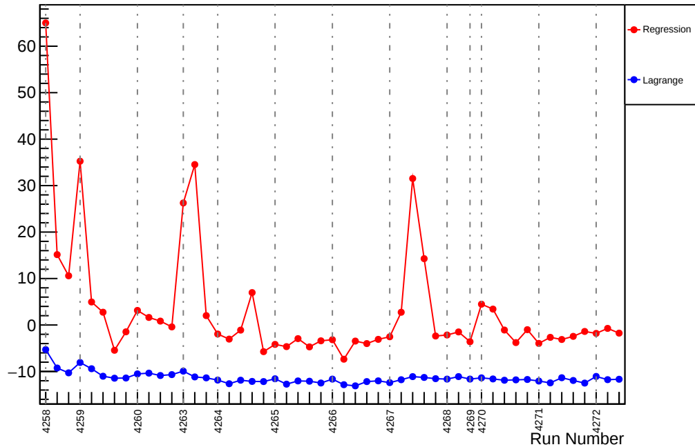
Slug51: Slope : usl_vs_evMon4 (ppm/um)
