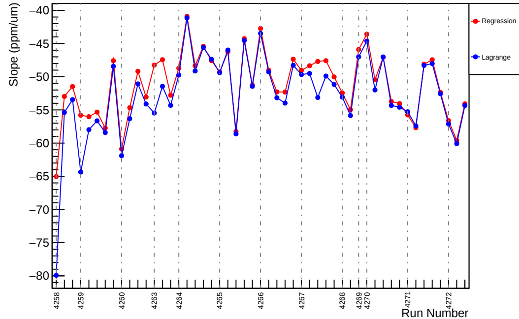
Slug51: Slope : usl_vs_evMon5 (ppm/um)
