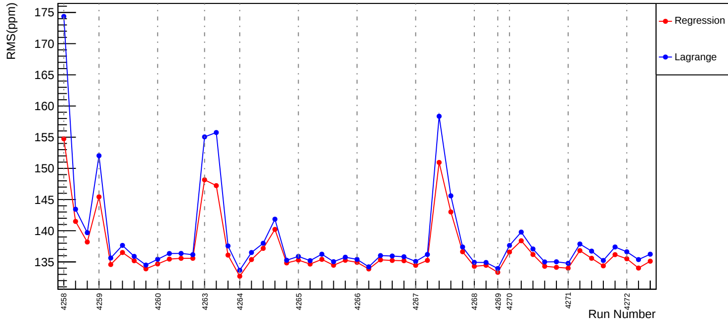
Slug51: Corrected RMS (ppm): asym_usl
