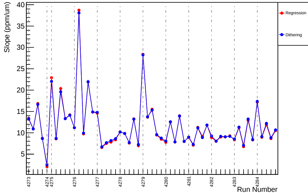
Slug52: Slope : usl_vs_evMon0 (ppm/um)
