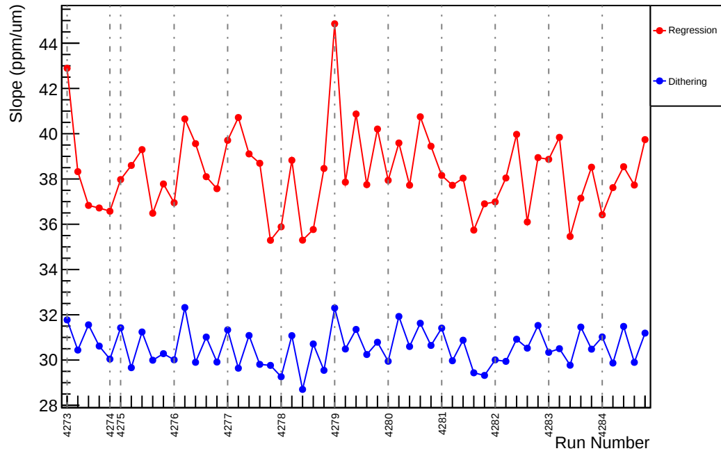
Slug52: Slope : usl_vs_evMon3 (ppm/um)
