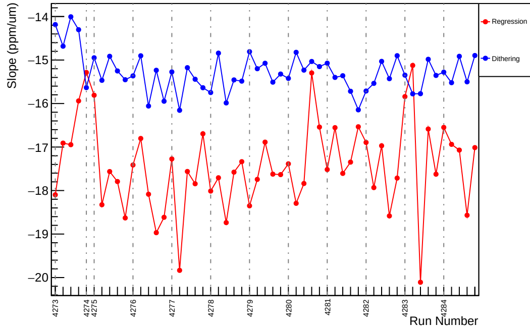
Slug52: Slope : usr_vs_evMon3 (ppm/um)
