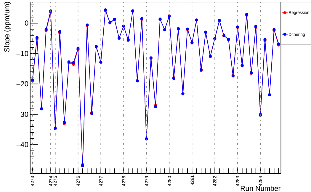
Slug52: Slope : usr_vs_evMon0 (ppm/um)
