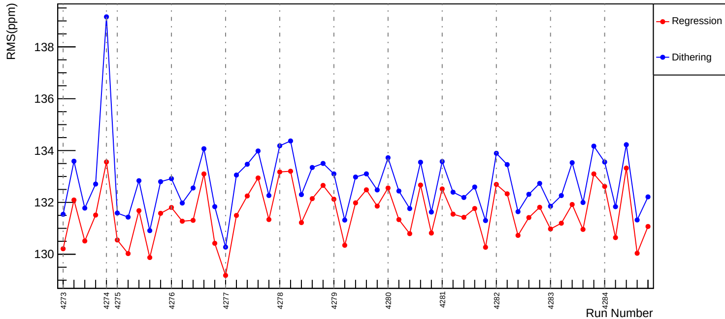
Slug52: Corrected RMS (ppm): asym_usr
