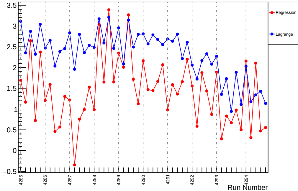
Slug53: Slope : usr_vs_evMon3 (ppm/um)
