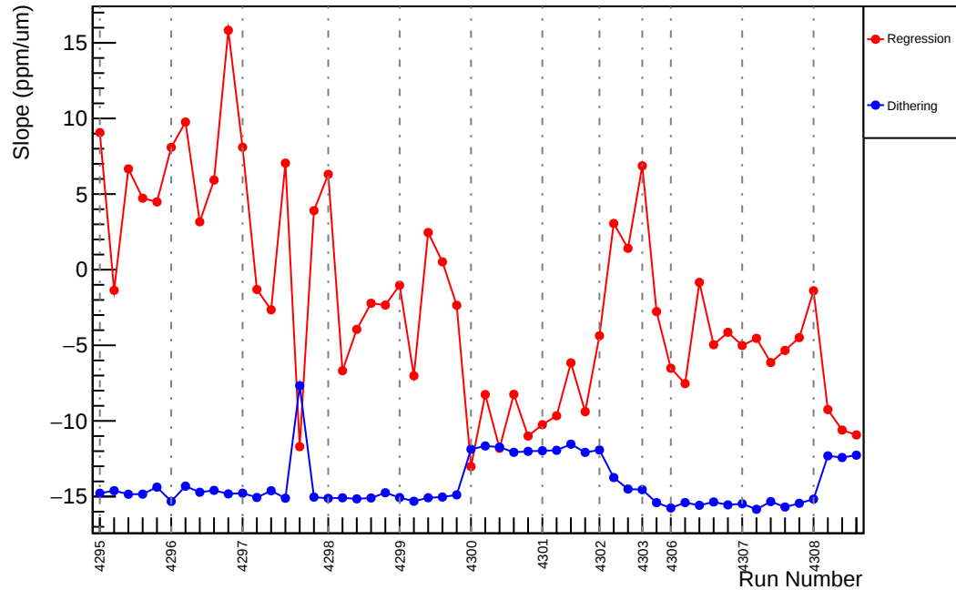
Slug54: Slope : us_avg_vs_evMon4 (ppm/um)
