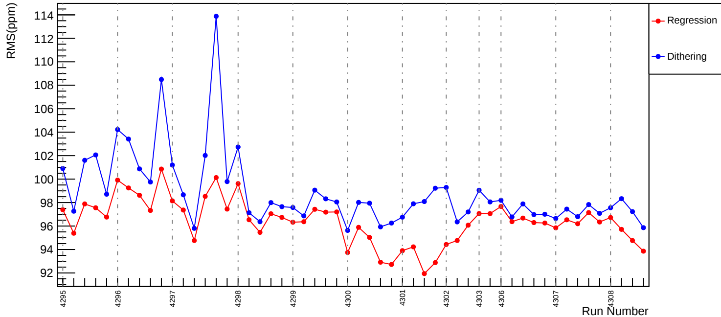
Slug54: Corrected RMS (ppm): asym_us_avg
