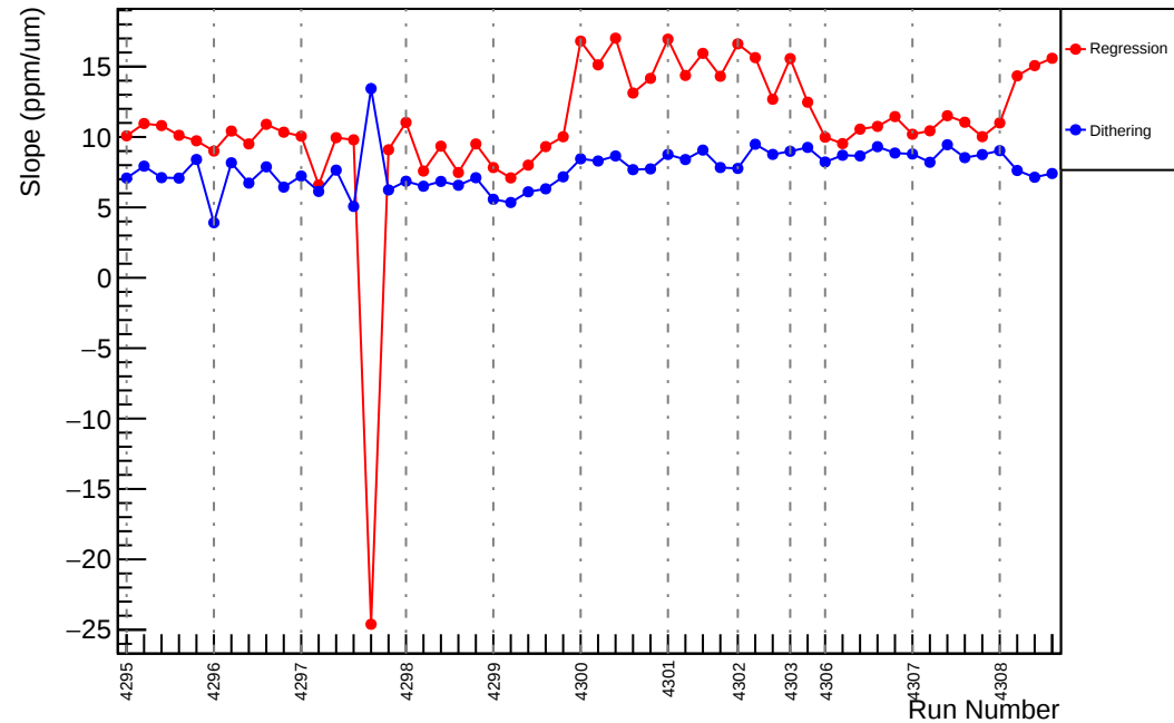
Slug54: Slope : us_avg_vs_evMon3 (ppm/um)
