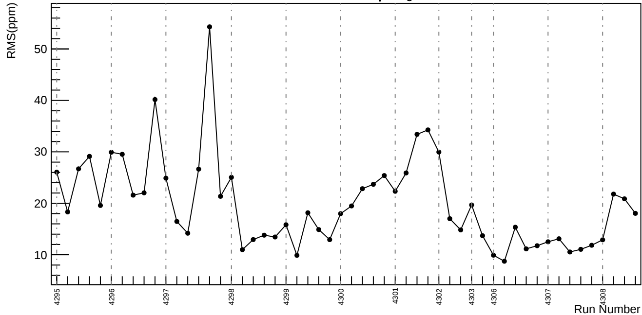
Slug54: asym_us_avg: \sqrt{\sigma_{\text{lagr}}^2 - \sigma_{\text{reg}}^2} (ppm)
