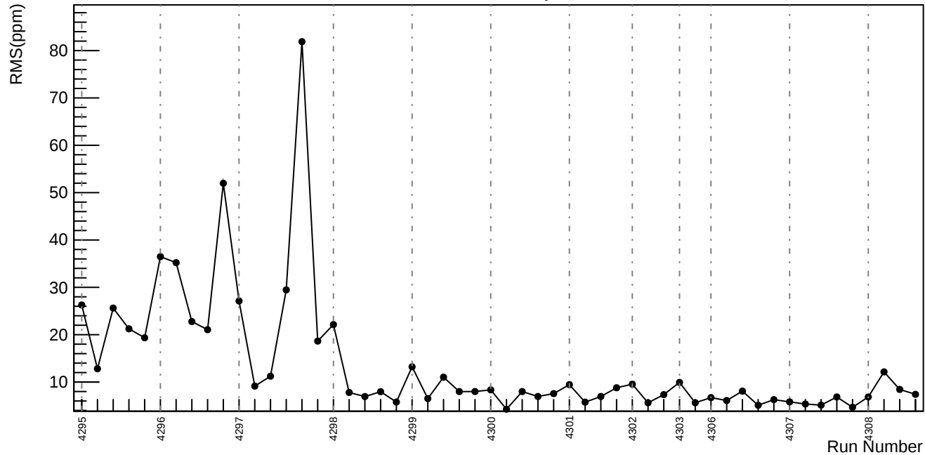
Slug54: asym_us_dd: \sqrt{\sigma_{\text{dit}}^2 - \sigma_{\text{reg}}^2} (ppm)
