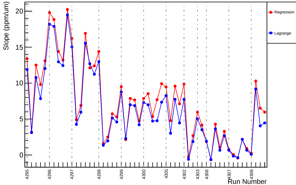
Slug54: Slope : us_dd_vs_evMon6 (ppm/um)
