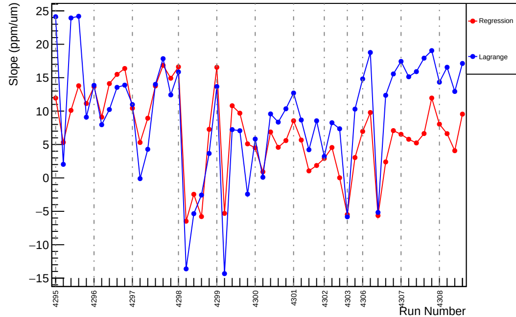
Slug54: Slope : us_dd_vs_evMon9 (ppm/um)
