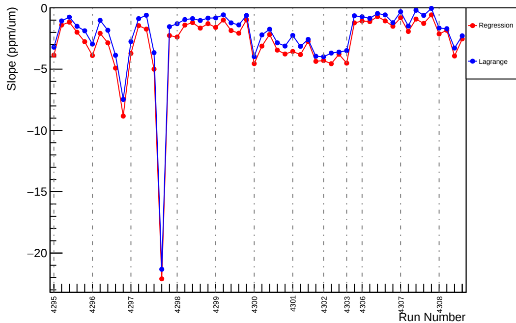
Slug54: Slope : us_dd_vs_evMon5 (ppm/um)
