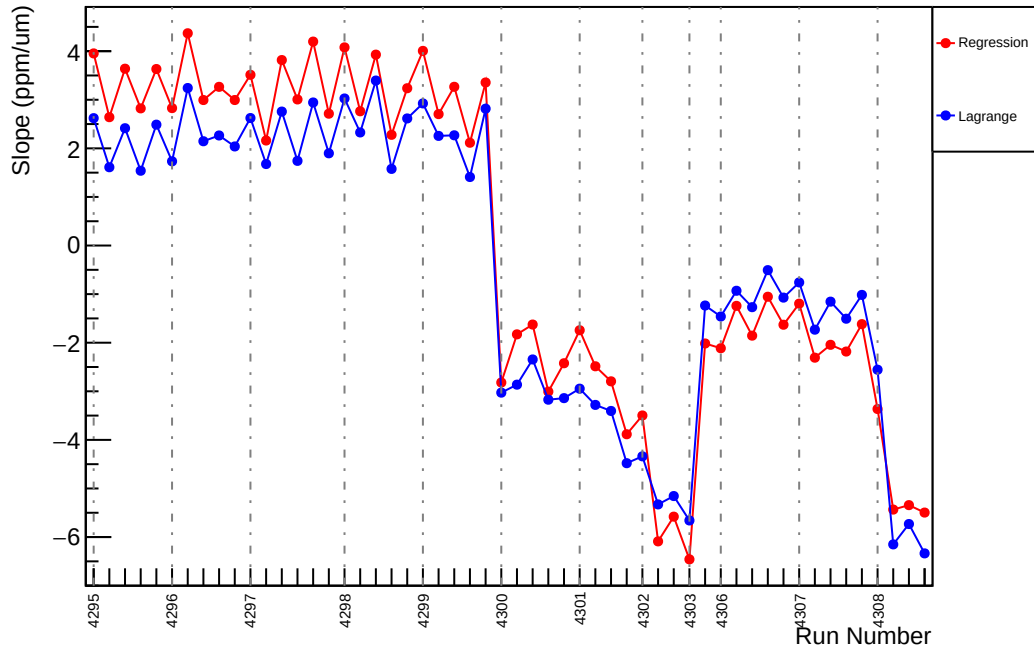
Slug54: Slope : us_dd_vs_evMon3 (ppm/um)
