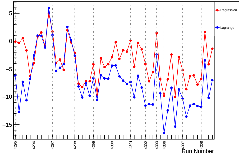
Slug54: Slope : us_dd_vs_evMon8 (ppm/um)
