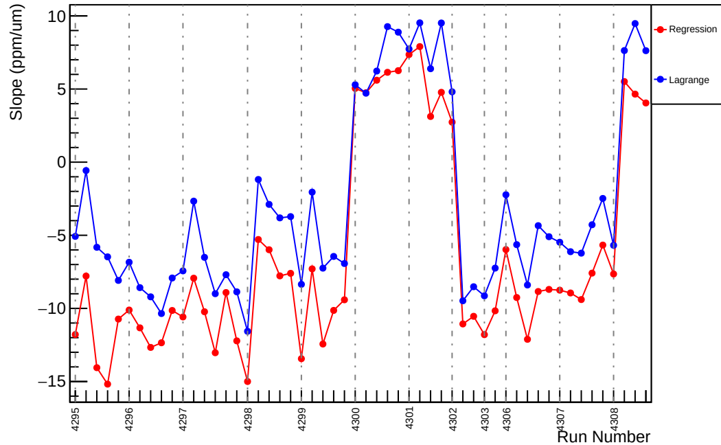
Slug54: Slope : us_dd_vs_evMon7 (ppm/um)
