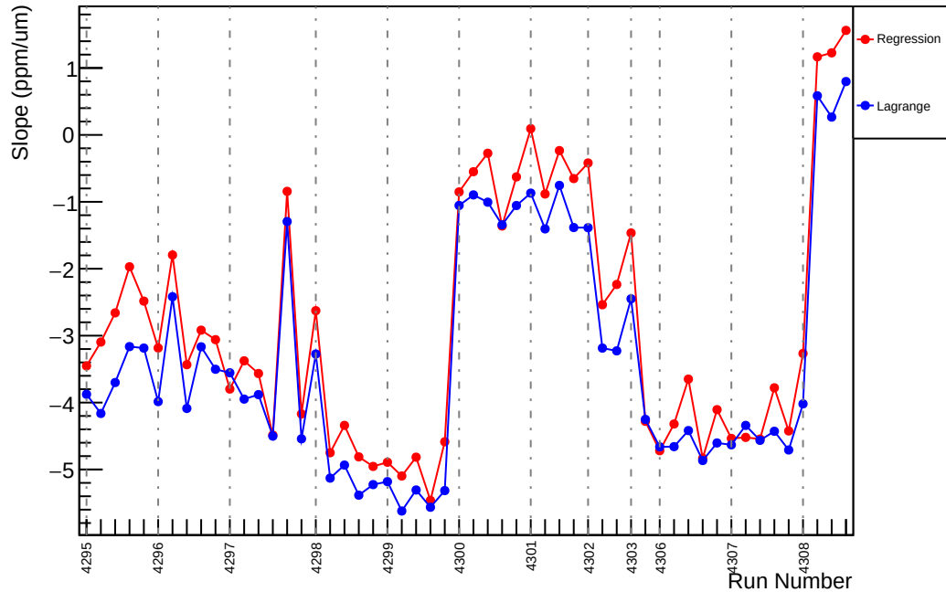
Slug54: Slope : us_dd_vs_evMon4 (ppm/um)
