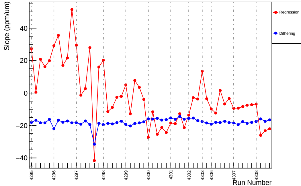
Slug54: Slope : usl_vs_evMon4 (ppm/um)
