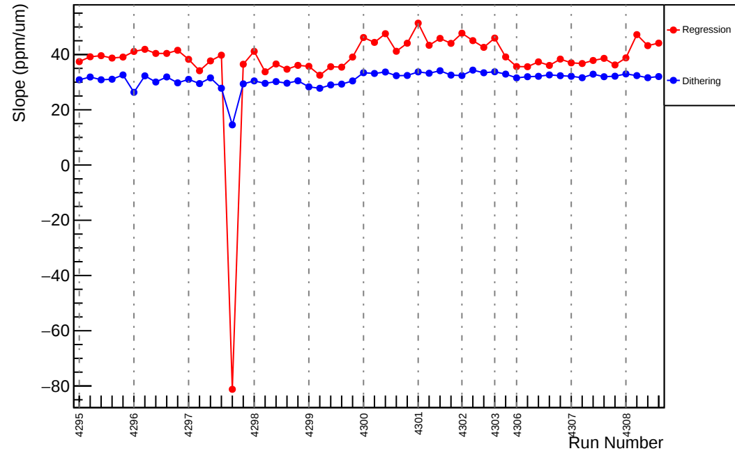
Slug54: Slope : usl_vs_evMon3 (ppm/um)
