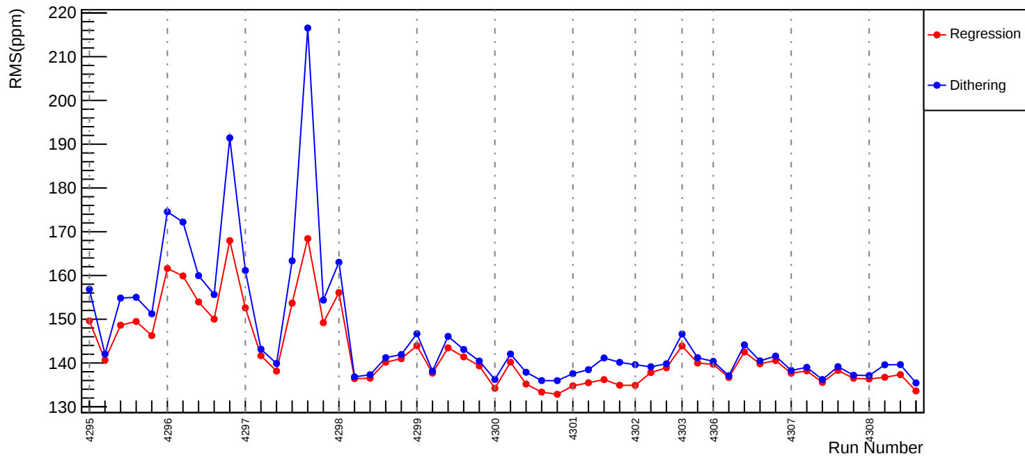
Slug54: Corrected RMS (ppm): asym_usl
