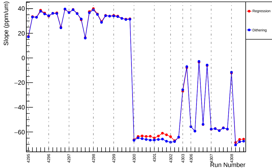
Slug54: Slope : usl_vs_evMon1 (ppm/um)
