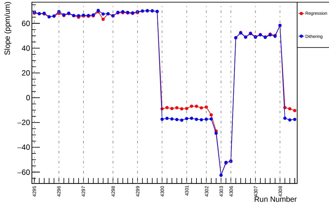
Slug54: Slope : usl_vs_evMon2 (ppm/um)
