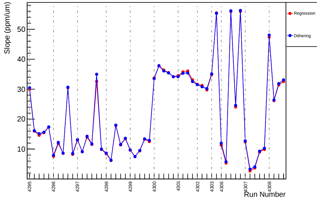
Slug54: Slope : usl_vs_evMon0 (ppm/um)
