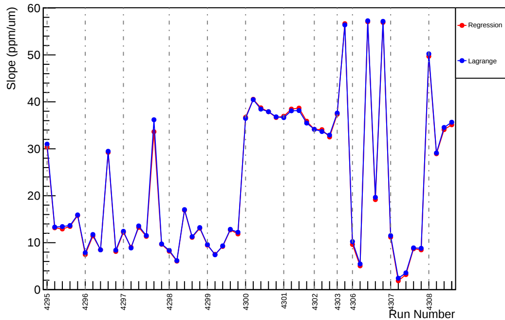
Slug54: Slope : usl_vs_evMon0 (ppm/um)
