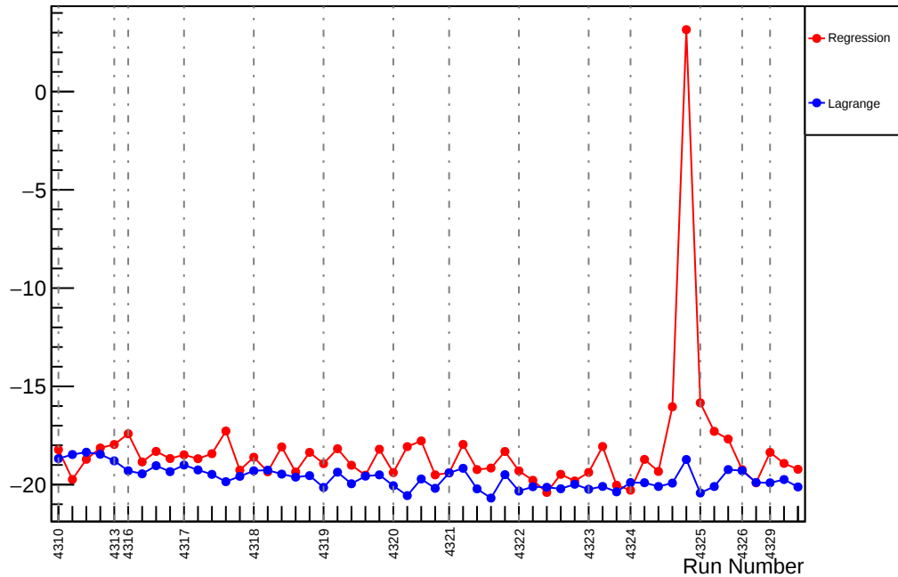
Slug55: Slope : us_dd_vs_evMon3 (ppm/um)
