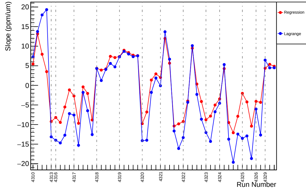
Slug55: Slope : us_dd_vs_evMon10 (ppm/um)
