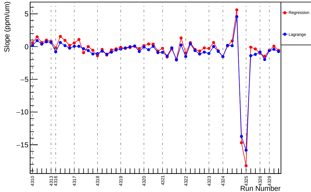
Slug55: Slope : us_dd_vs_evMon5 (ppm/um)
