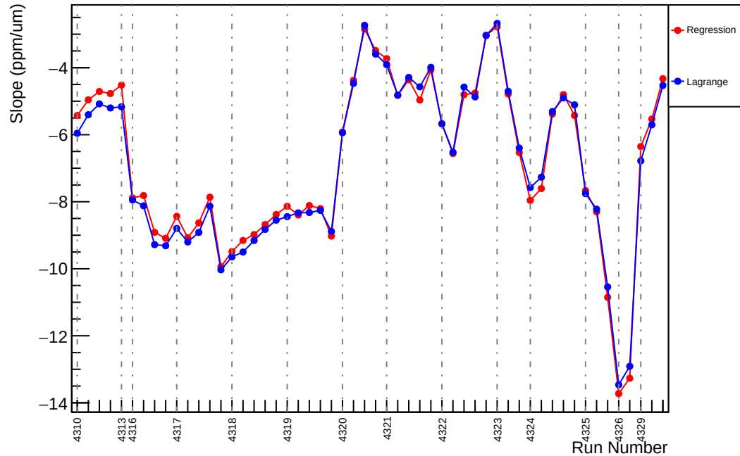
Slug55: Slope : us_dd_vs_evMon1 (ppm/um)
