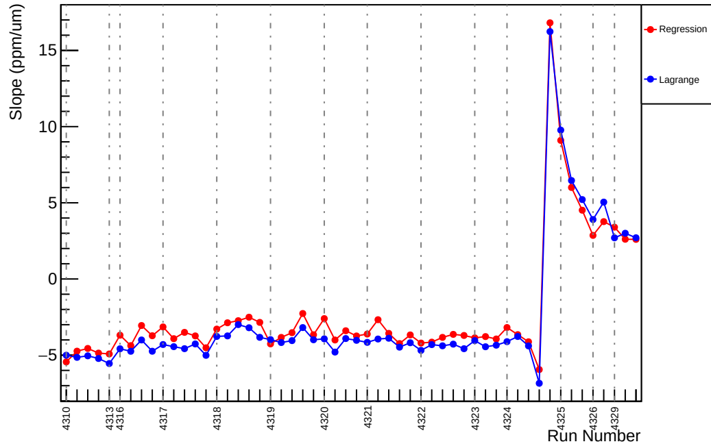
Slug55: Slope : us_dd_vs_evMon3 (ppm/um)
