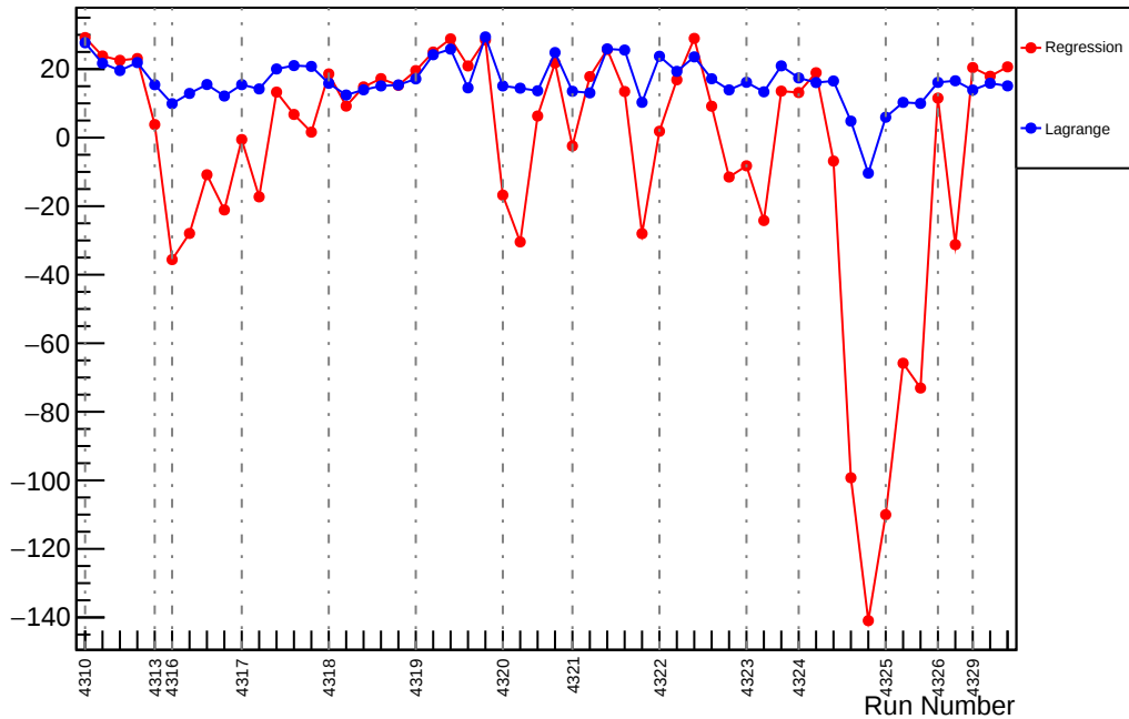
Slug55: Slope : usl_vs_evMon4 (ppm/um)
