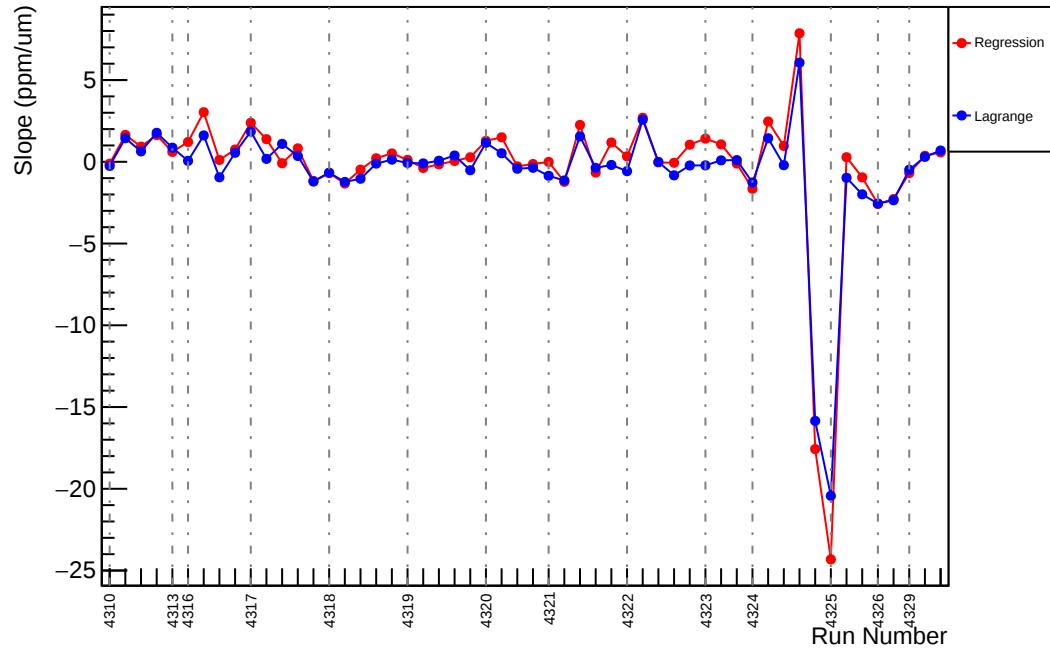
Slug55: Slope : usl_vs_evMon5 (ppm/um)
