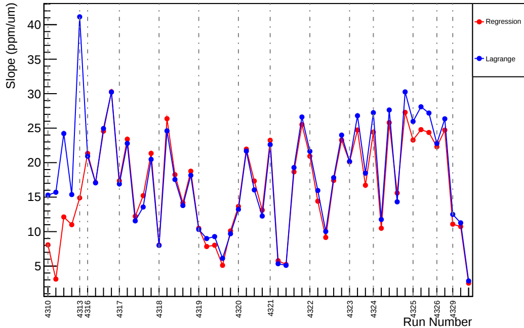
Slug55: Slope : usl_vs_evMon11 (ppm/um)
