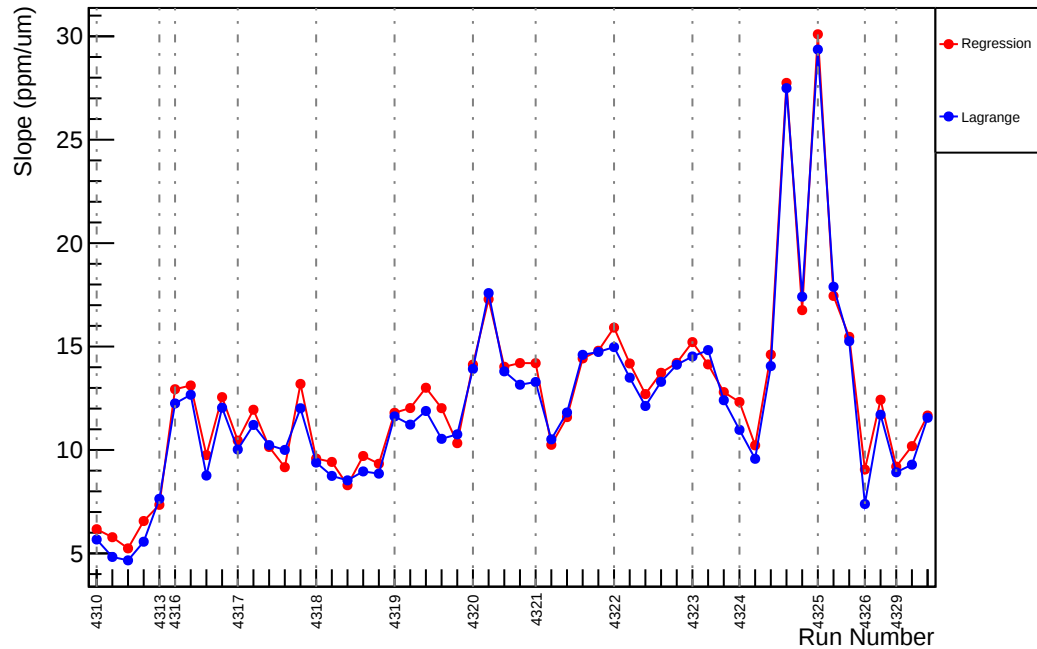
Slug55: Slope : usl_vs_evMon4 (ppm/um)
