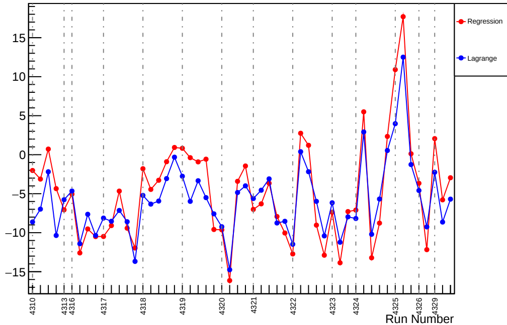
Slug55: Slope : usl_vs_evMon8 (ppm/um)
