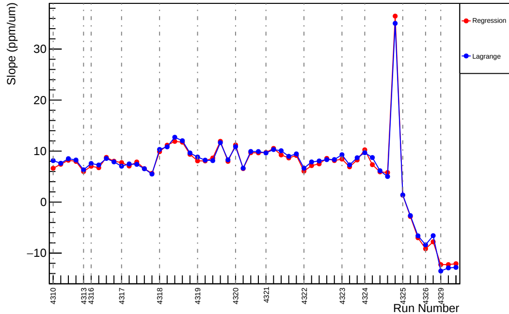
Slug55: Slope : usl_vs_evMon3 (ppm/um)
