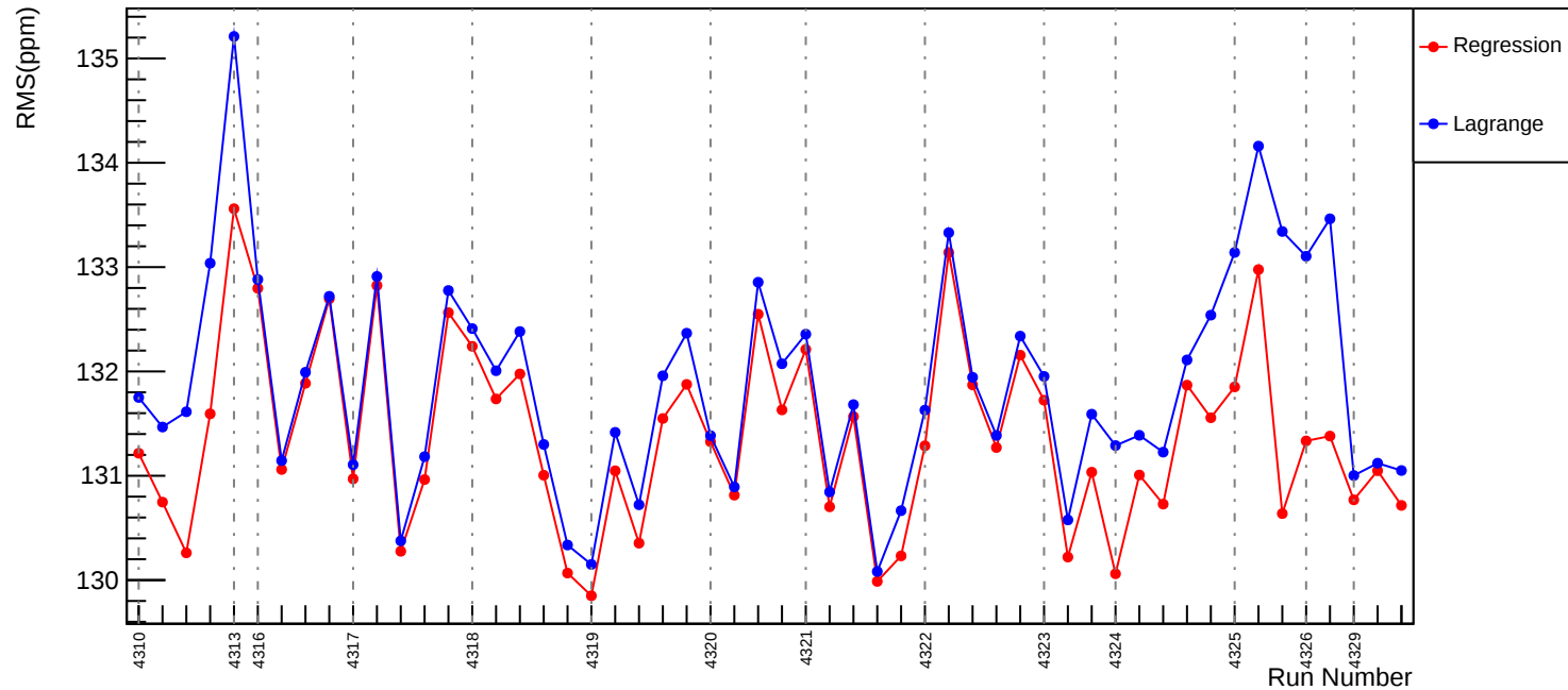
Slug55: Corrected RMS (ppm): asym_usl
