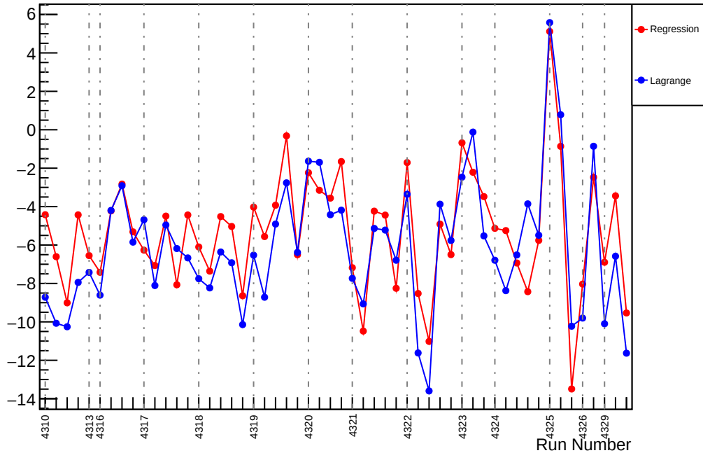
Slug55: Slope : usl_vs_evMon7 (ppm/um)
