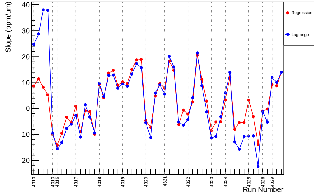
Slug55: Slope : usl_vs_evMon10 (ppm/um)
