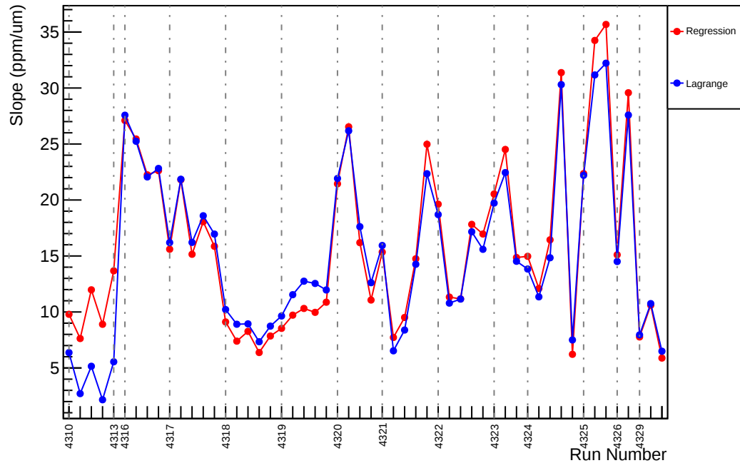
Slug55: Slope : usl_vs_evMon6 (ppm/um)
