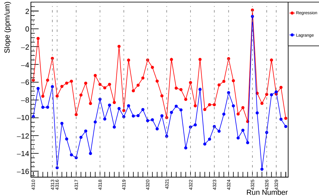
Slug55: Slope : usr_vs_evMon7 (ppm/um)
