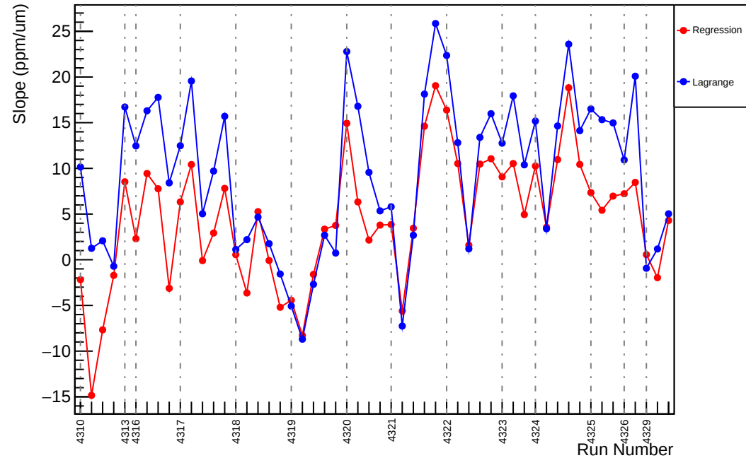
Slug55: Slope : usr_vs_evMon10 (ppm/um)
