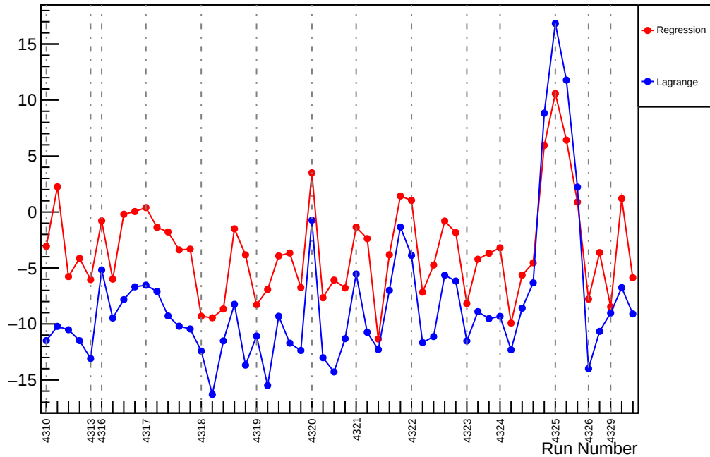
Slug55: Slope : usr_vs_evMon8 (ppm/um)
