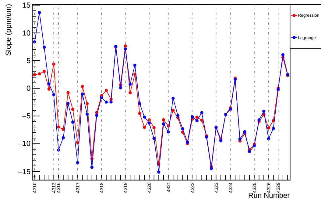
Slug55: Slope : usr_vs_evMon11 (ppm/um)
