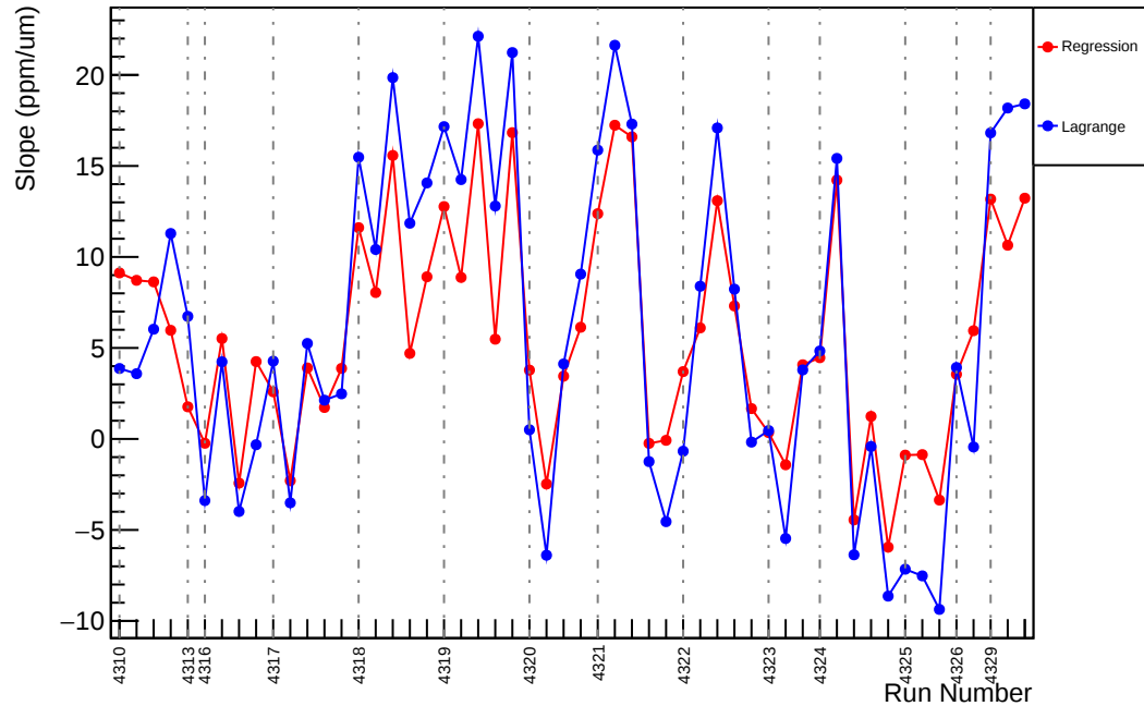
Slug55: Slope : usr_vs_evMon9 (ppm/um)
