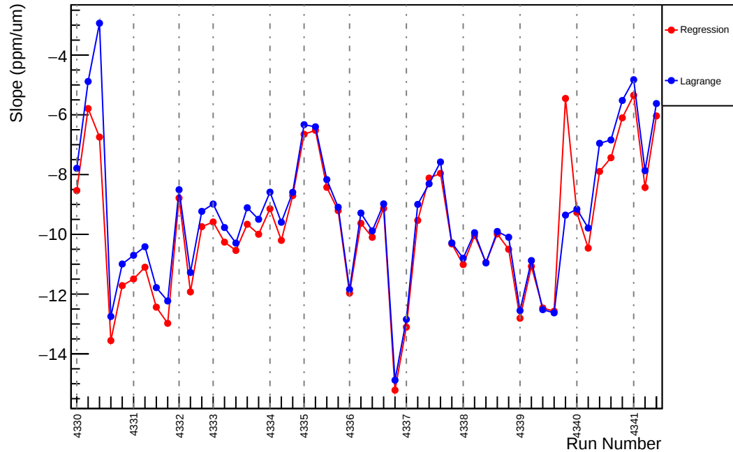
Slug56: Slope : us_avg_vs_evMon0 (ppm/um)
