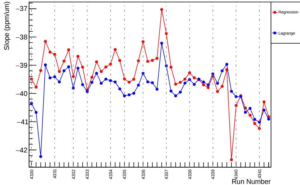
Slug56: Slope : us_avg_vs_evMon1 (ppm/um)
