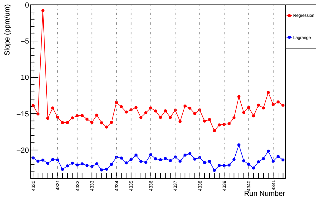
Slug56: Slope : us_avg_vs_evMon2 (ppm/um)
