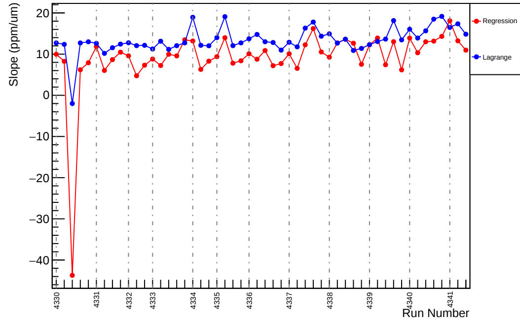
Slug56: Slope : us_avg_vs_evMon4 (ppm/um)
