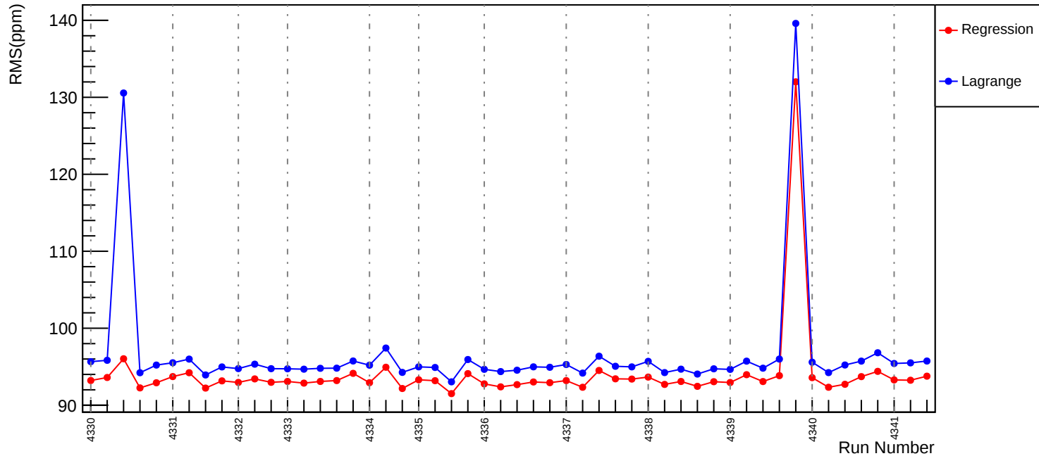
Slug56: Corrected RMS (ppm): asym_us_avg
