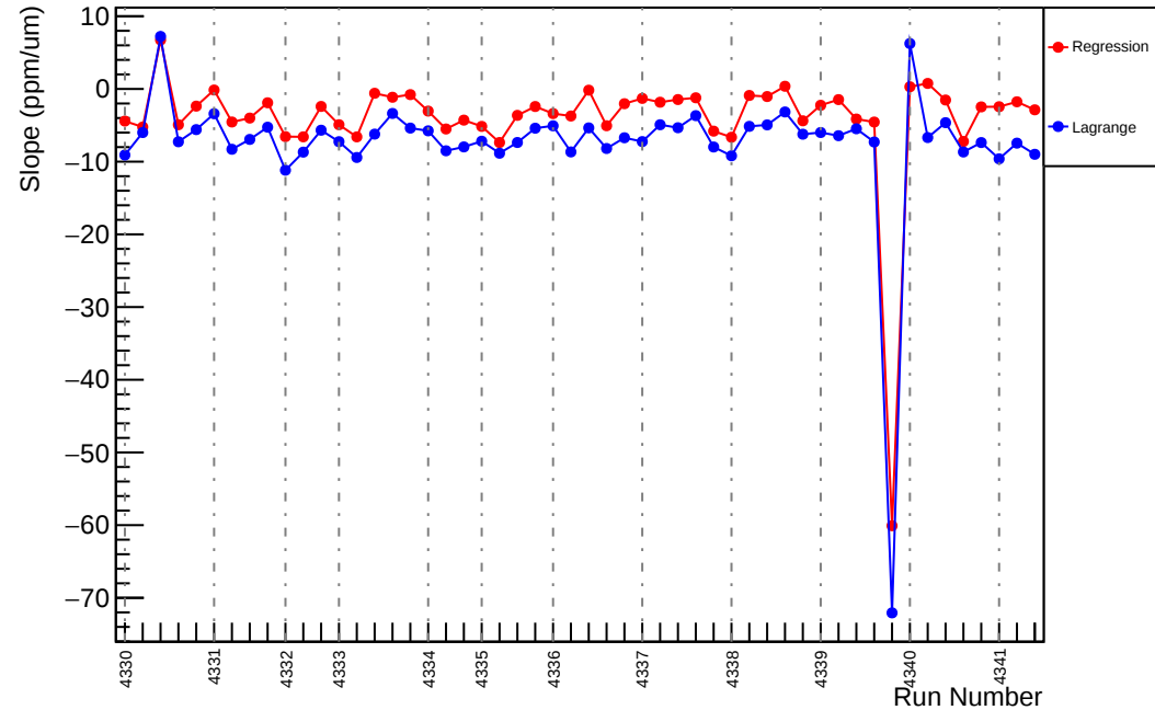
Slug56: Slope : us_avg_vs_evMon8 (ppm/um)
