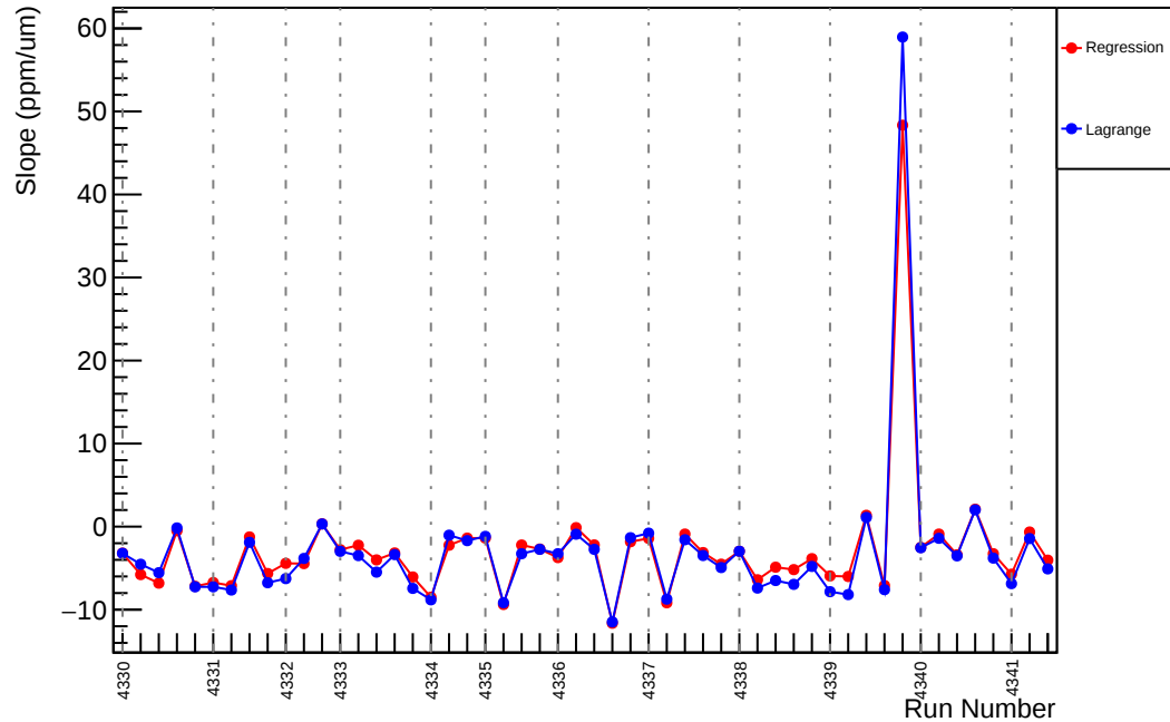
Slug56: Slope : us_avg_vs_evMon10 (ppm/um)
