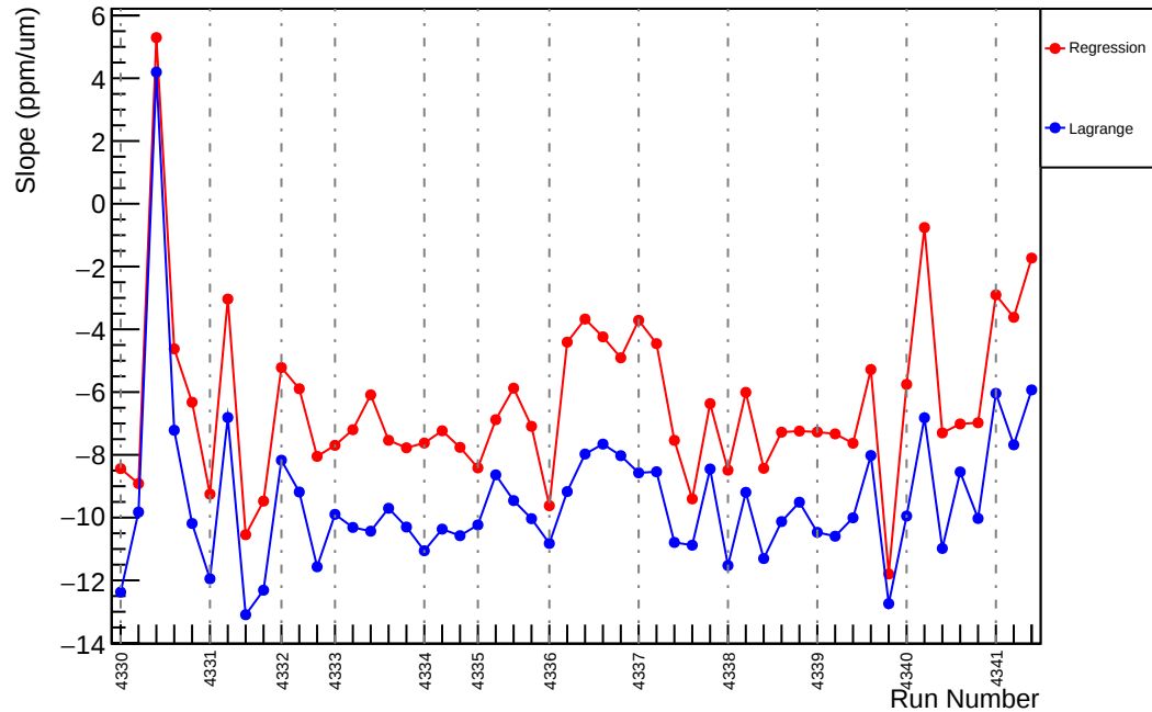
Slug56: Slope : us_avg_vs_evMon7 (ppm/um)
