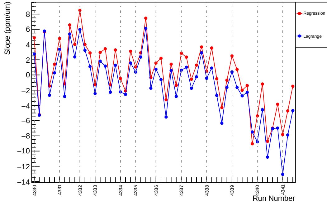
Slug56: Slope : us_avg_vs_evMon9 (ppm/um)
