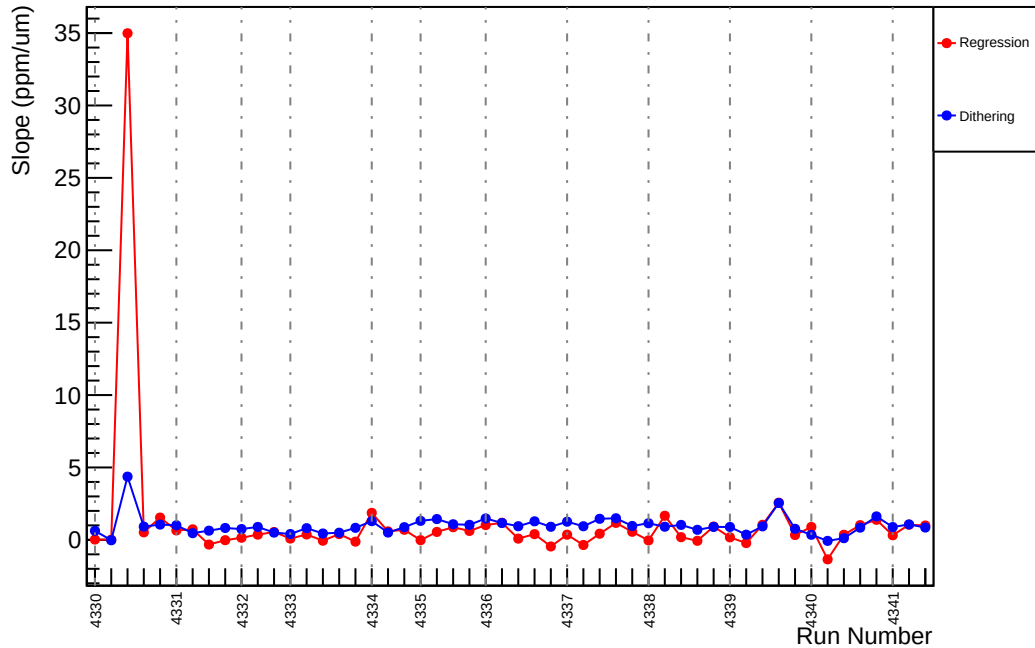
Slug56: Slope : us_dd_vs_evMon2 (ppm/um)
