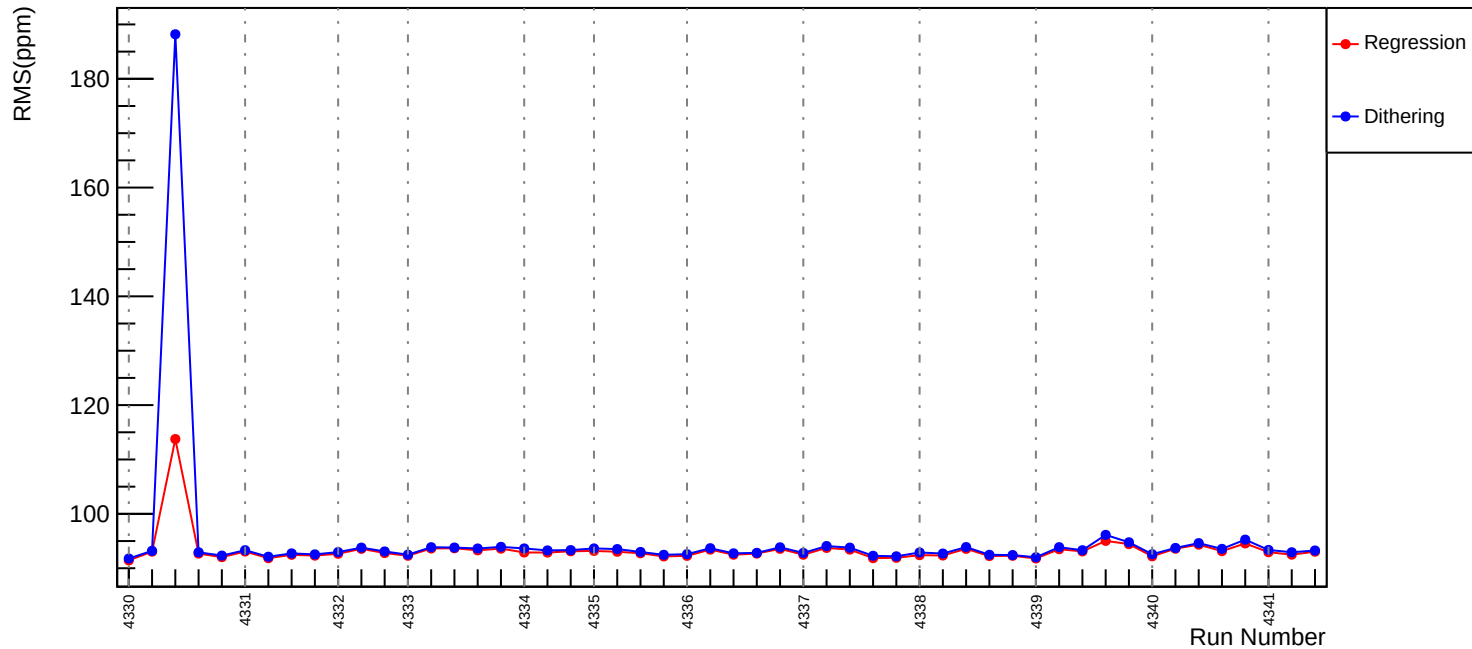
Slug56: Corrected RMS (ppm): asym_us_dd
