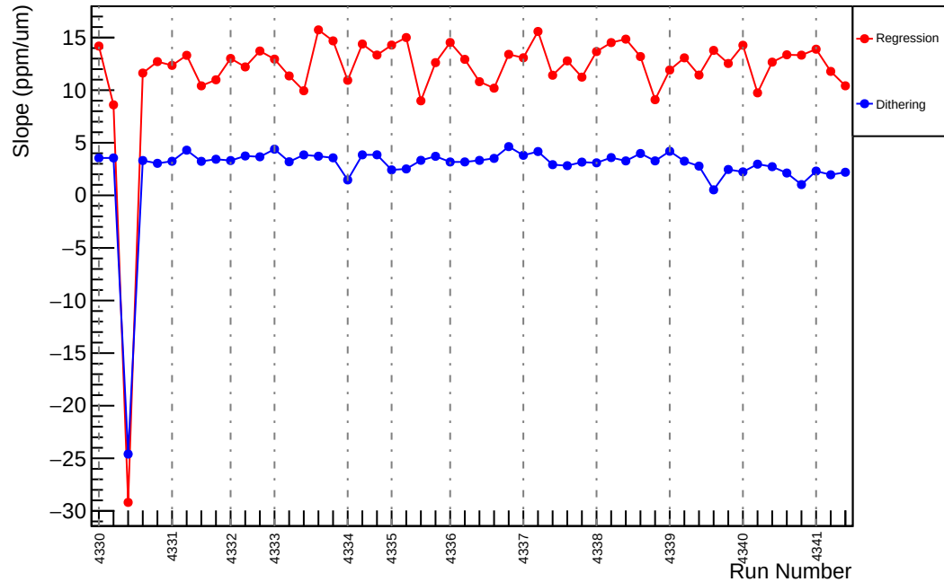
Slug56: Slope : us_dd_vs_evMon4 (ppm/um)
