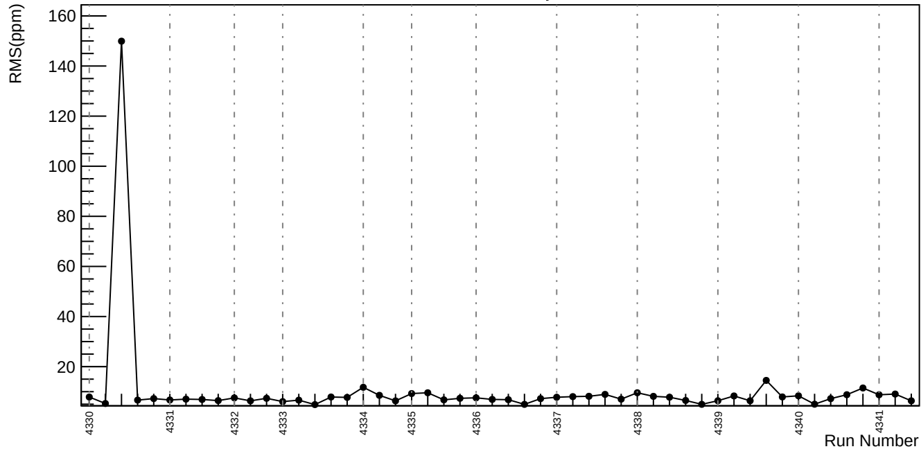
Slug56: asym_us_dd: \sqrt{\sigma_{\text{dit}}^2 - \sigma_{\text{reg}}^2} (ppm)
