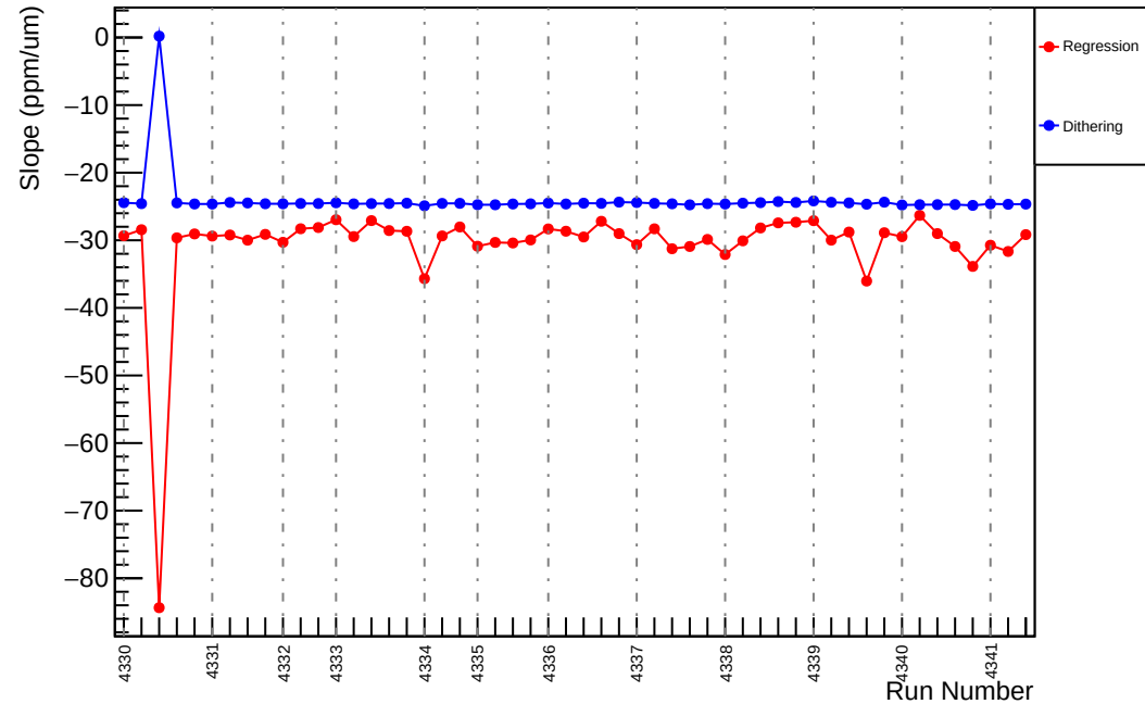
Slug56: Slope : us_dd_vs_evMon3 (ppm/um)
