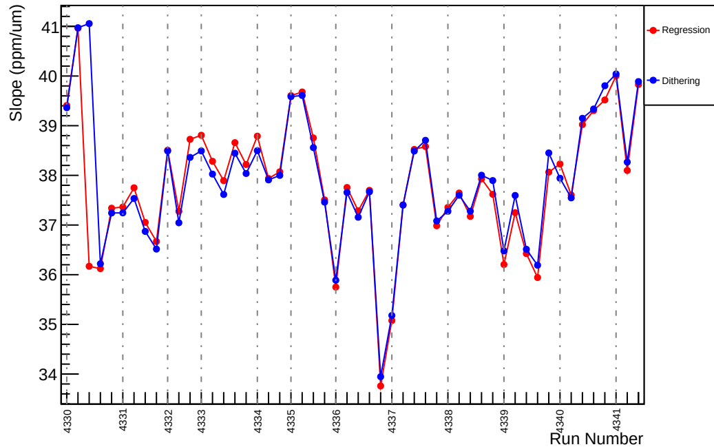
Slug56: Slope : us_dd_vs_evMon0 (ppm/um)
