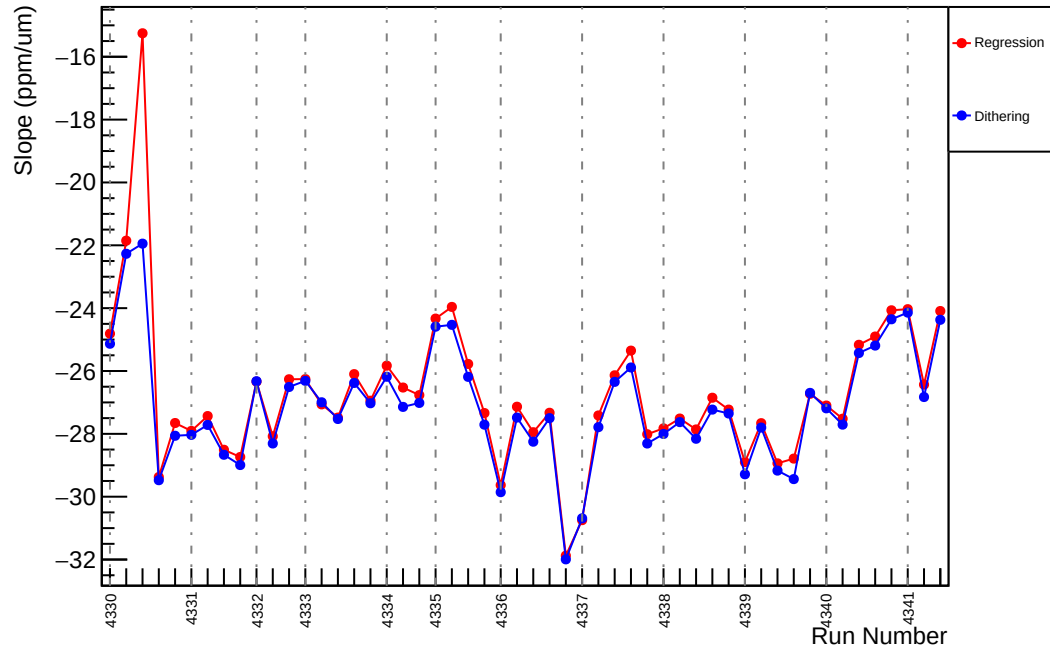
Slug56: Slope : us_dd_vs_evMon1 (ppm/um)
