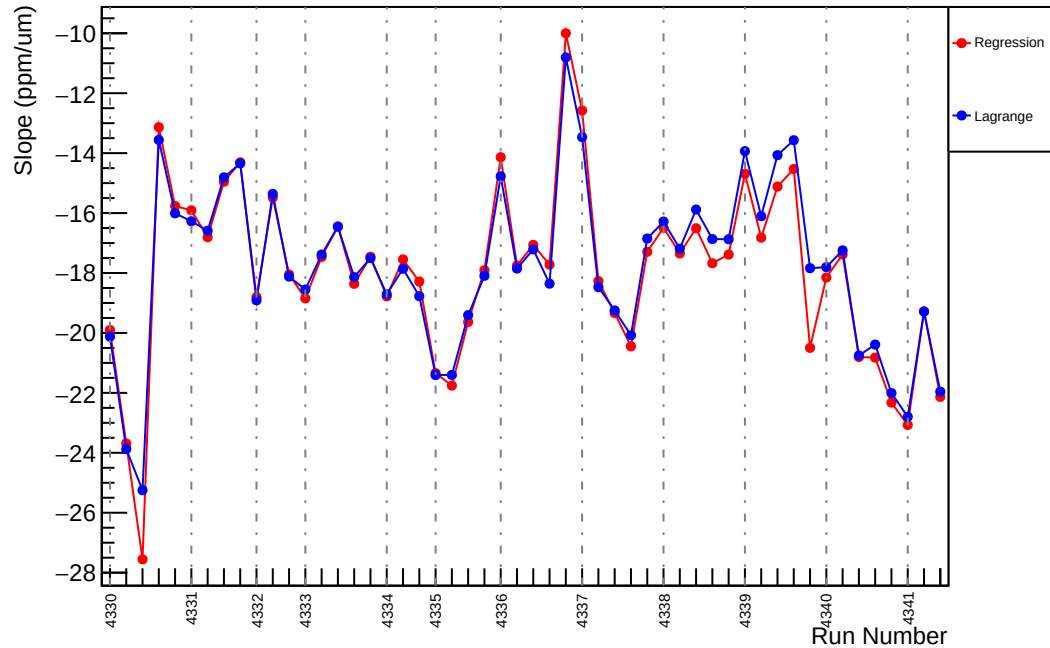
Slug56: Slope : usr_vs_evMon1 (ppm/um)
