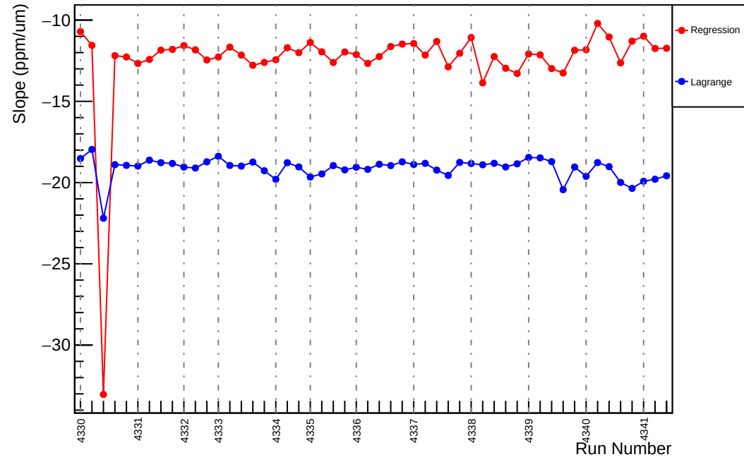
Slug56: Slope : usr_vs_evMon2 (ppm/um)
