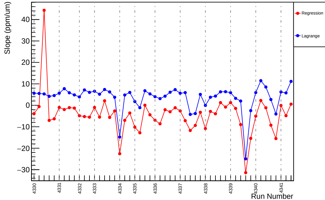
Slug56: Slope : usr_vs_evMon4 (ppm/um)
