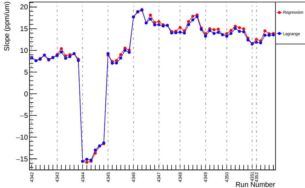
Slug57: Slope : us_avg_vs_evMon3 (ppm/um)
