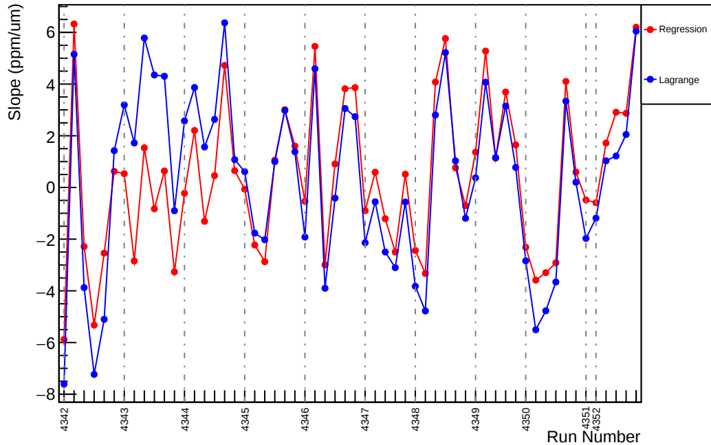
Slug57: Slope : us_avg_vs_evMon10 (ppm/um)
