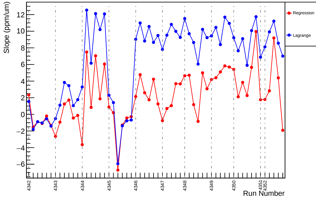
Slug57: Slope : us_avg_vs_evMon8 (ppm/um)
