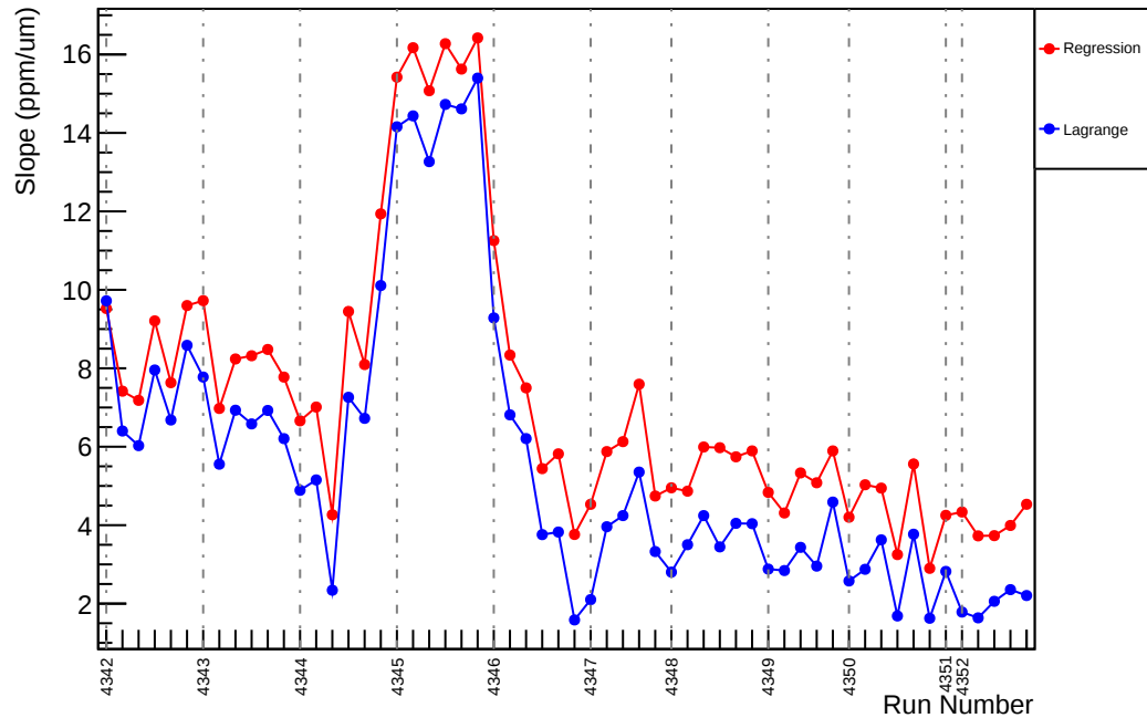
Slug57: Slope : us_avg_vs_evMon4 (ppm/um)
