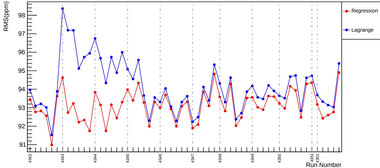
Slug57: Corrected RMS (ppm): asym_us_avg
