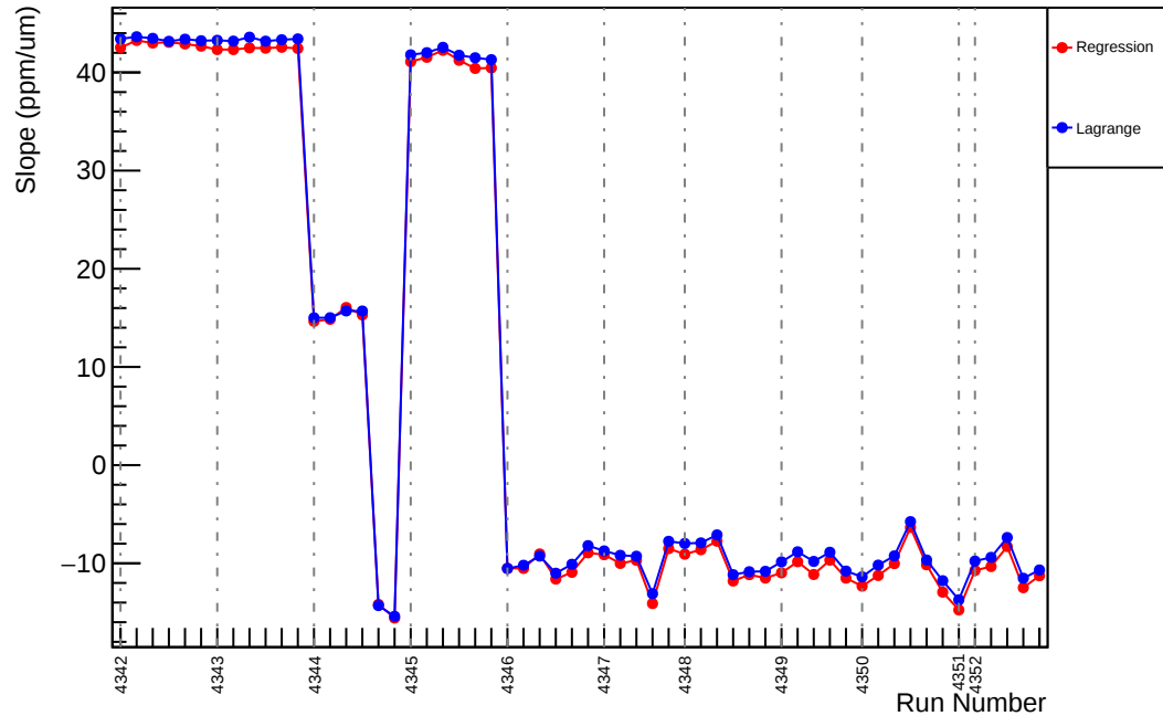
Slug57: Slope : us_avg_vs_evMon2 (ppm/um)
