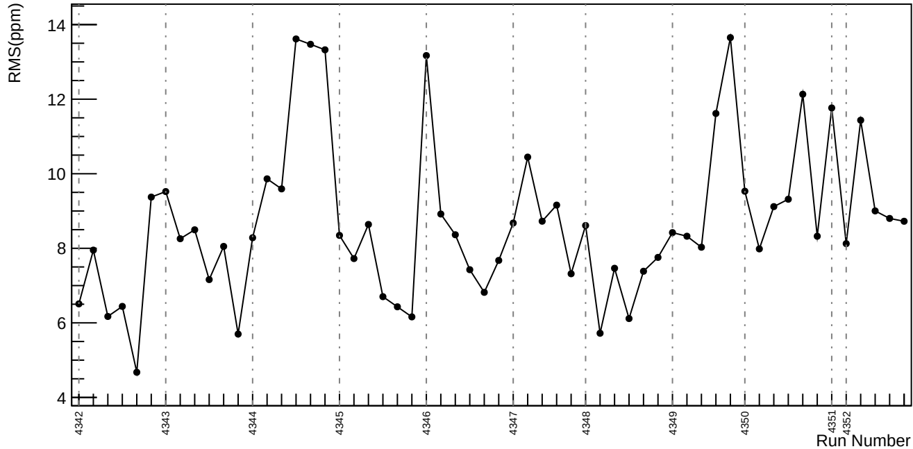
Slug57: asym_us_dd: \sqrt{\sigma_{\text{dit}}^2 - \sigma_{\text{reg}}^2} (ppm)
