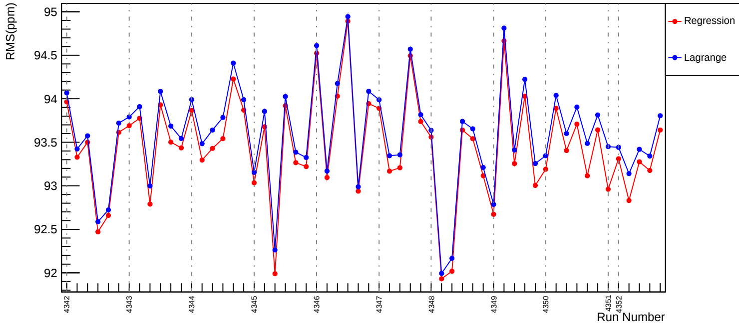
Slug57: Corrected RMS (ppm): asym_us_dd
