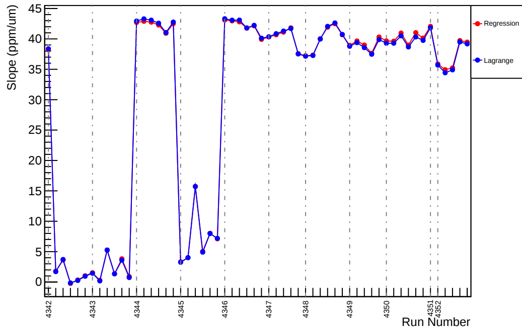
Slug57: Slope : us_dd_vs_evMon0 (ppm/um)
