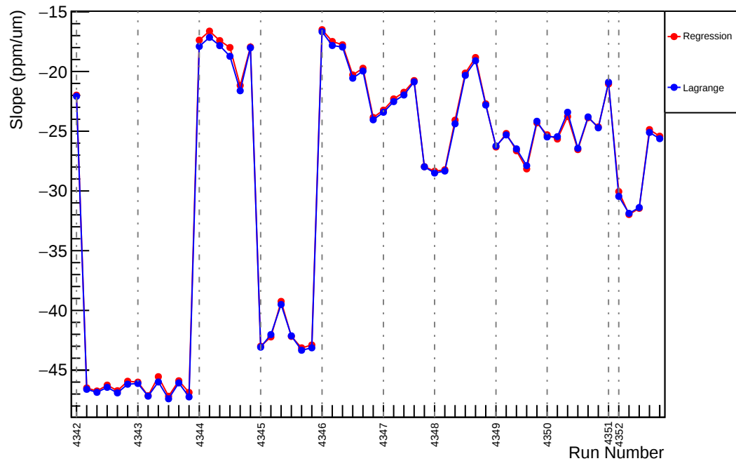
Slug57: Slope : us_dd_vs_evMon1 (ppm/um)
