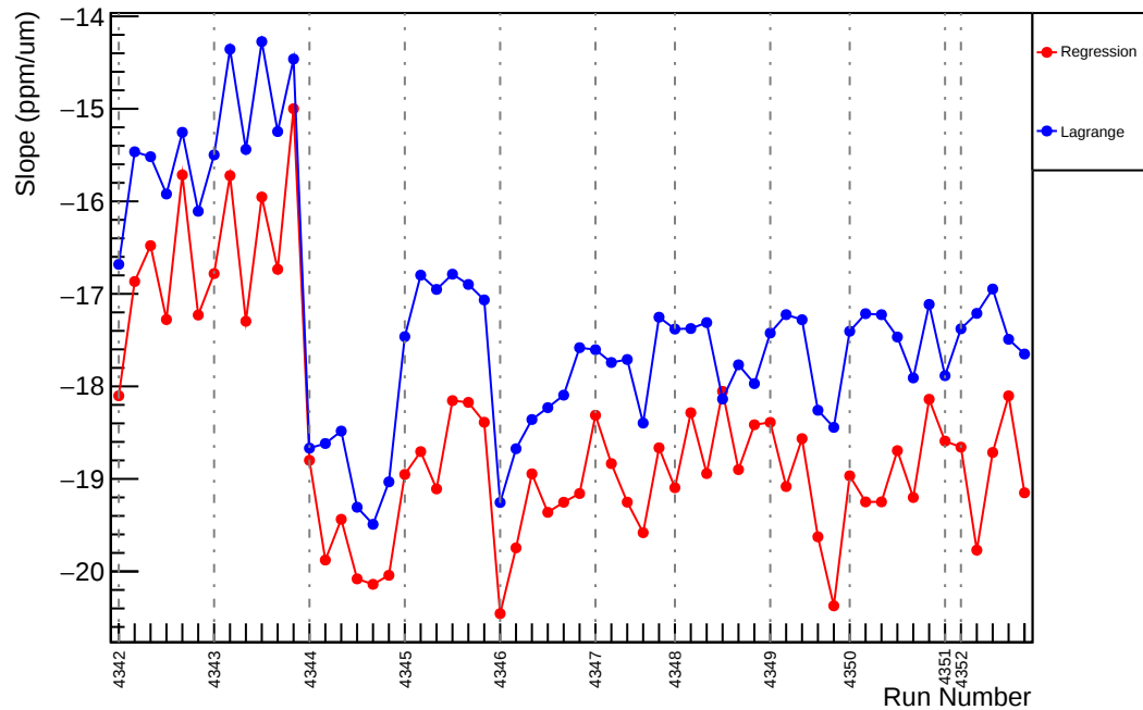
Slug57: Slope : us_dd_vs_evMon3 (ppm/um)
