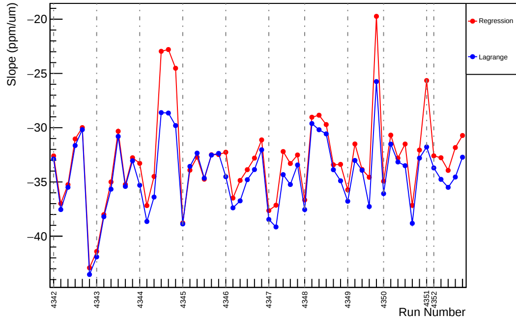
Slug57: Slope : us_dd_vs_evMon5 (ppm/um)
