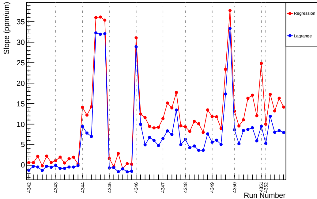
Slug57: Slope : us_dd_vs_evMon4 (ppm/um)
