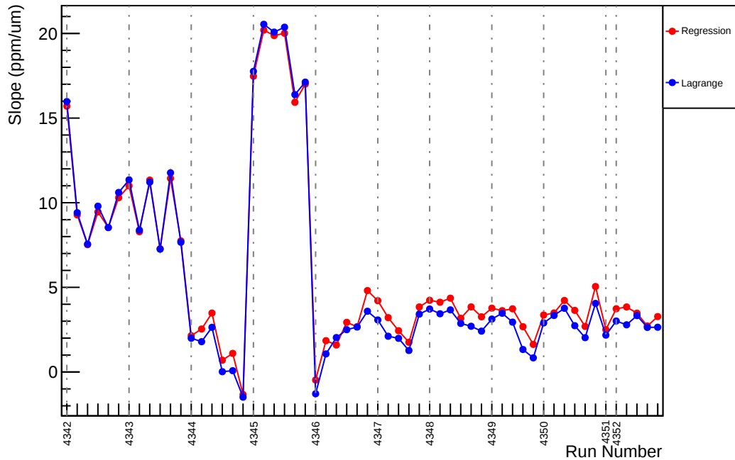
Slug57: Slope : us_dd_vs_evMon2 (ppm/um)
