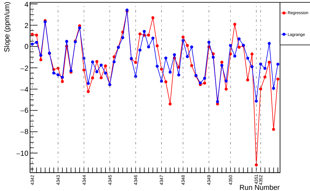
Slug57: Slope : us_dd_vs_evMon8 (ppm/um)
