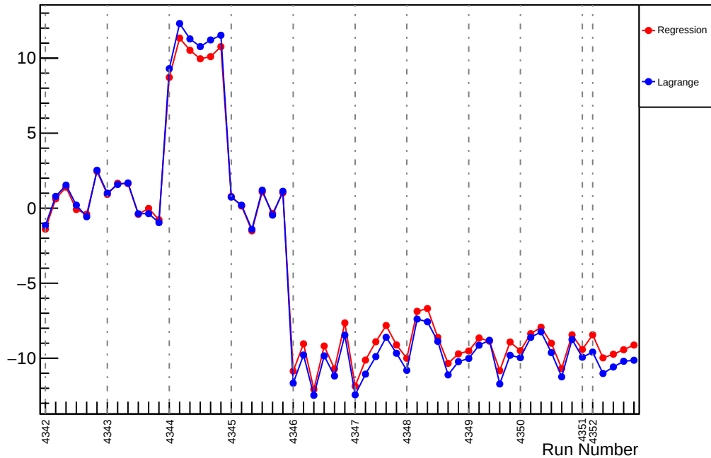
Slug57: Slope : us_dd_vs_evMon6 (ppm/um)
