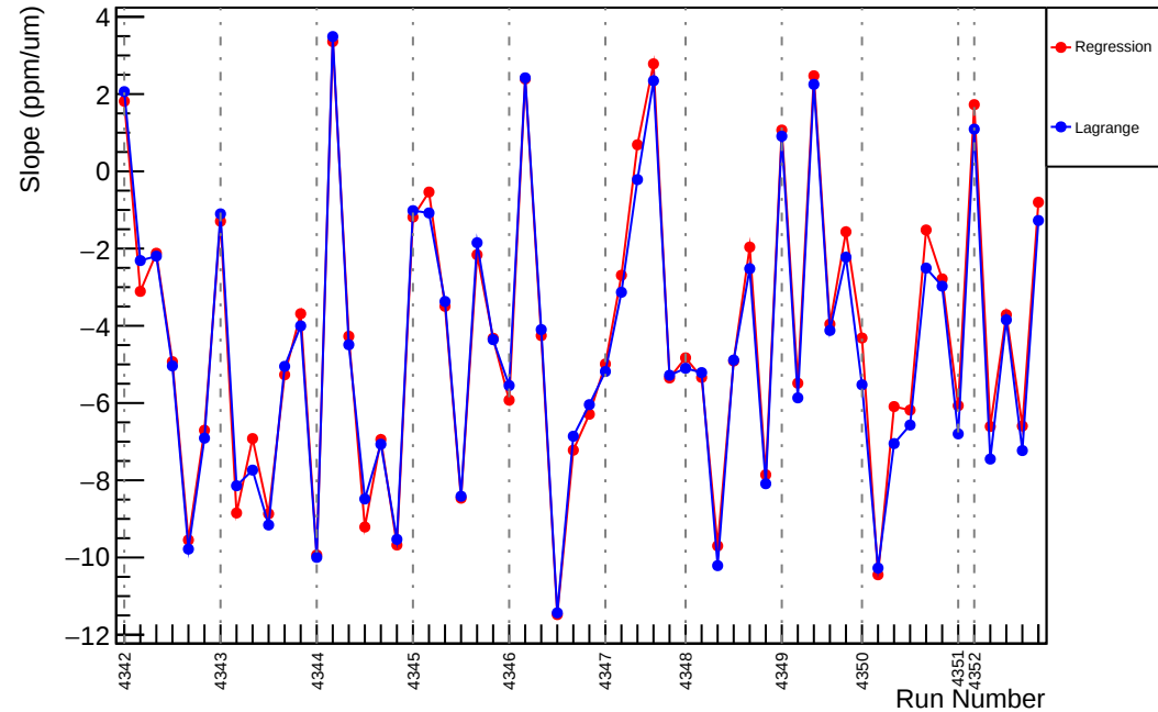
Slug57: Slope : us_dd_vs_evMon11 (ppm/um)
