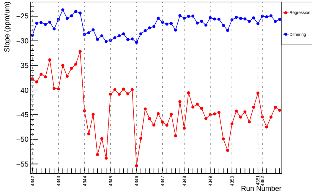
Slug57: Slope : usl_vs_evMon3 (ppm/um)
