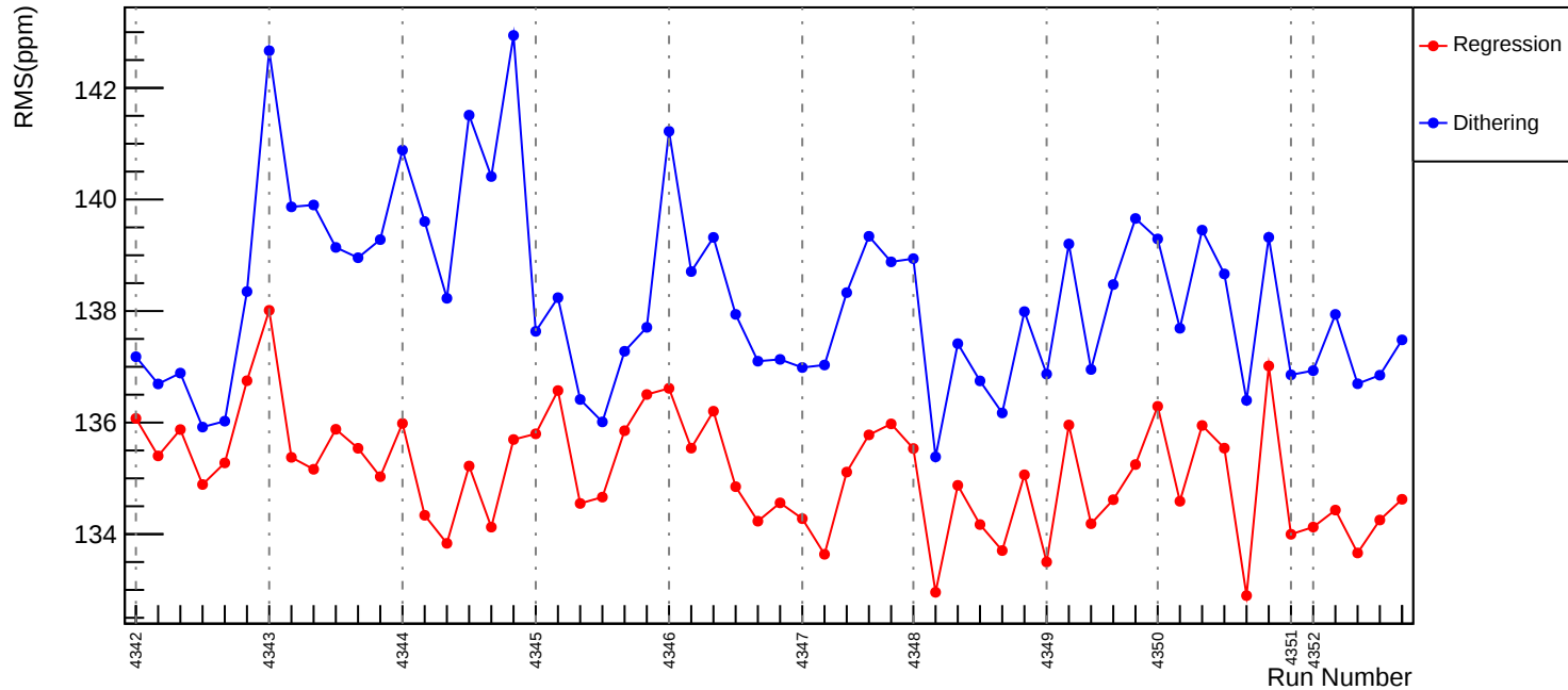
Slug57: Corrected RMS (ppm): asym_usl
