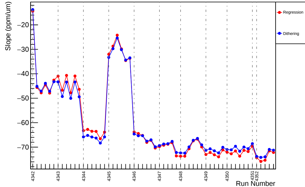
Slug57: Slope : usl_vs_evMon1 (ppm/um)
