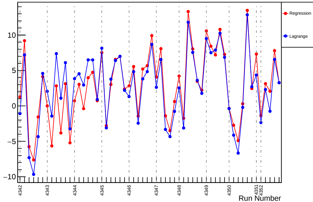
Slug57: Slope : usl_vs_evMon10 (ppm/um)
