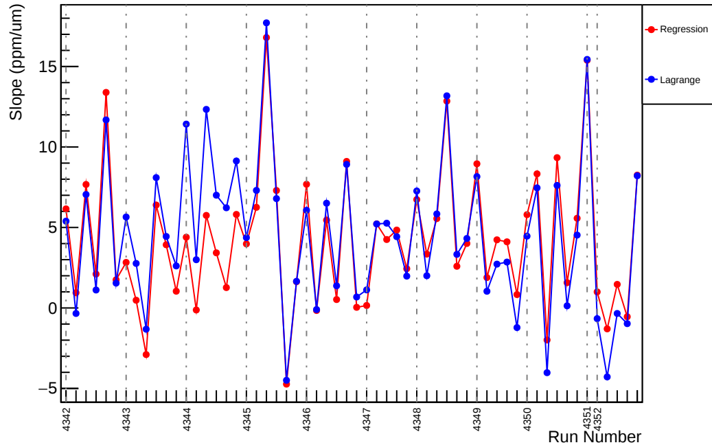
Slug57: Slope : usl_vs_evMon9 (ppm/um)
