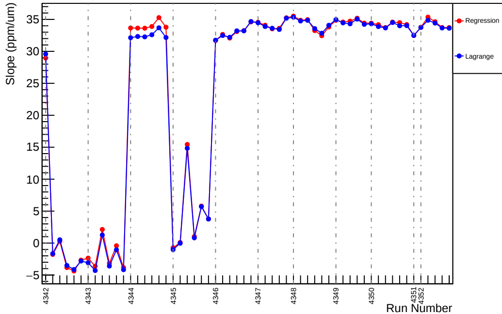
Slug57: Slope : usr_vs_evMon0 (ppm/um)
