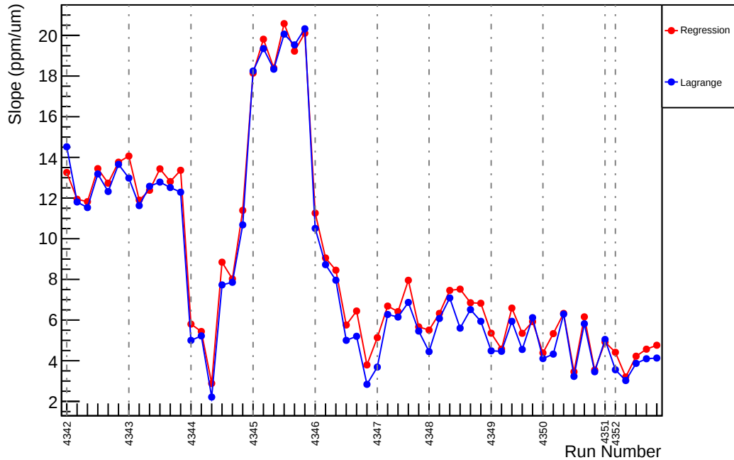
Slug57: Slope : usr_vs_evMon4 (ppm/um)
