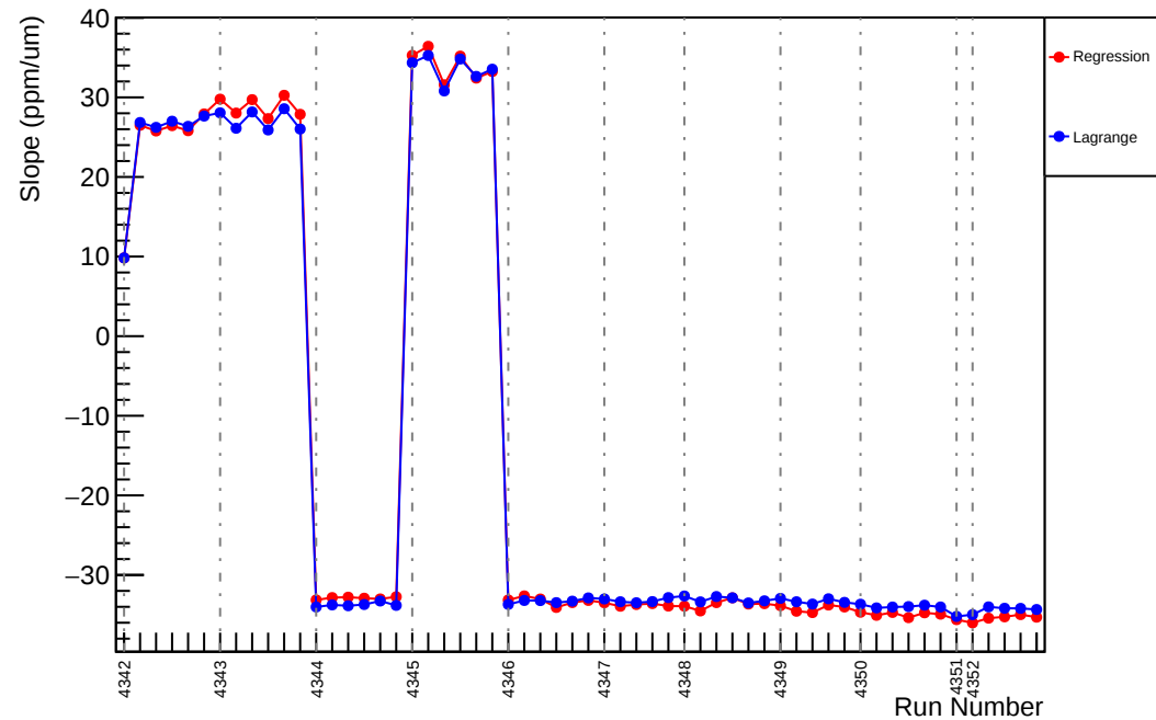
Slug57: Slope : usr_vs_evMon1 (ppm/um)
