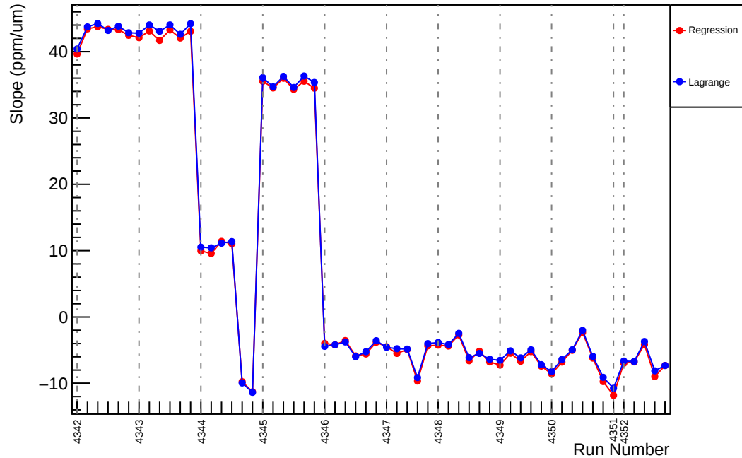
Slug57: Slope : usr_vs_evMon2 (ppm/um)
