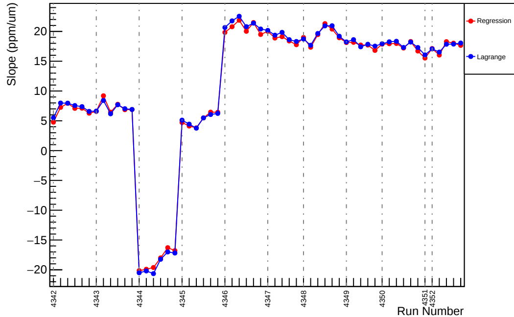
Slug57: Slope : usr_vs_evMon3 (ppm/um)
