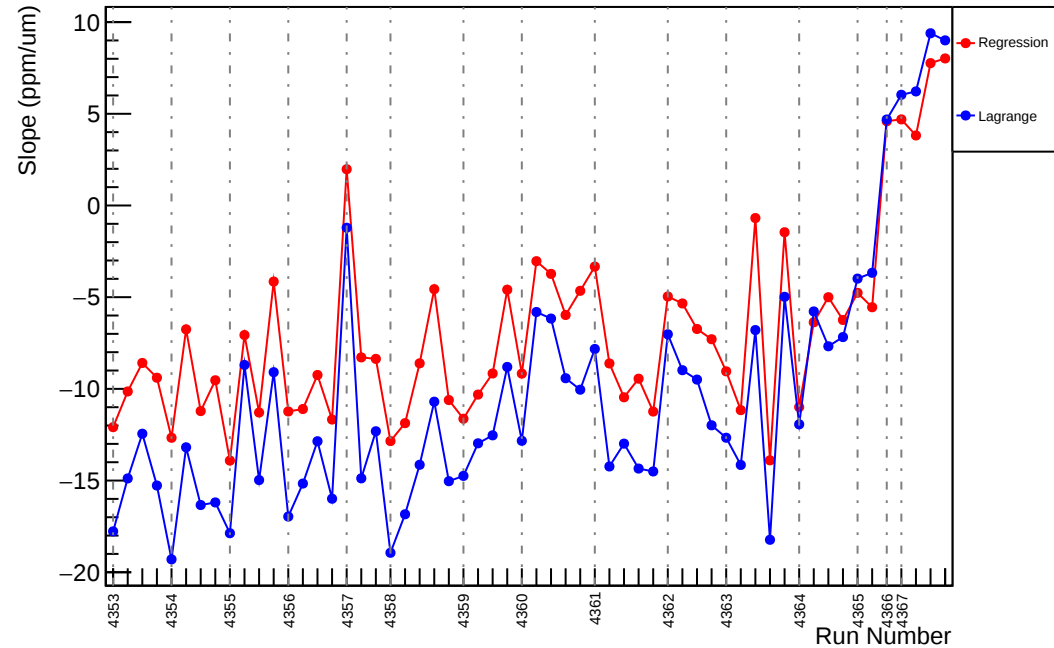
Slug58: Slope : us_avg_vs_evMon5 (ppm/um)
