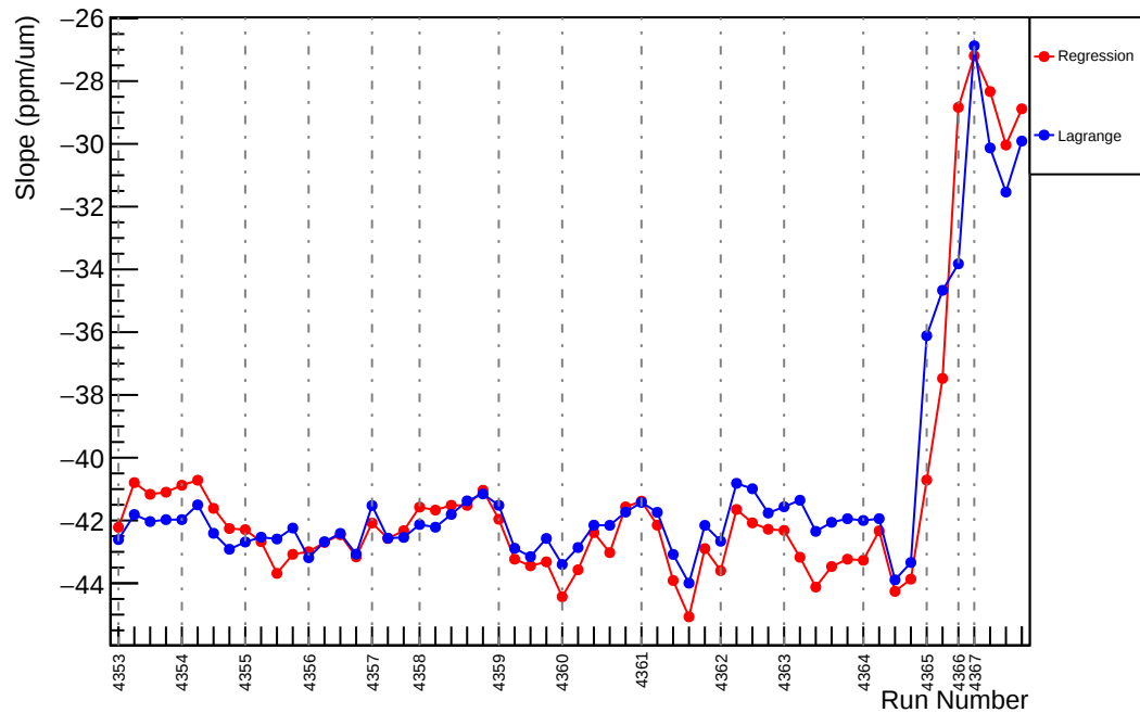
Slug58: Slope : us_avg_vs_evMon1 (ppm/um)
