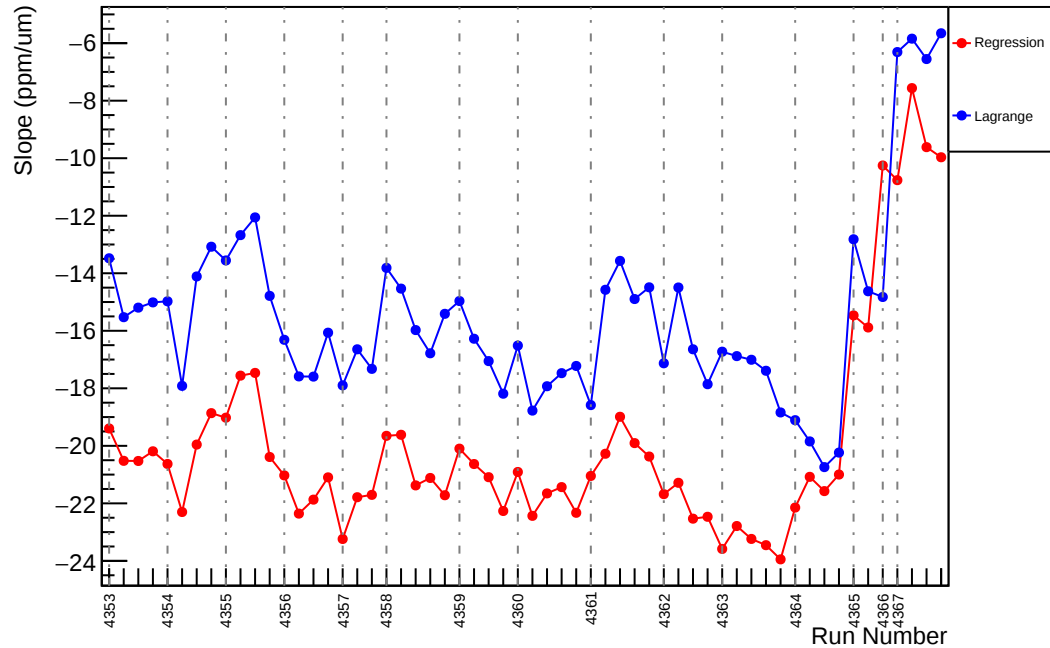
Slug58: Slope : us_avg_vs_evMon3 (ppm/um)
