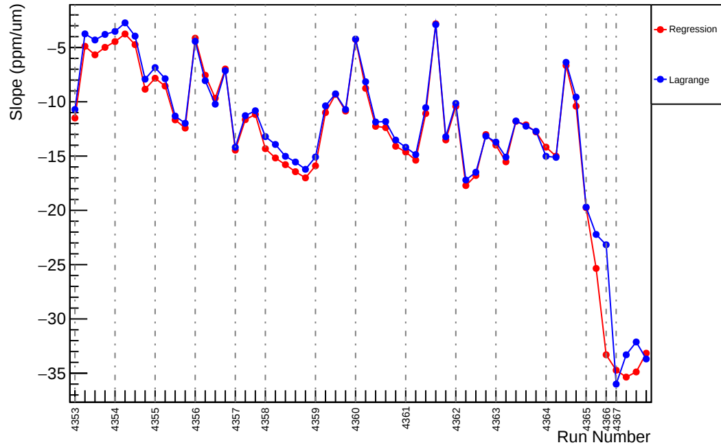
Slug58: Slope : us_avg_vs_evMon0 (ppm/um)
