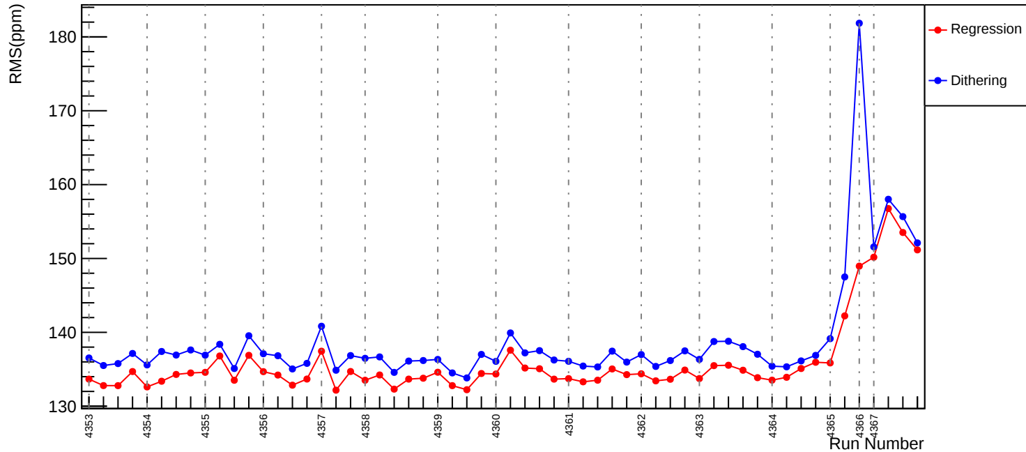
Slug58: Corrected RMS (ppm): asym_usl
