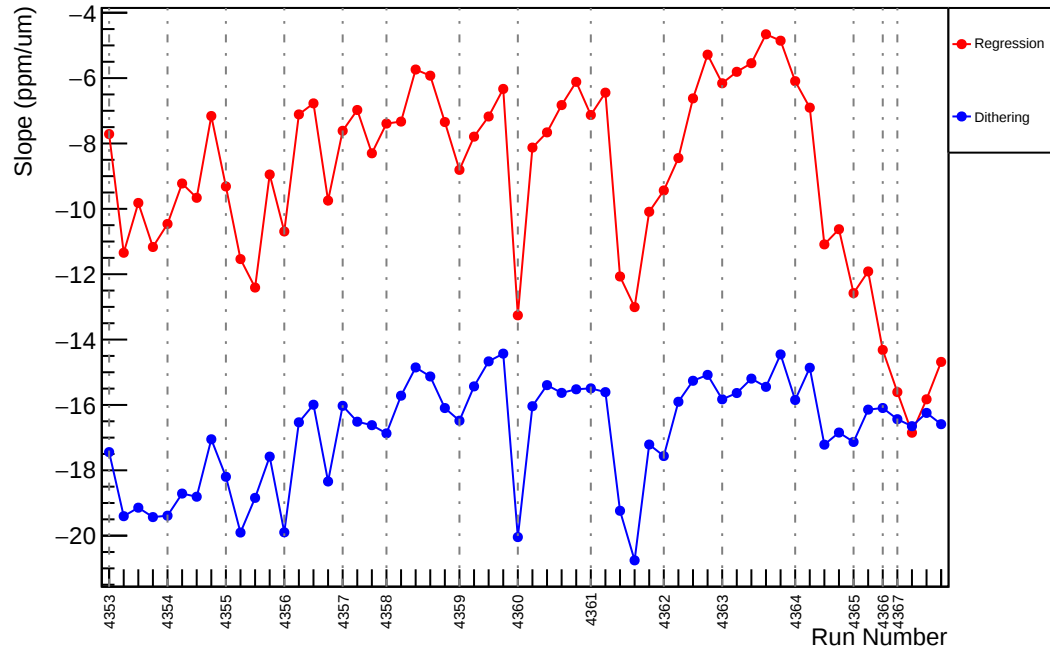
Slug58: Slope : usl_vs_evMon2 (ppm/um)
