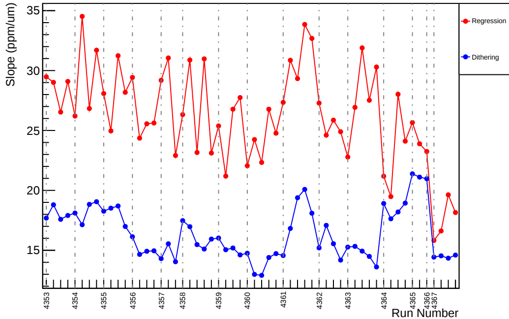
Slug58: Slope : usl_vs_evMon4 (ppm/um)
