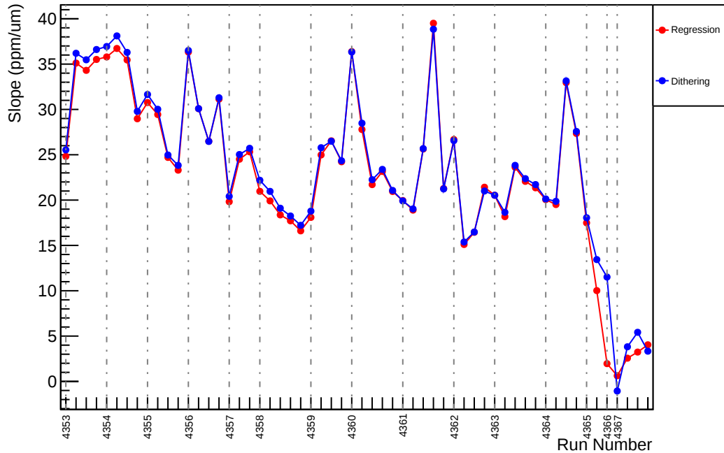
Slug58: Slope : usl_vs_evMon0 (ppm/um)
