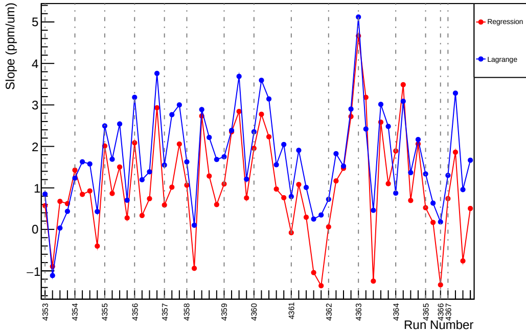
Slug58: Slope : usl_vs_evMon5 (ppm/um)
