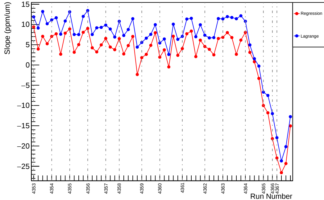
Slug58: Slope : usl_vs_evMon7 (ppm/um)
