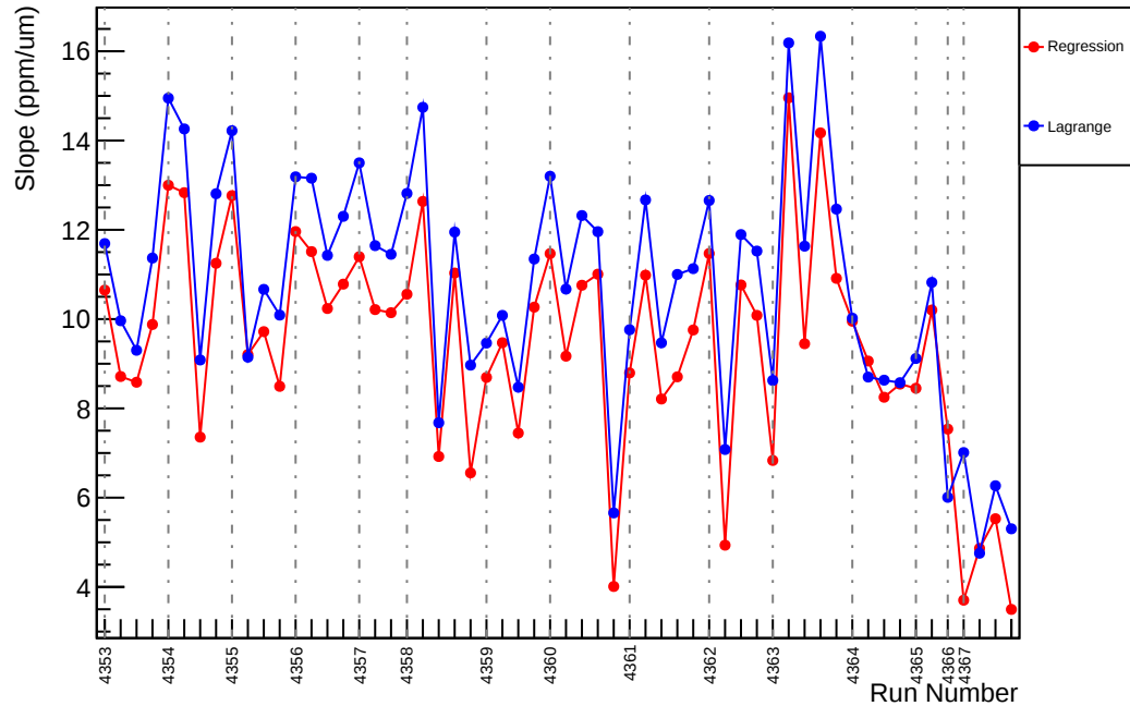
Slug58: Slope : usl_vs_evMon6 (ppm/um)
