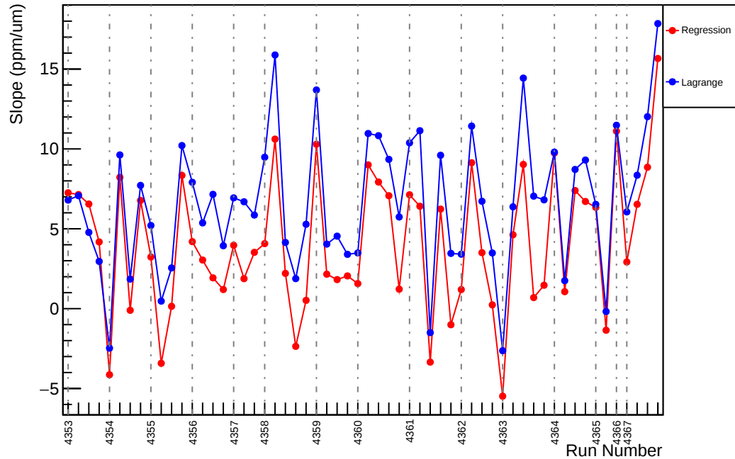
Slug58: Slope : usl_vs_evMon9 (ppm/um)
