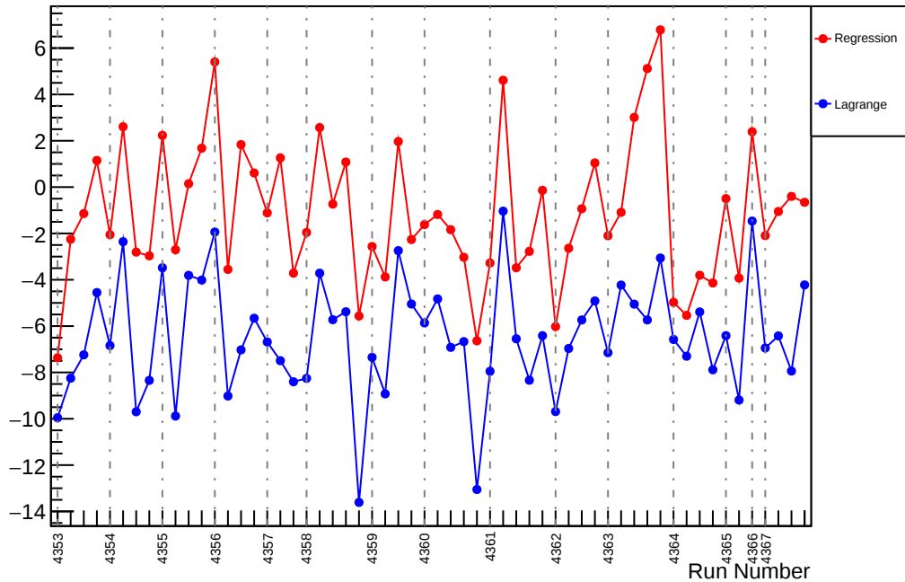
Slug58: Slope : usl_vs_evMon8 (ppm/um)
