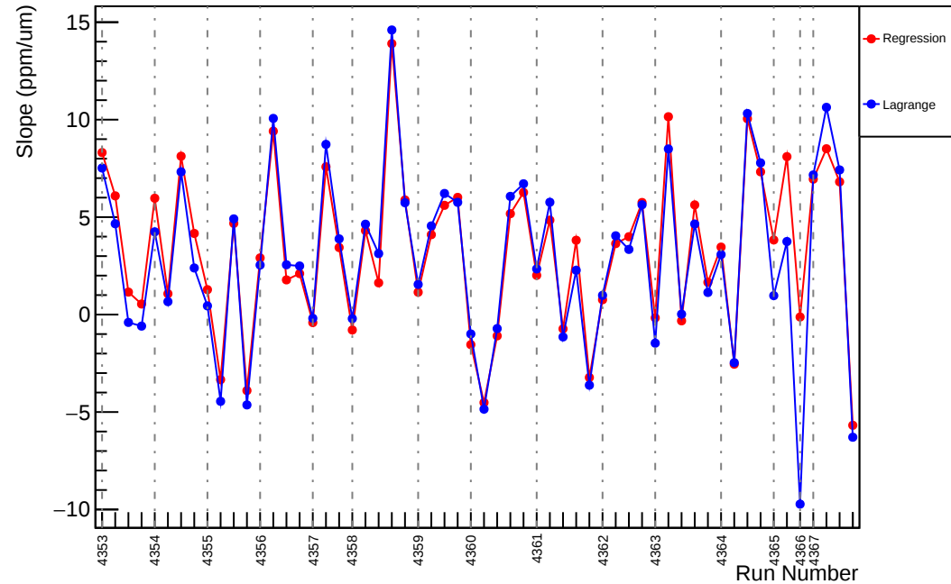
Slug58: Slope : usl_vs_evMon10 (ppm/um)
