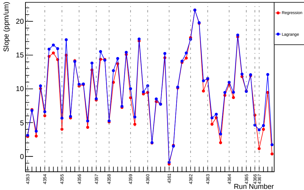
Slug58: Slope : usl_vs_evMon11 (ppm/um)
