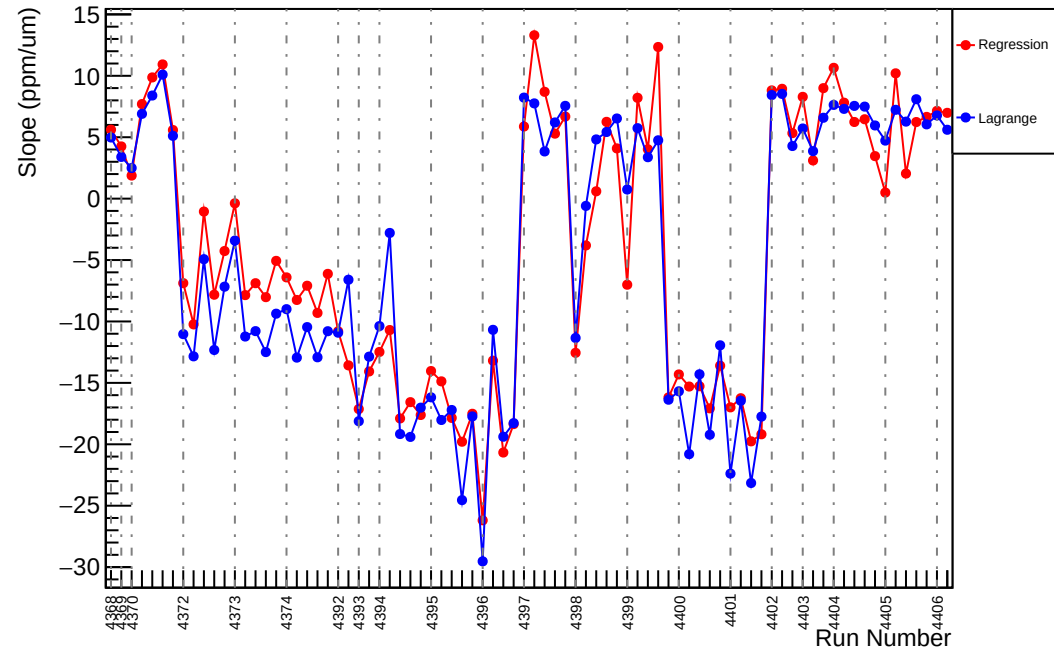
Slug59: Slope : us_avg_vs_evMon5 (ppm/um)
