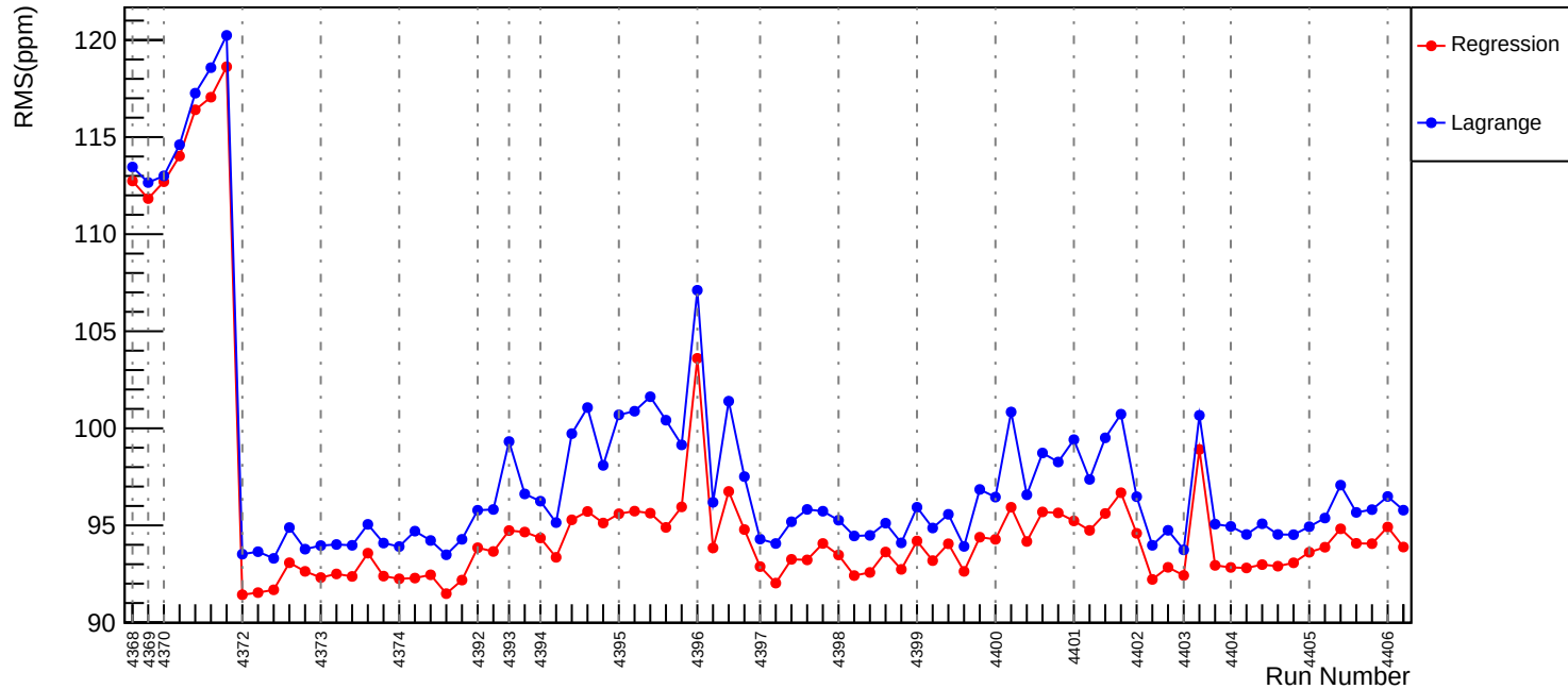
Slug59: Corrected RMS (ppm): asym_us_avg
