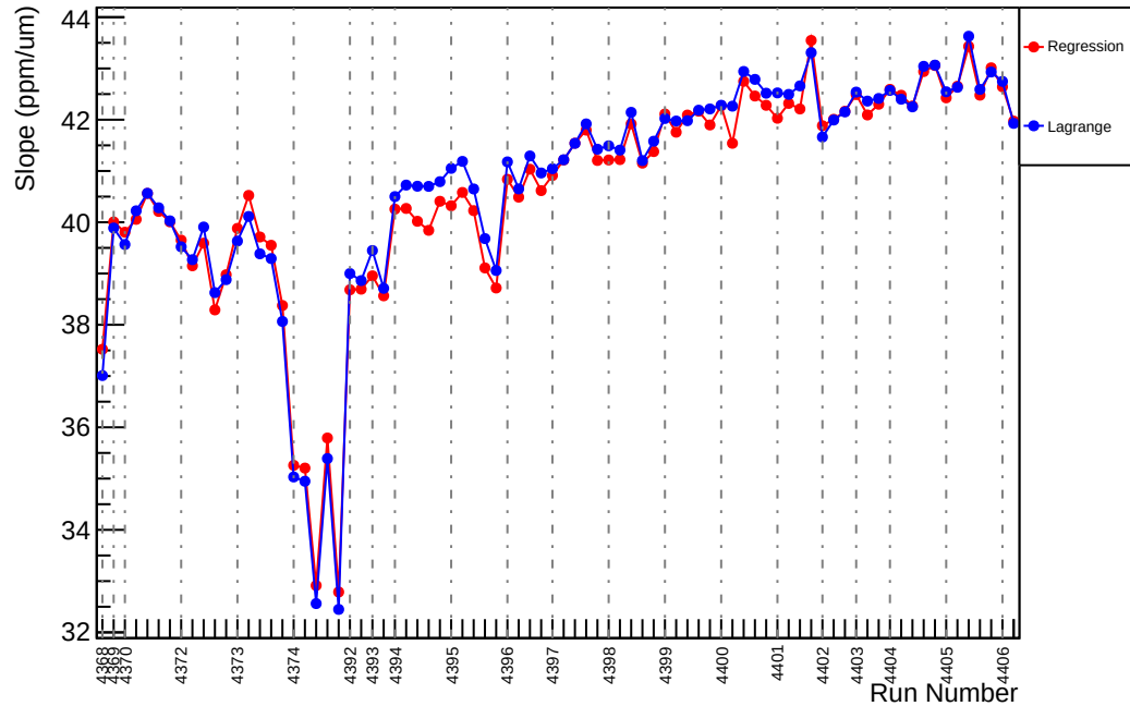
Slug59: Slope : us_dd_vs_evMon0 (ppm/um)
