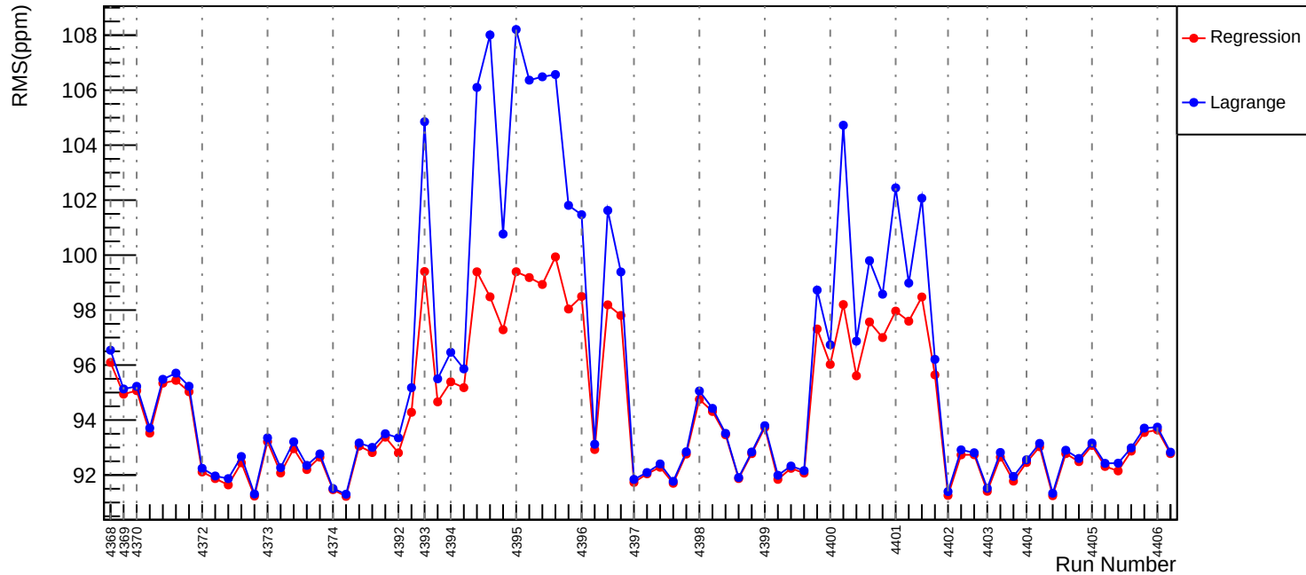
Slug59: Corrected RMS (ppm): asym_us_dd
