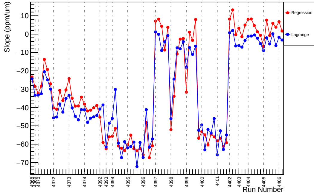
Slug59: Slope : usl_vs_evMon5 (ppm/um)
