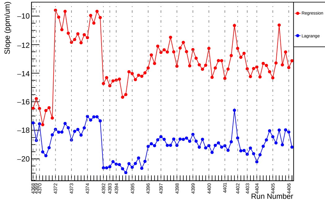
Slug59: Slope : usr_vs_evMon2 (ppm/um)
