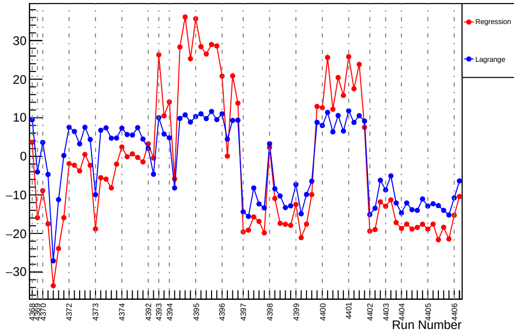
Slug59: Slope : usr_vs_evMon4 (ppm/um)
