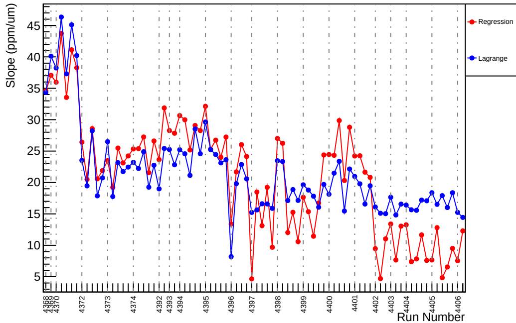
Slug59: Slope : usr_vs_evMon5 (ppm/um)
