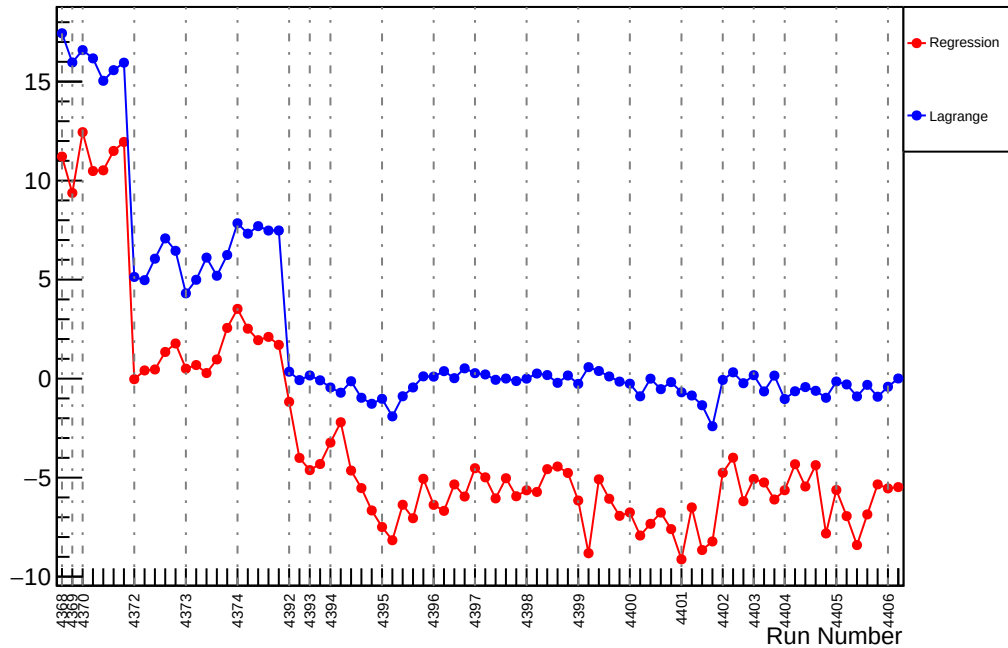
Slug59: Slope : usr_vs_evMon3 (ppm/um)
