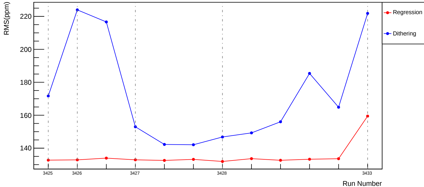
Slug5: Corrected RMS (ppm): asym_usl
