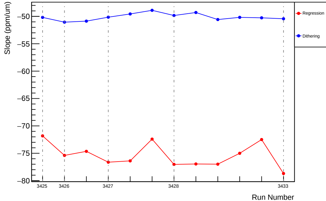
Slug5: Slope : usl_vs_evMon4 (ppm/um)
