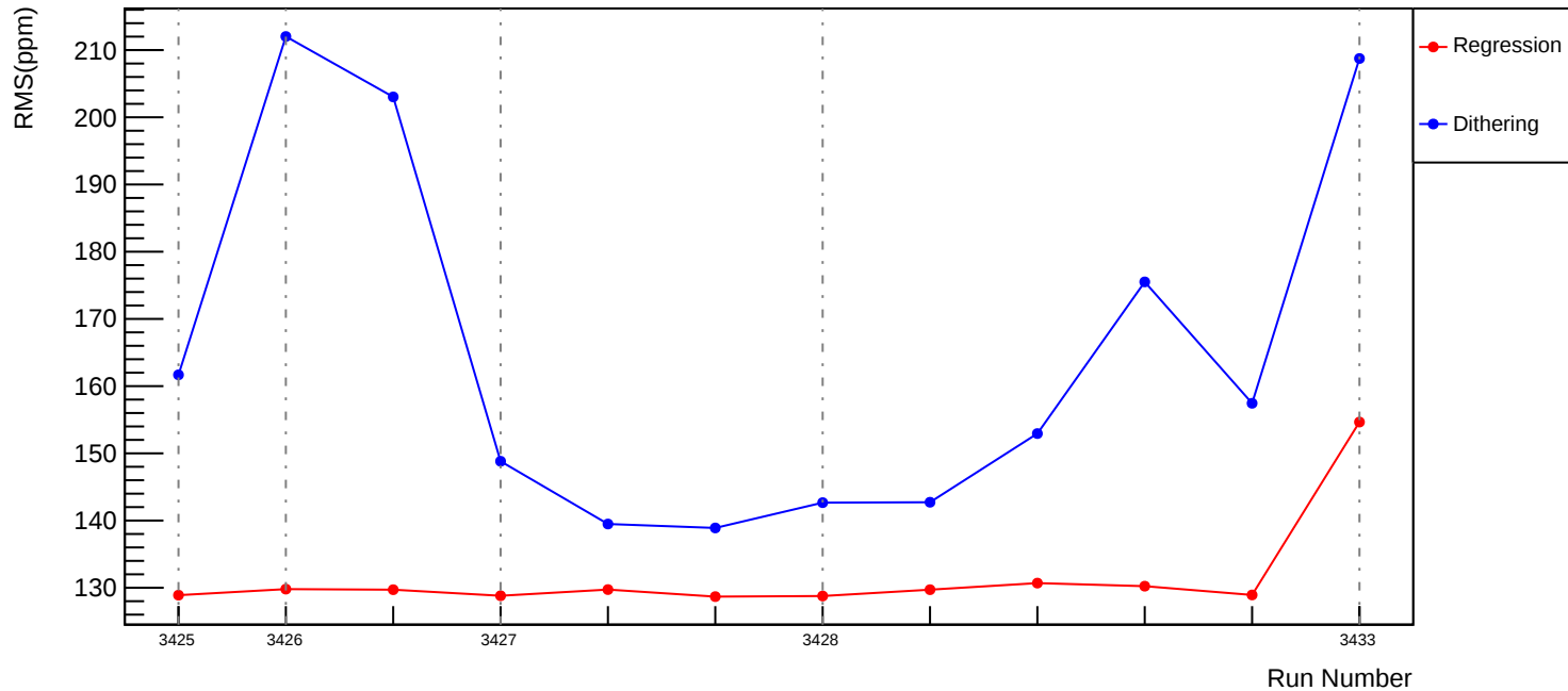
Slug5: Corrected RMS (ppm): asym_usr
