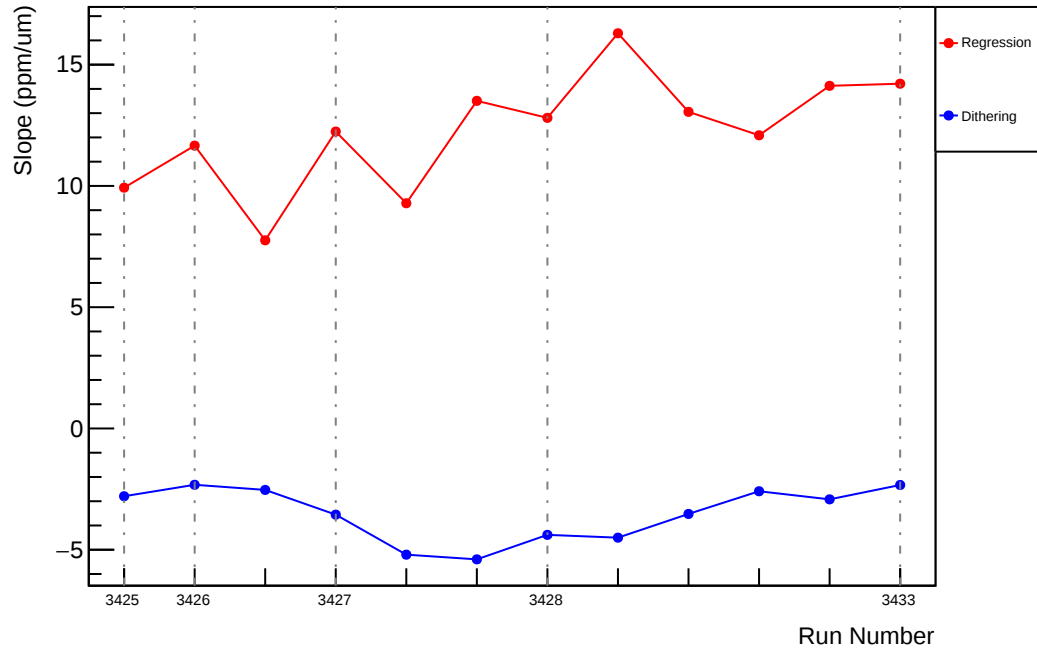
Slug5: Slope : usr_vs_evMon4 (ppm/um)
