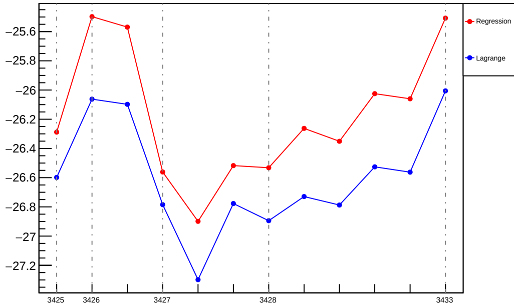
Slug5: Slope : usr_vs_evMon0 (ppm/um)
