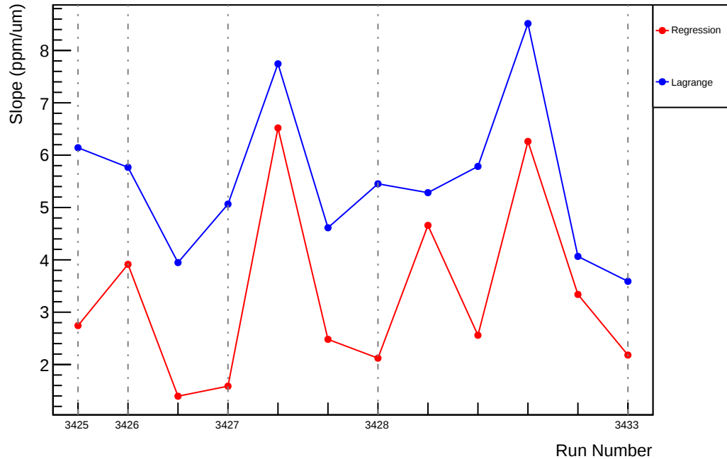
Slug5: Slope : usr_vs_evMon7 (ppm/um)
