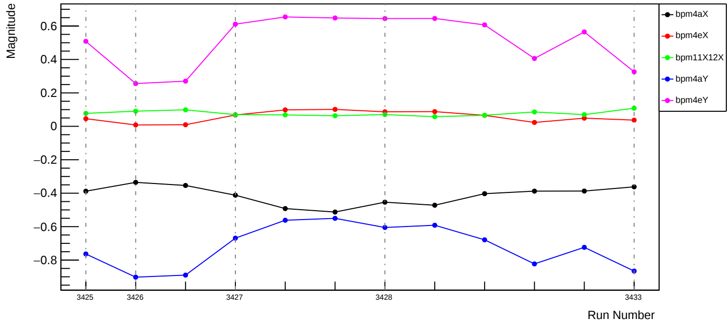
Slug5: EigenVector #3
