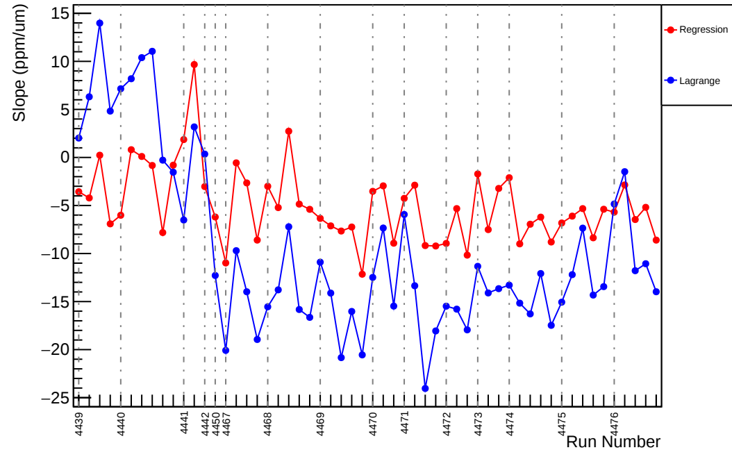
Slug60: Slope : us_avg_vs_evMon9 (ppm/um)
