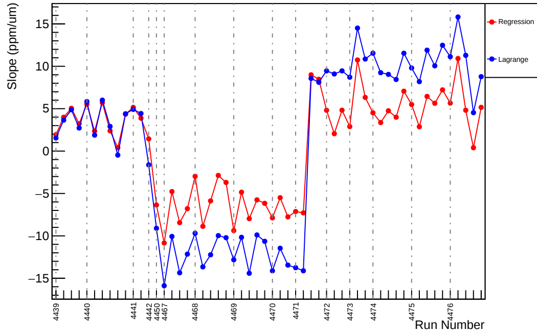
Slug60: Slope : us_avg_vs_evMon7 (ppm/um)
