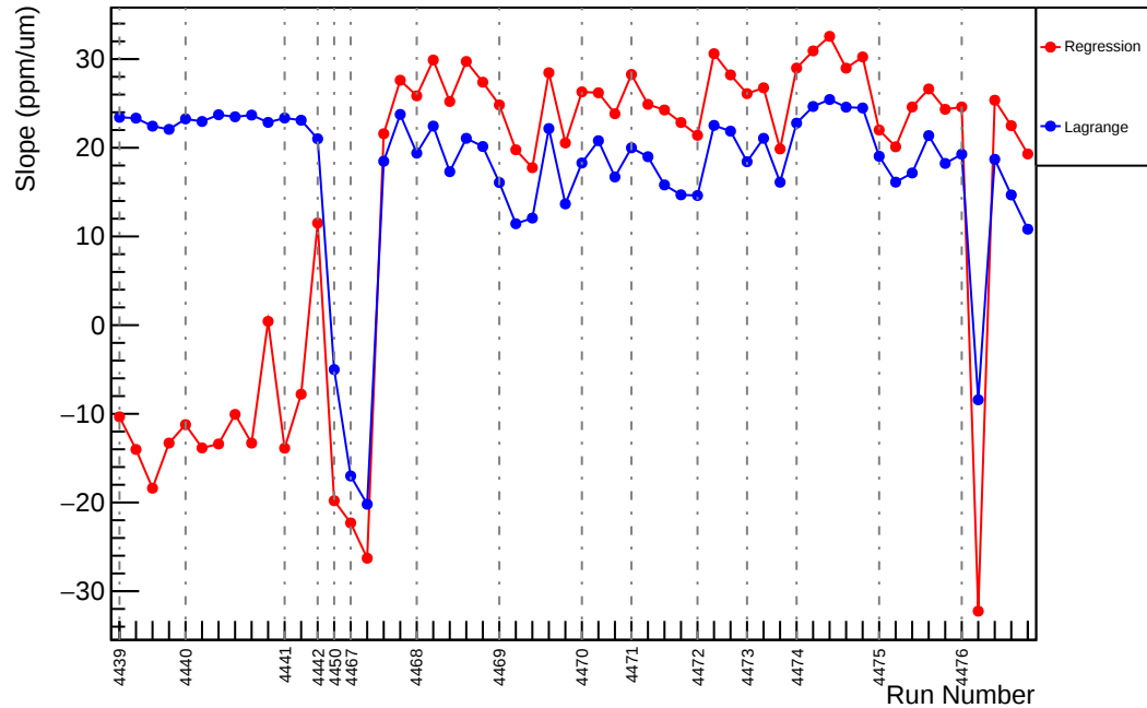
Slug60: Slope : usr_vs_evMon4 (ppm/um)
