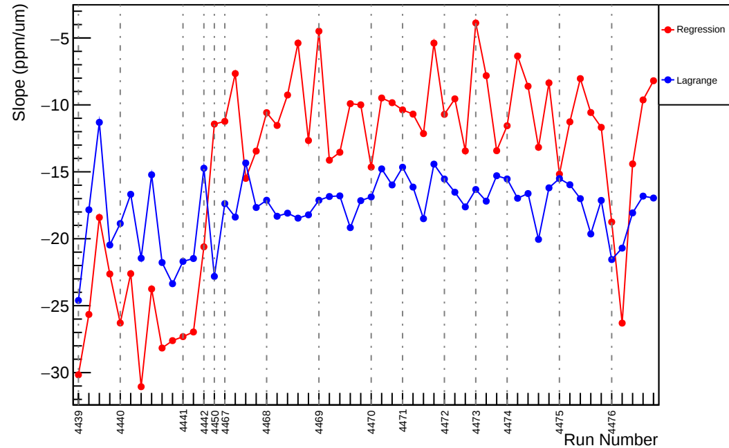
Slug60: Slope : usr_vs_evMon5 (ppm/um)
