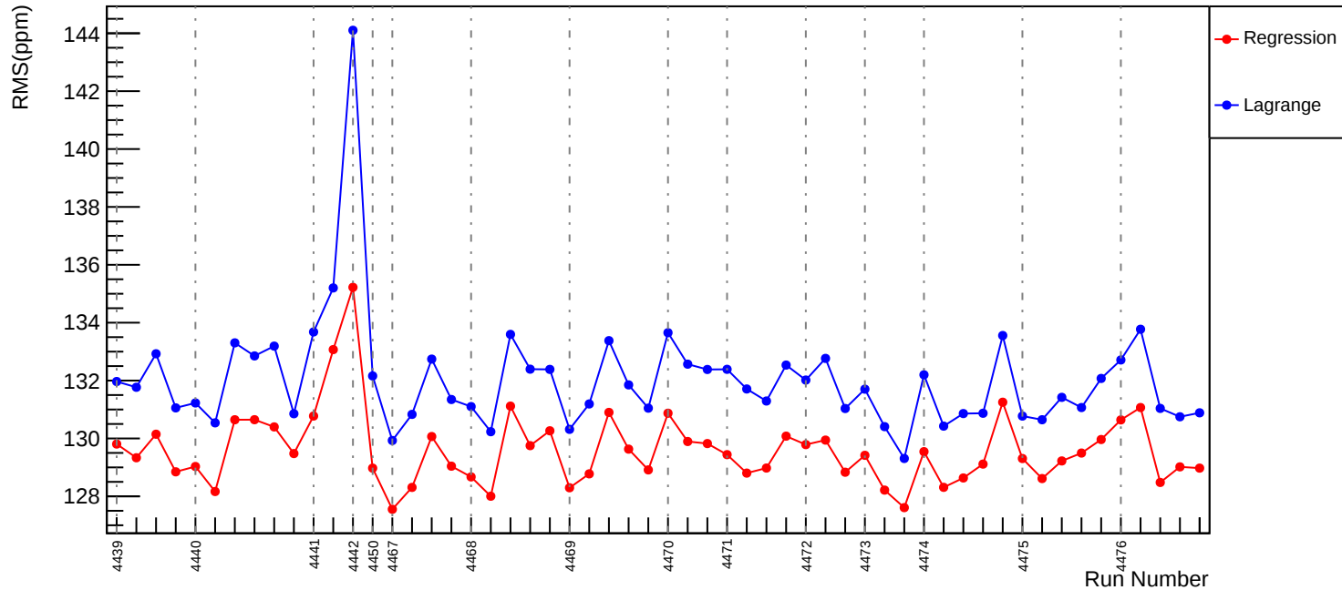
Slug60: Corrected RMS (ppm): asym_usr
