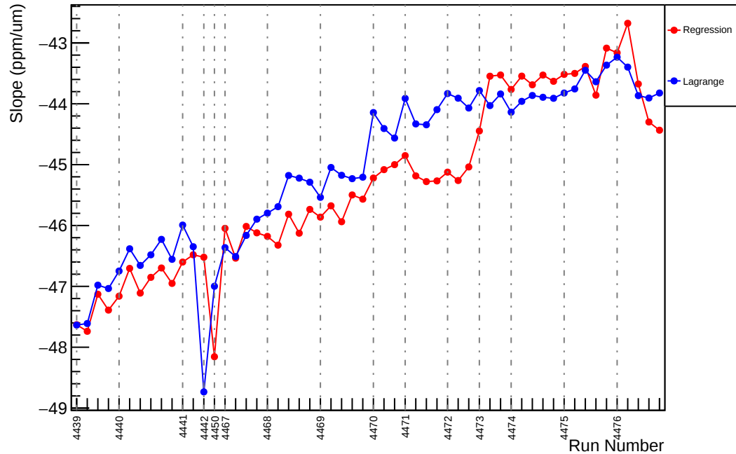
Slug60: Slope : usr_vs_evMon0 (ppm/um)
