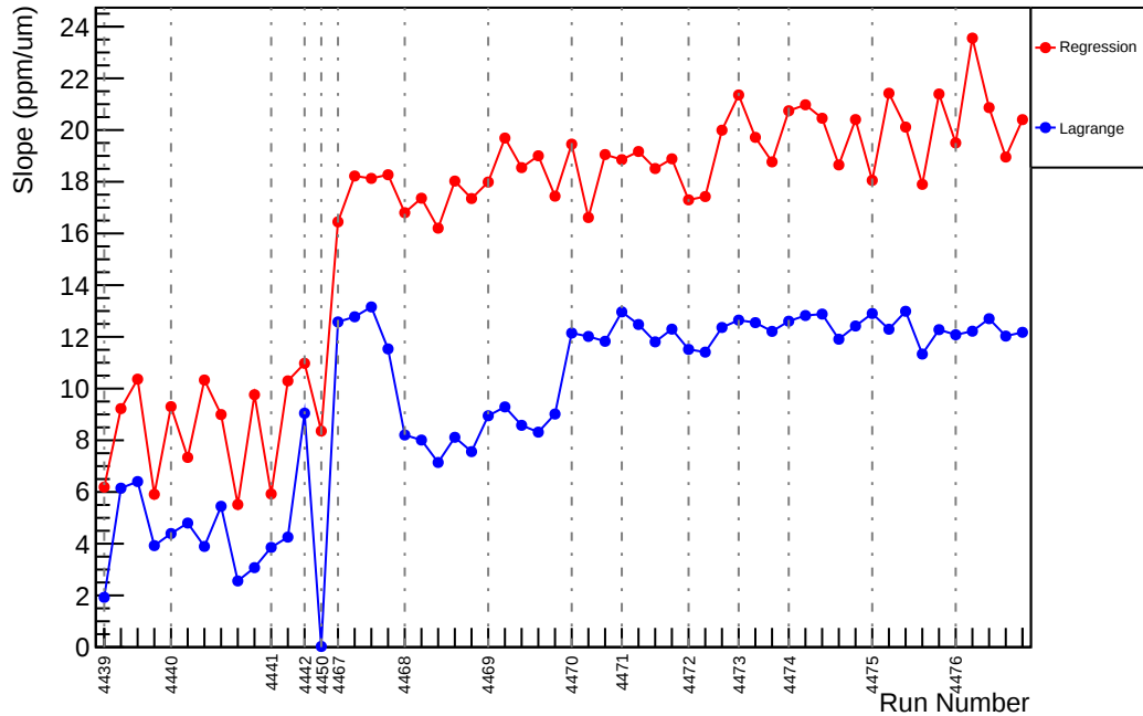
Slug60: Slope : usr_vs_evMon3 (ppm/um)
