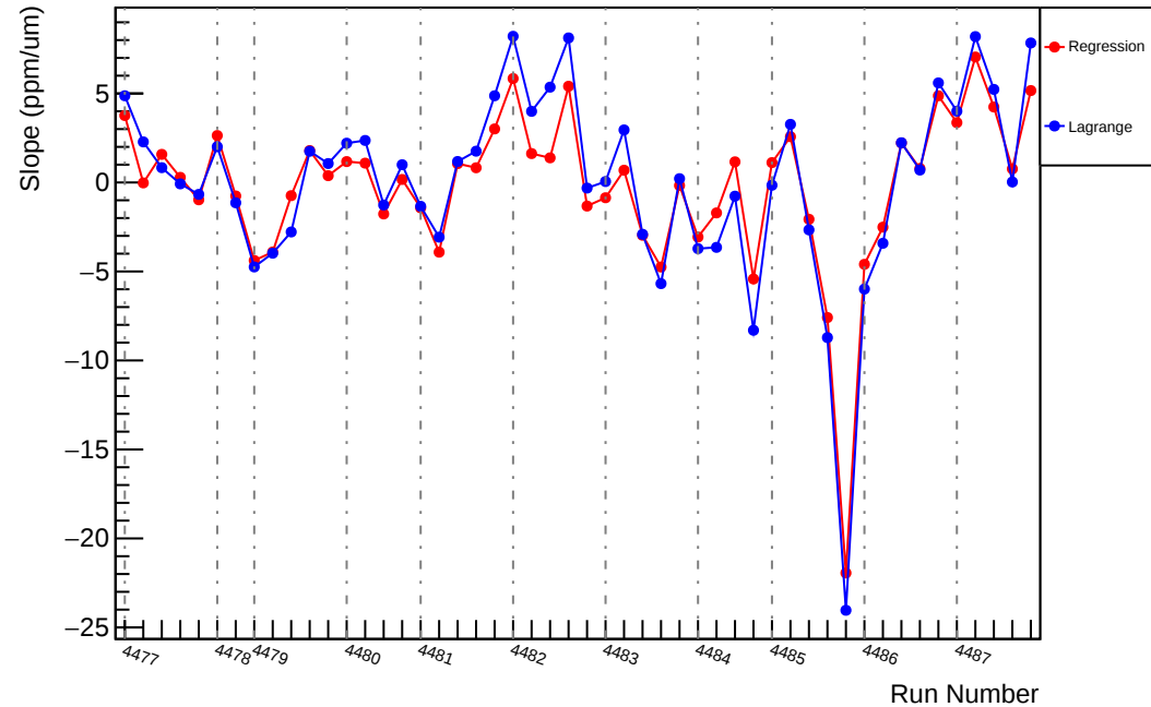
Slug61: Slope : usl_vs_evMon6 (ppm/um)
