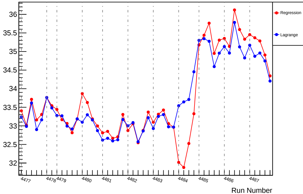
Slug61: Slope : usl_vs_evMon0 (ppm/um)
