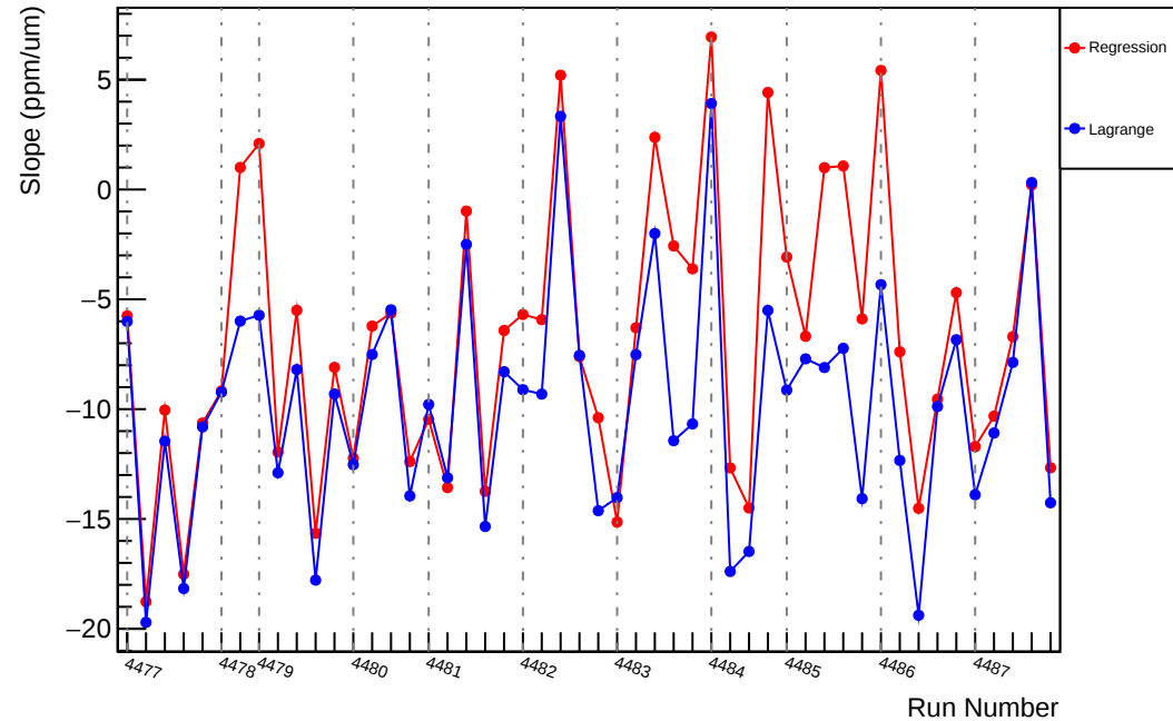
Slug61: Slope : usl_vs_evMon10 (ppm/um)
