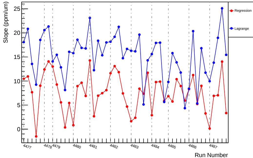
Slug61: Slope : usl_vs_evMon9 (ppm/um)
