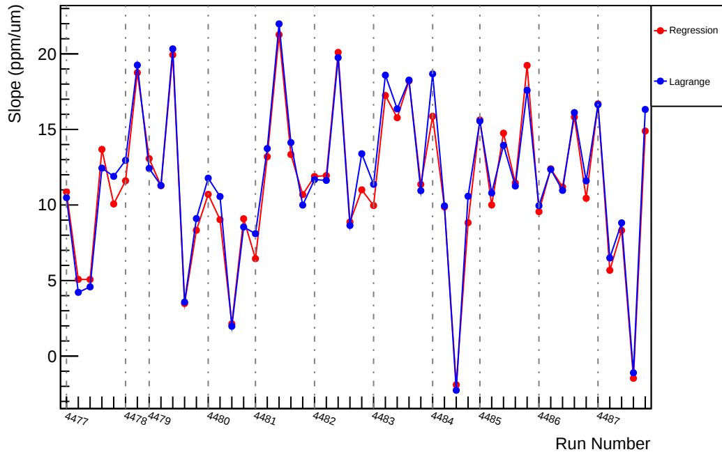
Slug61: Slope : usl_vs_evMon11 (ppm/um)
