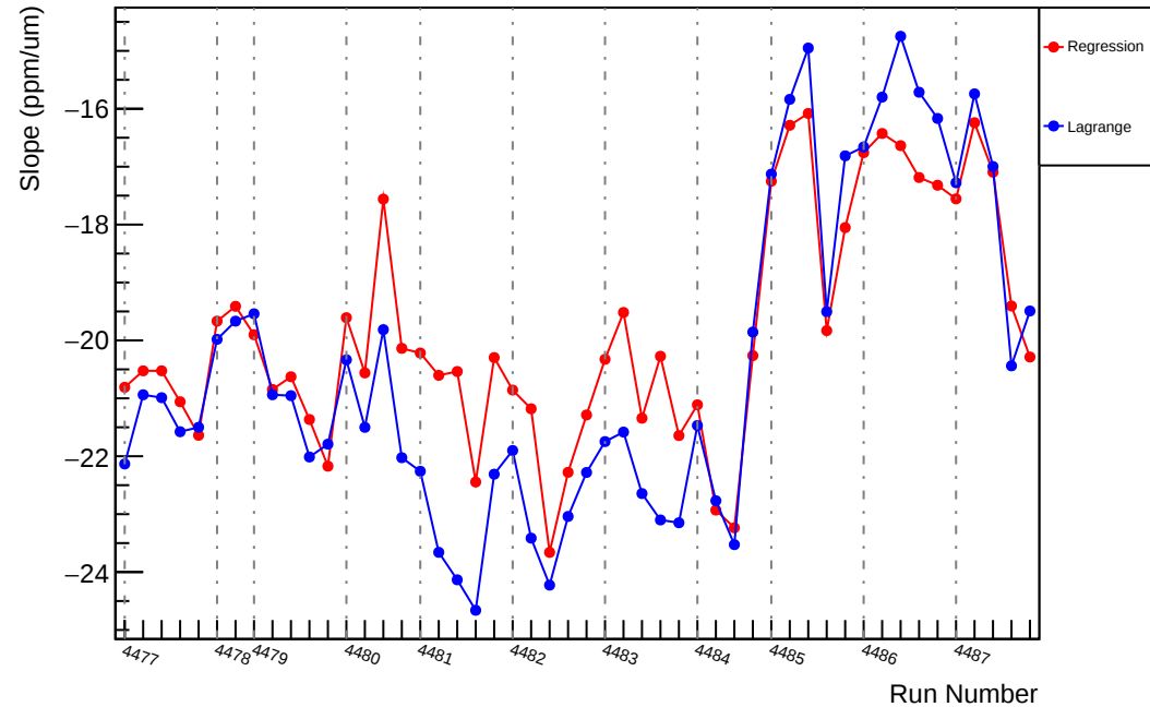
Slug61: Slope : usr_vs_evMon4 (ppm/um)
