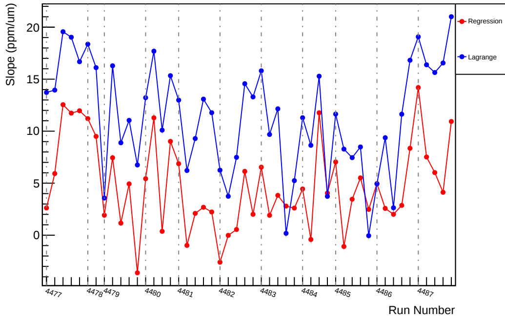
Slug61: Slope : usr_vs_evMon9 (ppm/um)
