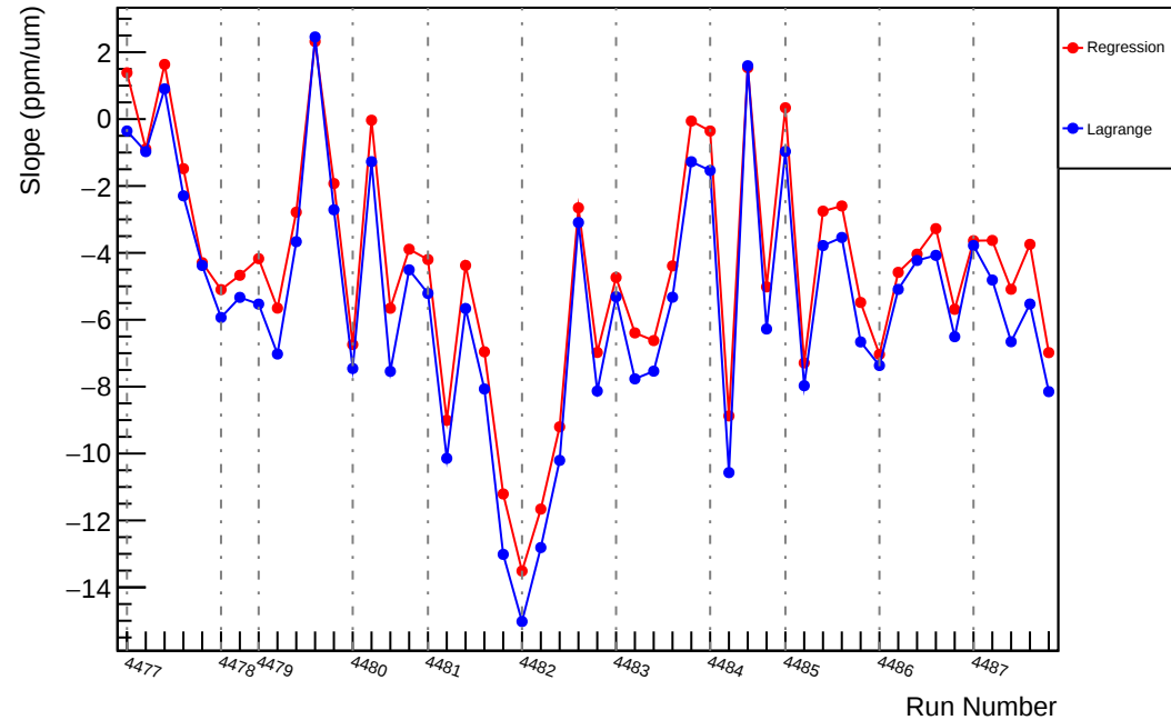
Slug61: Slope : usr_vs_evMon3 (ppm/um)
