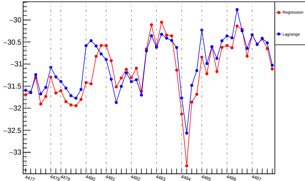
Slug61: Slope : usr_vs_evMon0 (ppm/um)
