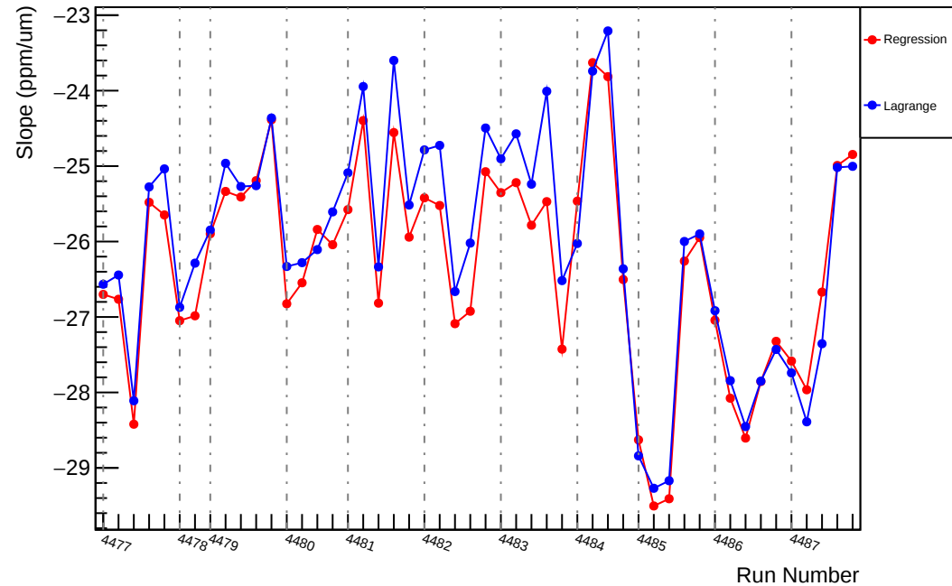
Slug61: Slope : usr_vs_evMon1 (ppm/um)
