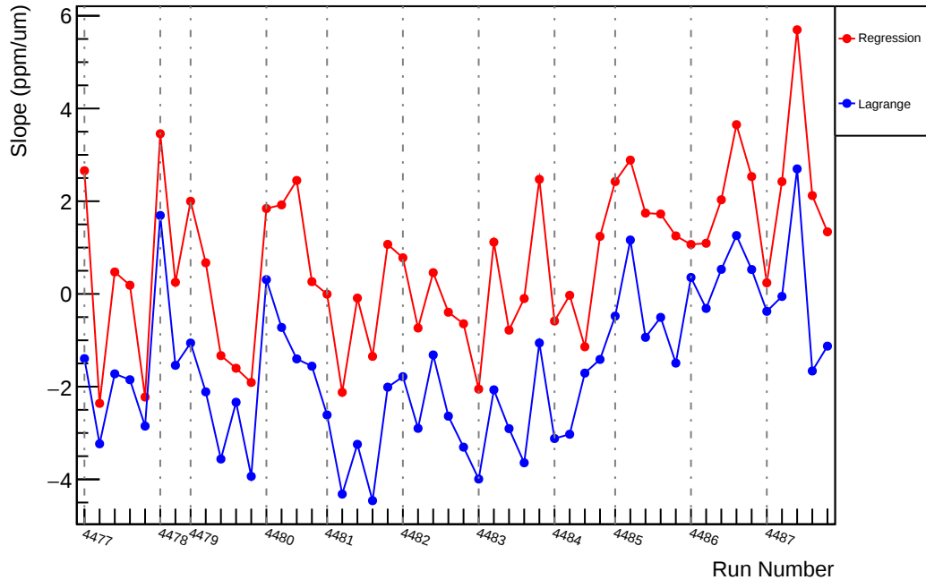
Slug61: Slope : usr_vs_evMon5 (ppm/um)
