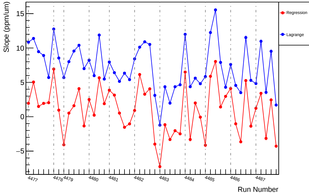
Slug61: Slope : usr_vs_evMon8 (ppm/um)
