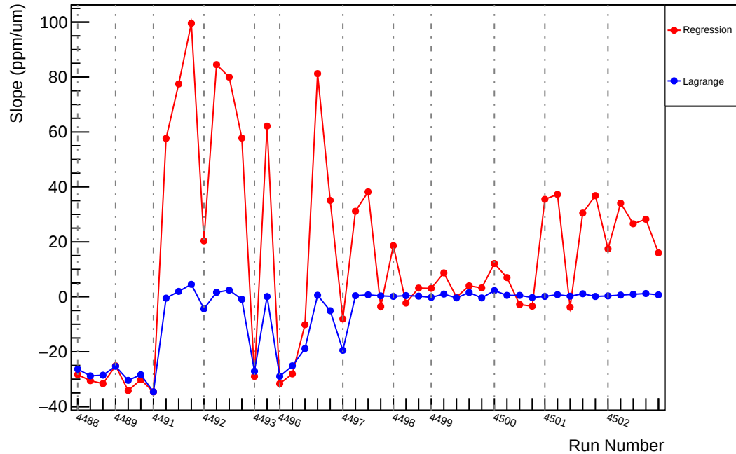
Slug62: Slope : us_dd_vs_evMon4 (ppm/um)
