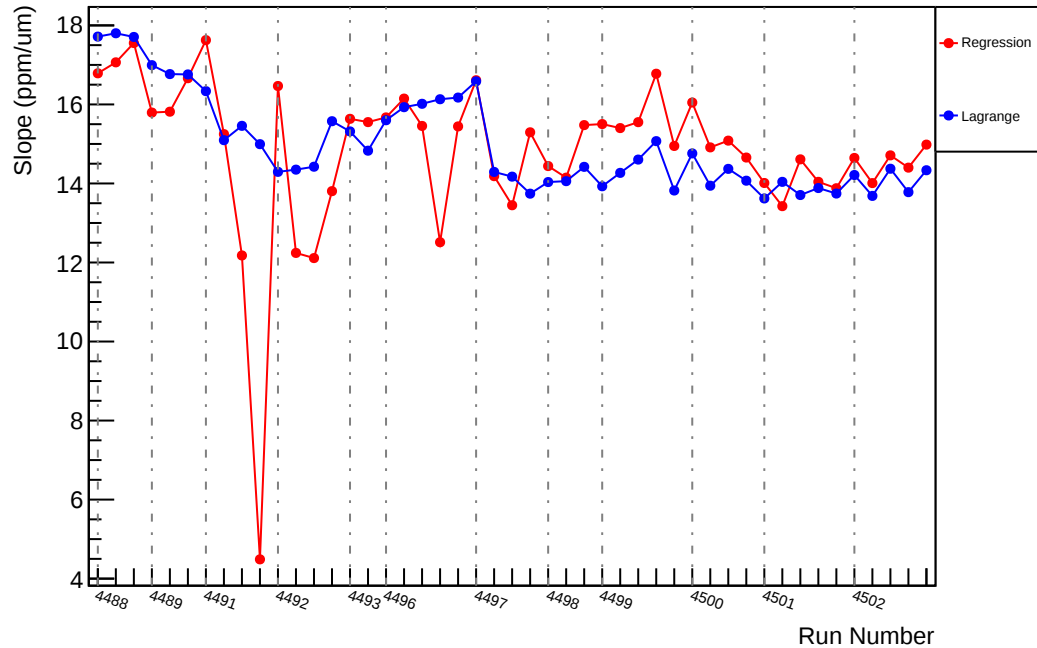
Slug62: Slope : us_dd_vs_evMon3 (ppm/um)
