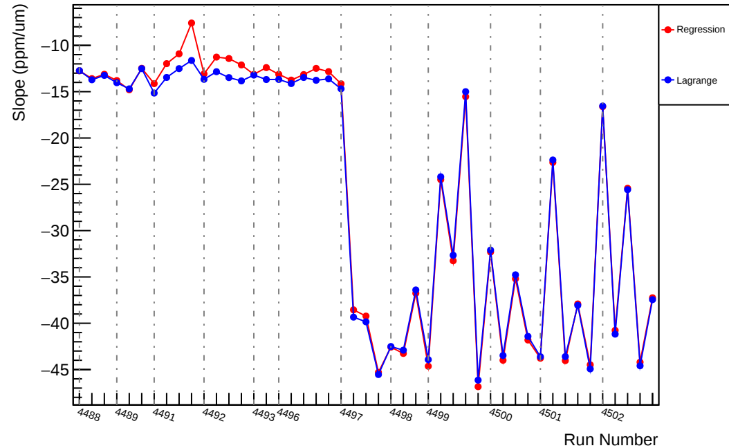
Slug62: Slope : us_dd_vs_evMon1 (ppm/um)
