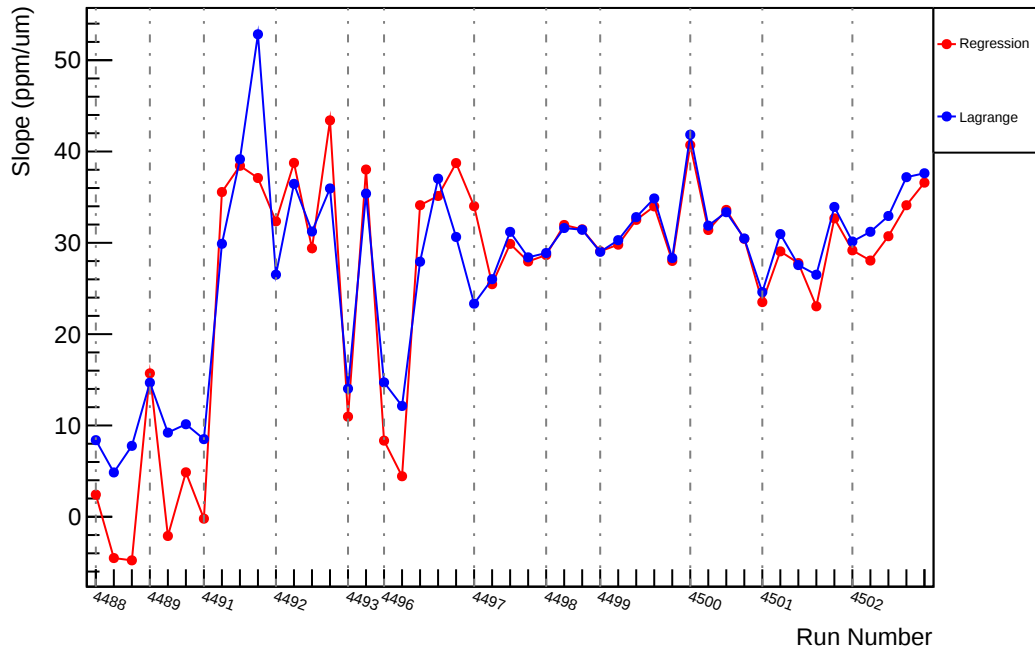
Slug62: Slope : us_dd_vs_evMon5 (ppm/um)
