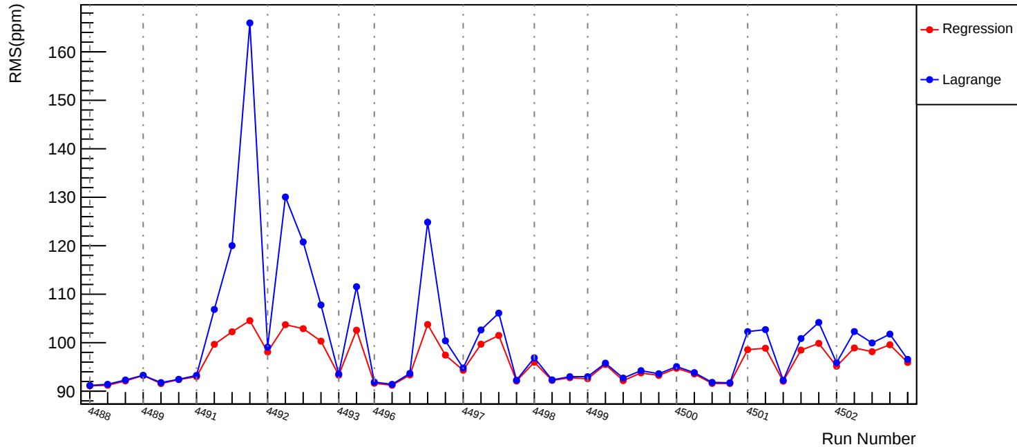
Slug62: Corrected RMS (ppm): asym_us_dd
