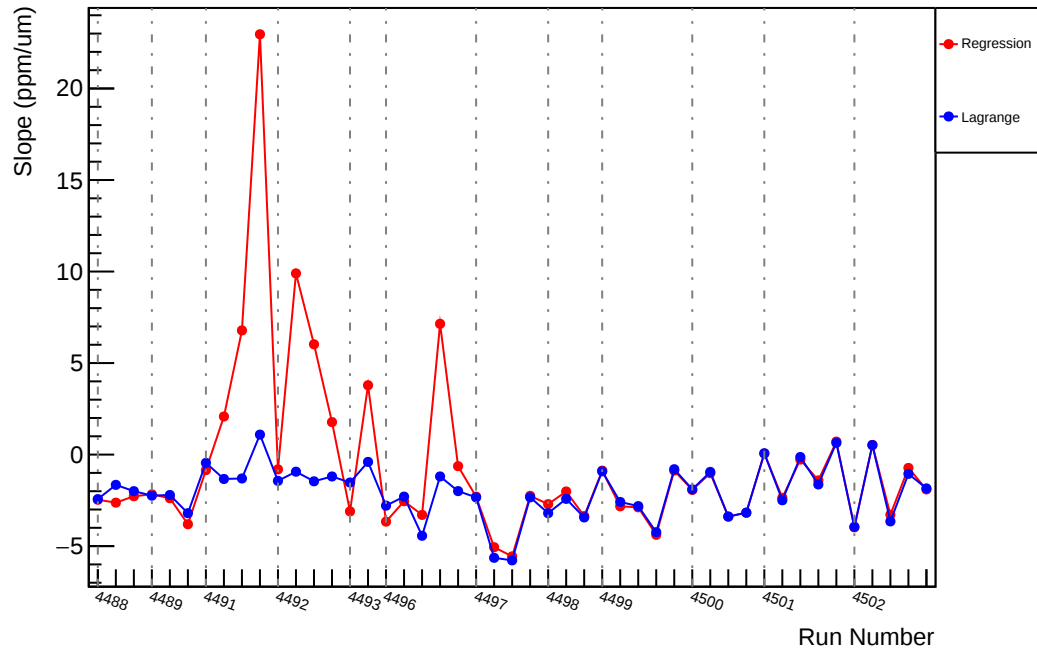
Slug62: Slope : us_dd_vs_evMon2 (ppm/um)
