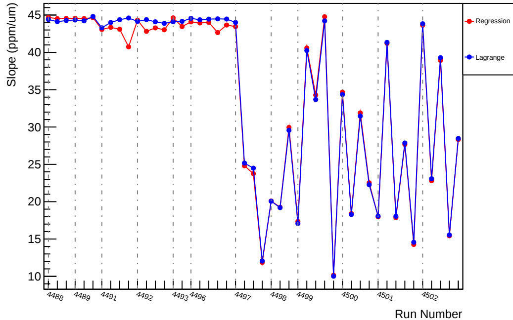
Slug62: Slope : us_dd_vs_evMon0 (ppm/um)
