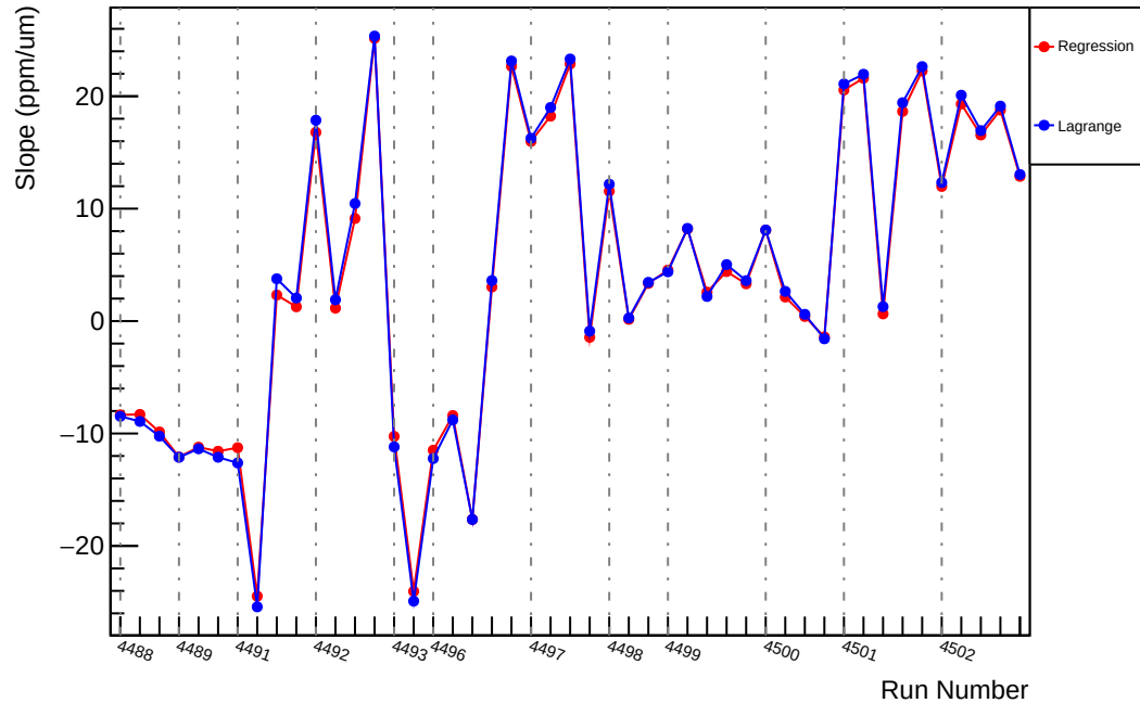
Slug62: Slope : us_dd_vs_evMon6 (ppm/um)
