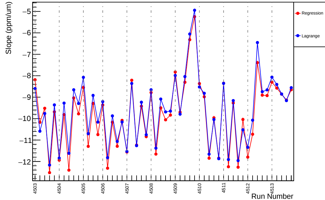
Slug63: Slope : us_avg_vs_evMon0 (ppm/um)
