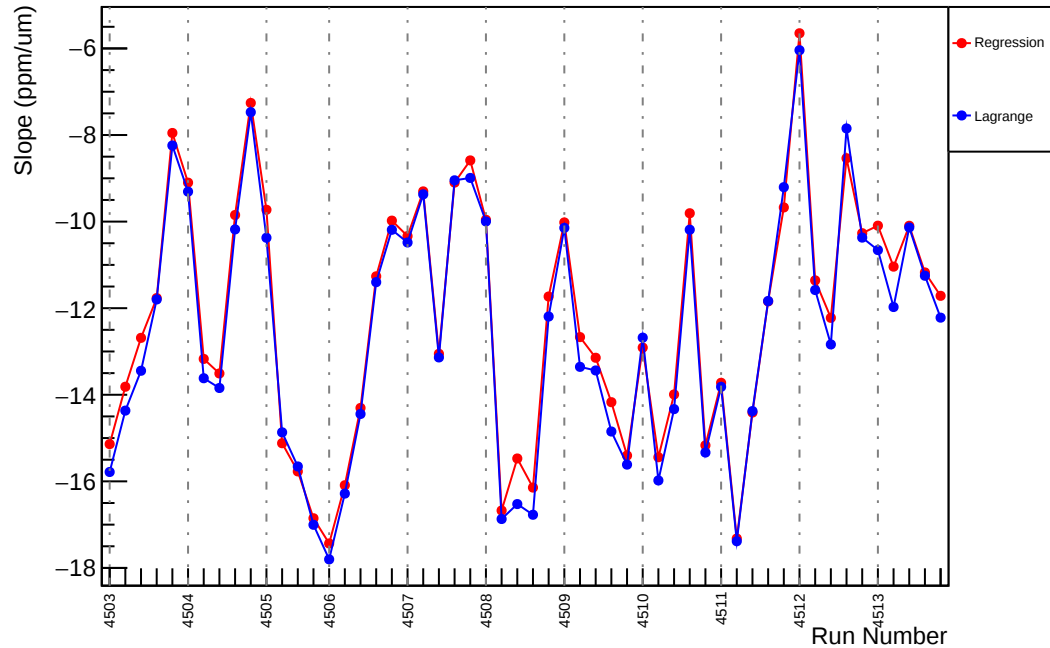
Slug63: Slope : us_avg_vs_evMon7 (ppm/um)
