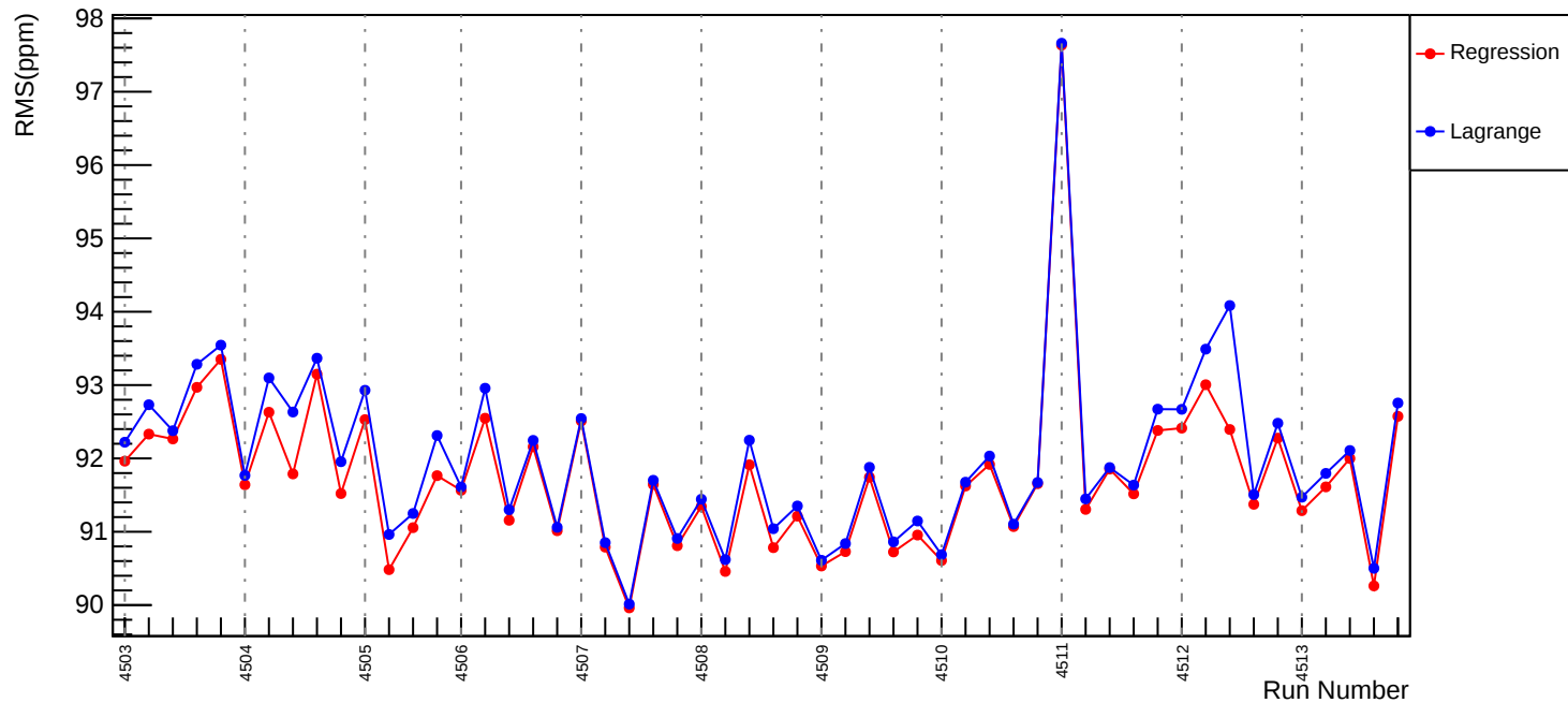
Slug63: Corrected RMS (ppm): asym_us_avg
