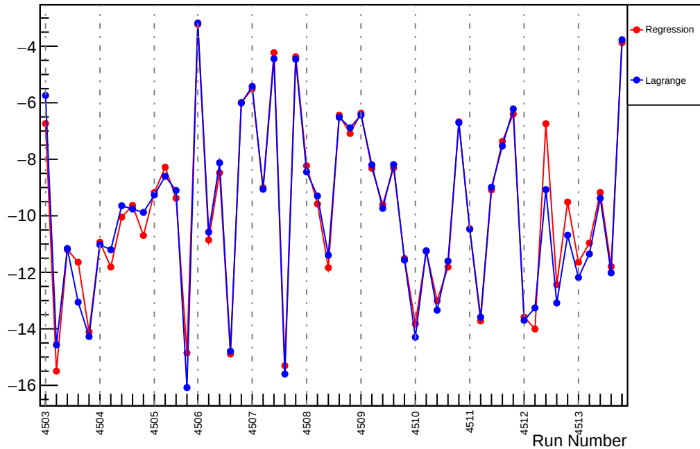
Slug63: Slope : us_avg_vs_evMon11 (ppm/um)
