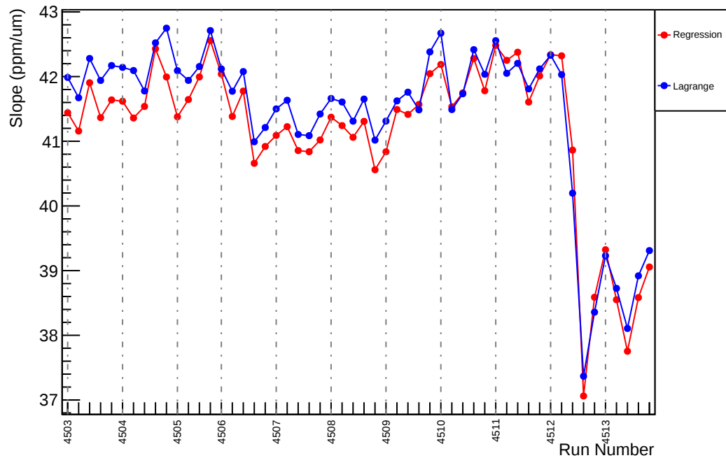
Slug63: Slope : us_avg_vs_evMon2 (ppm/um)
