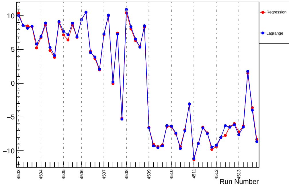
Slug63: Slope : us_avg_vs_evMon10 (ppm/um)
