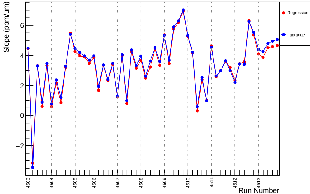
Slug63: Slope : us_avg_vs_evMon1 (ppm/um)
