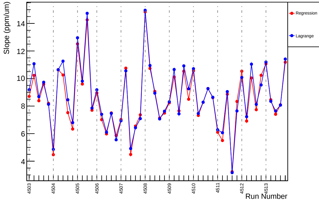
Slug63: Slope : us_avg_vs_evMon8 (ppm/um)
