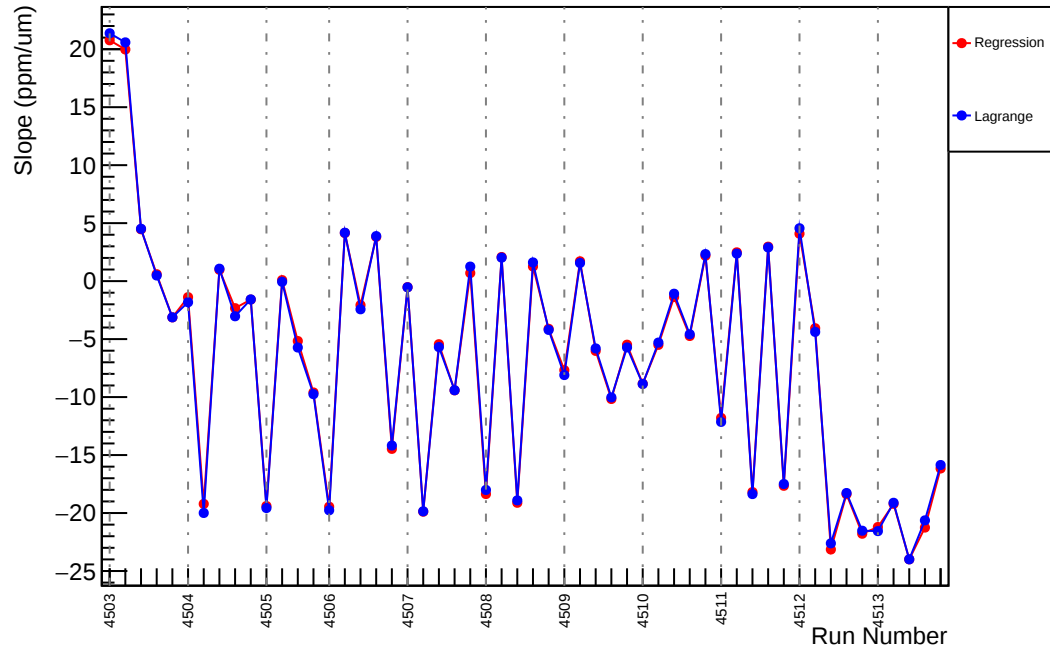
Slug63: Slope : us_avg_vs_evMon4 (ppm/um)
