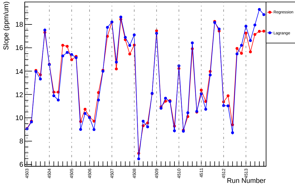
Slug63: Slope : us_avg_vs_evMon6 (ppm/um)
