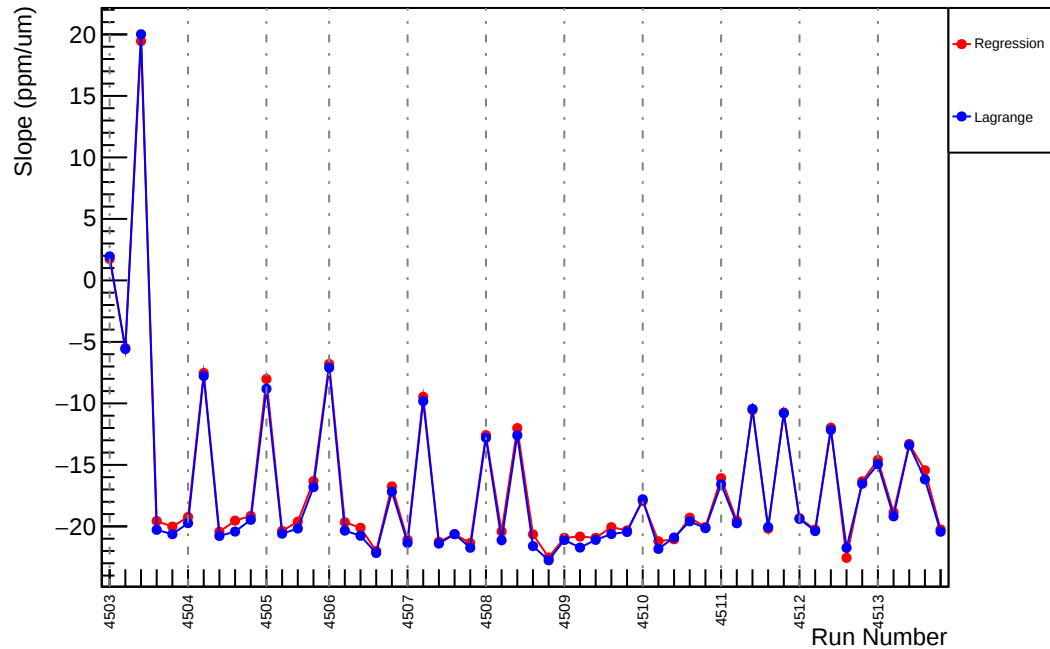
Slug63: Slope : us_avg_vs_evMon3 (ppm/um)
