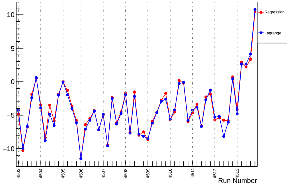
Slug63: Slope : us_avg_vs_evMon9 (ppm/um)
