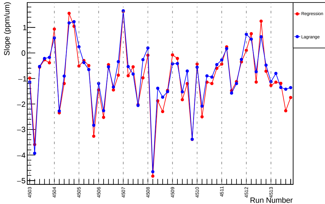
Slug63: Slope : us_avg_vs_evMon5 (ppm/um)
