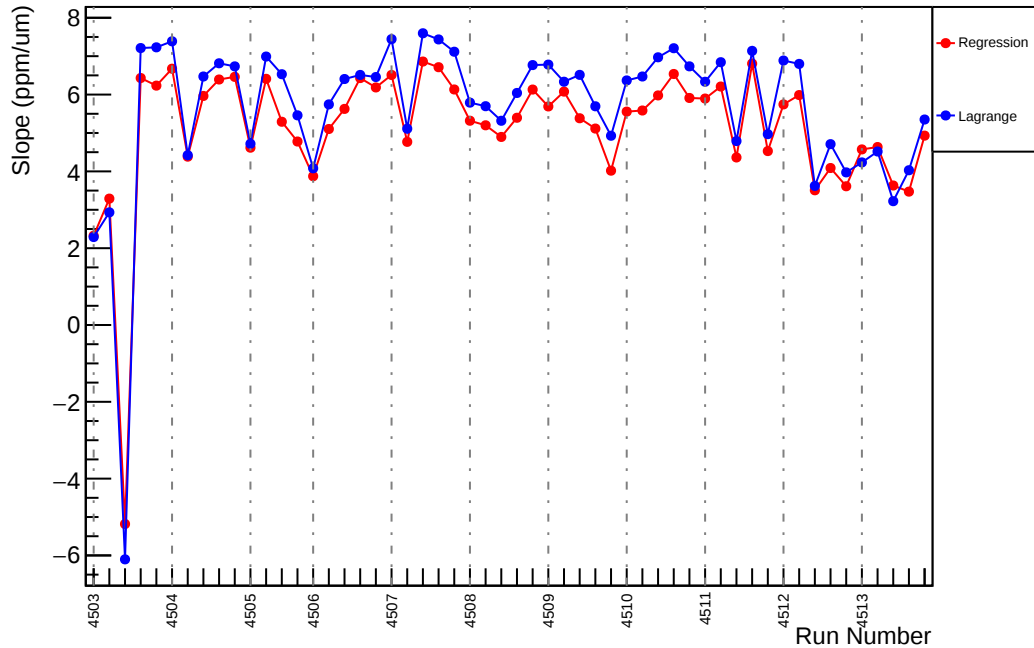
Slug63: Slope : us_dd_vs_evMon3 (ppm/um)
