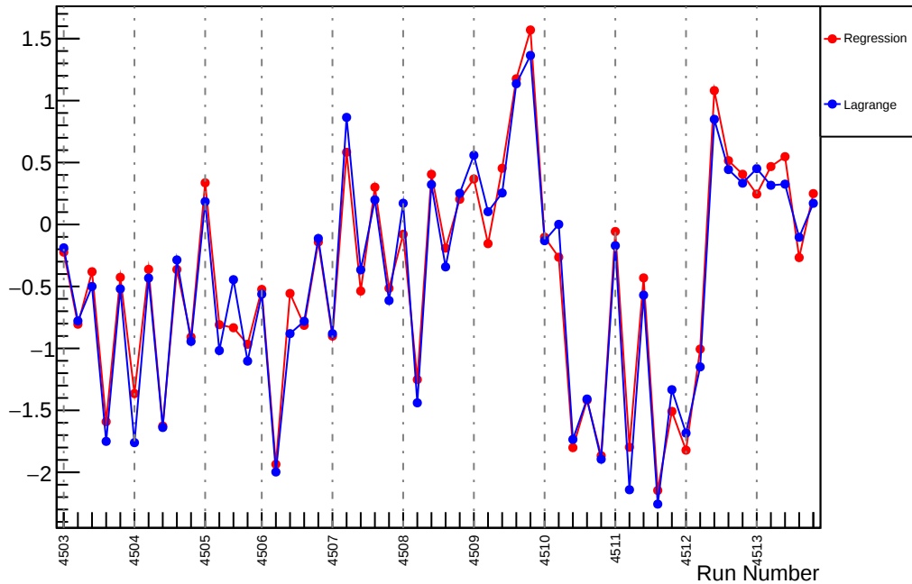
Slug63: Slope : us_dd_vs_evMon2 (ppm/um)
