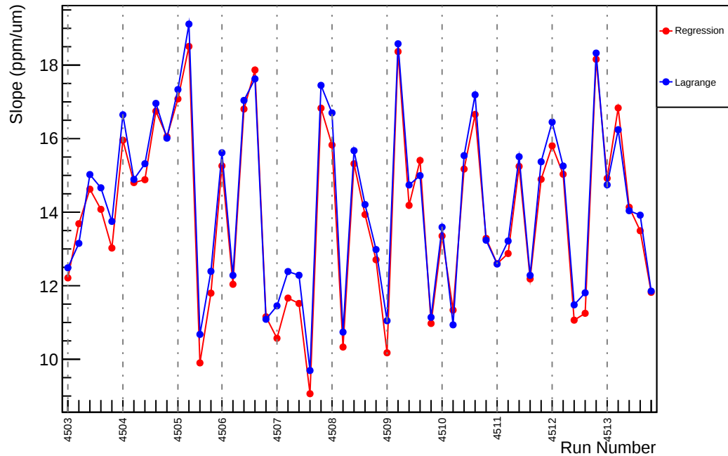
Slug63: Slope : us_dd_vs_evMon7 (ppm/um)
