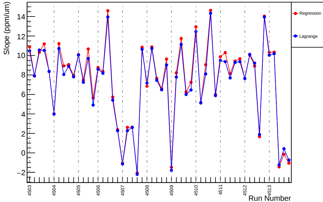
Slug63: Slope : us_dd_vs_evMon9 (ppm/um)
