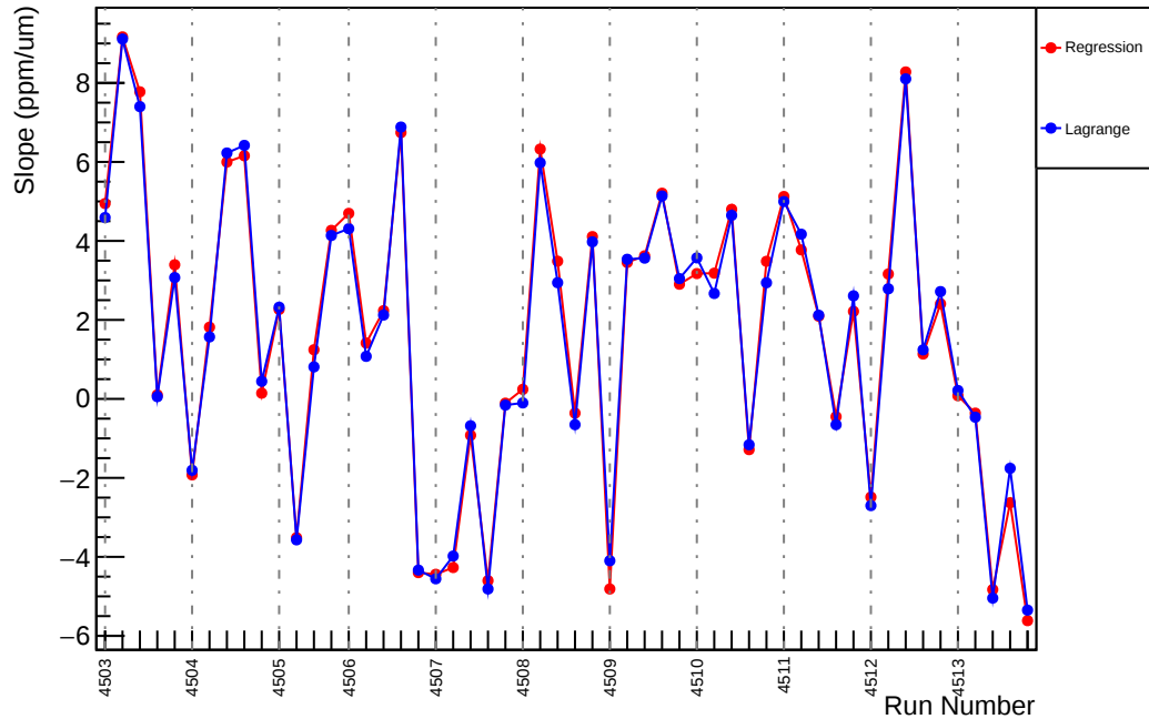
Slug63: Slope : us_dd_vs_evMon8 (ppm/um)
