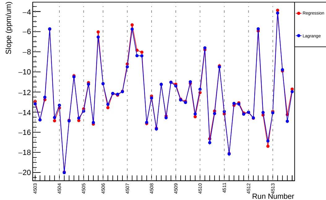
Slug63: Slope : us_dd_vs_evMon11 (ppm/um)
