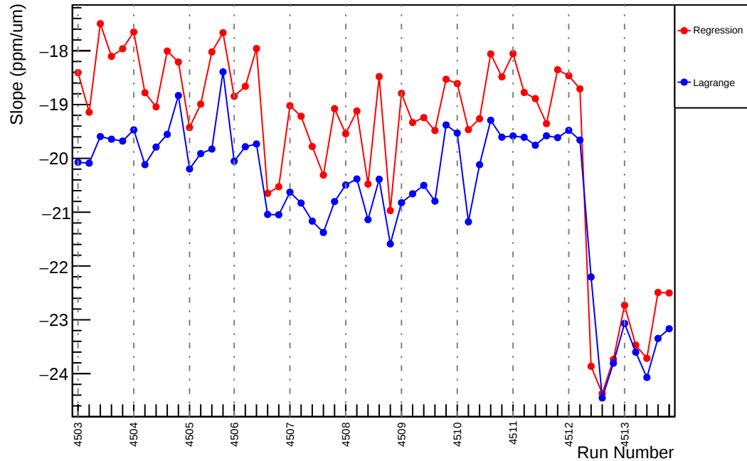
Slug63: Slope : usr_vs_evMon3 (ppm/um)
