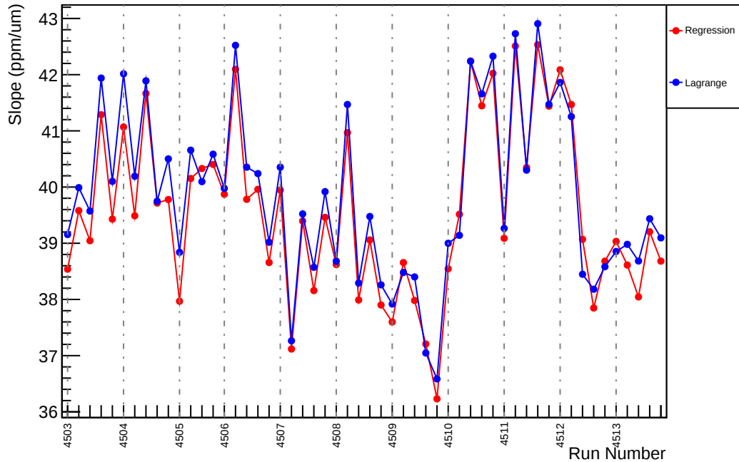
Slug63: Slope : usr_vs_evMon2 (ppm/um)
