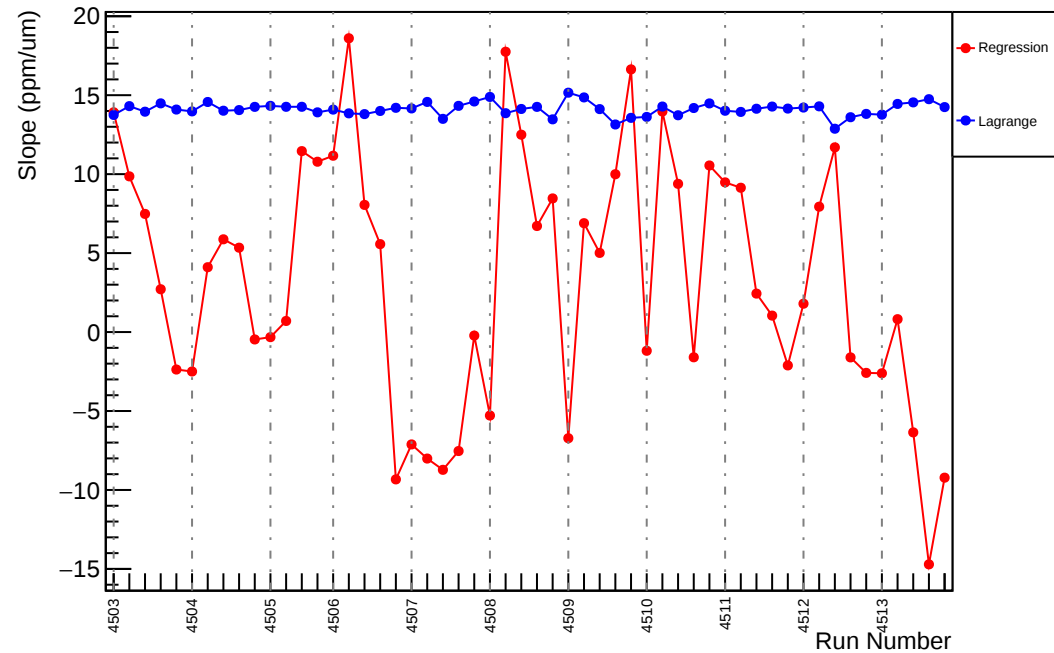
Slug63: Slope : usr_vs_evMon4 (ppm/um)
