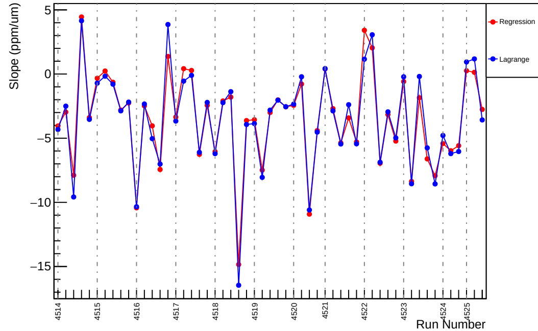
Slug64: Slope : us_avg_vs_evMon10 (ppm/um)
