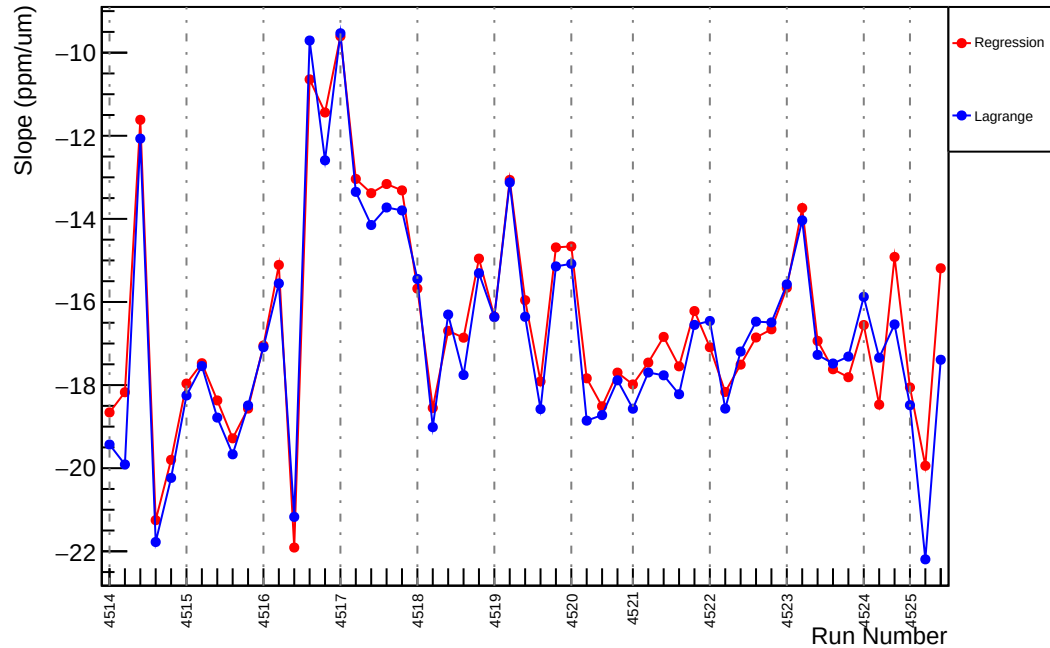
Slug64: Slope : us_avg_vs_evMon6 (ppm/um)
