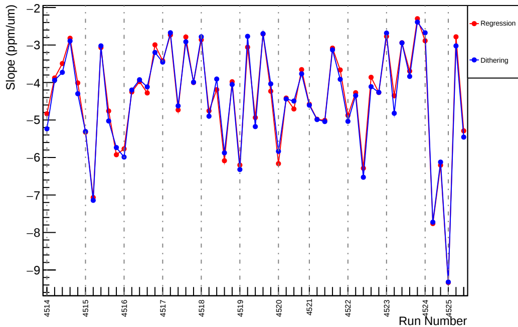
Slug64: Slope : us_dd_vs_evMon2 (ppm/um)
