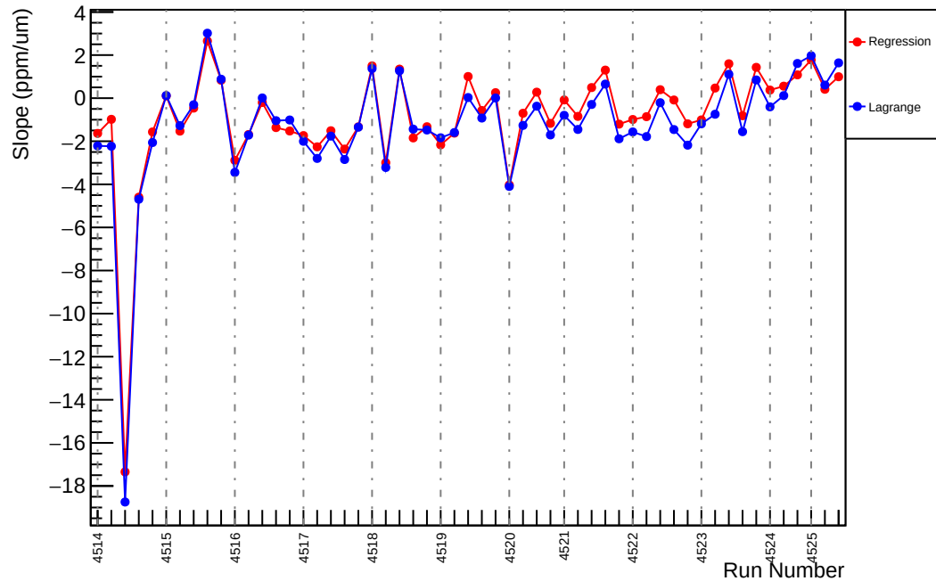
Slug64: Slope : us_dd_vs_evMon6 (ppm/um)
