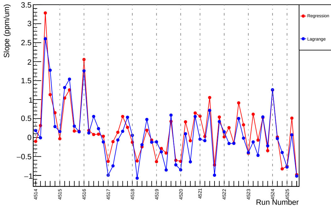
Slug64: Slope : us_dd_vs_evMon5 (ppm/um)
