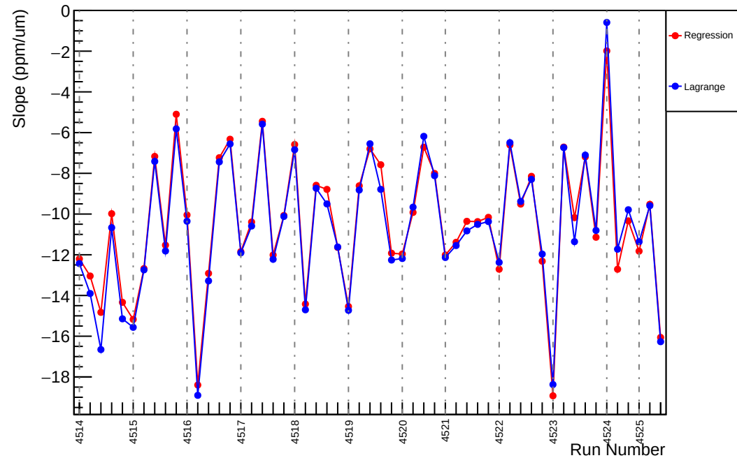
Slug64: Slope : us_dd_vs_evMon11 (ppm/um)
