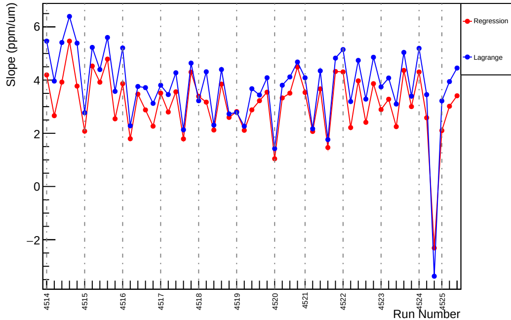
Slug64: Slope : us_dd_vs_evMon4 (ppm/um)
