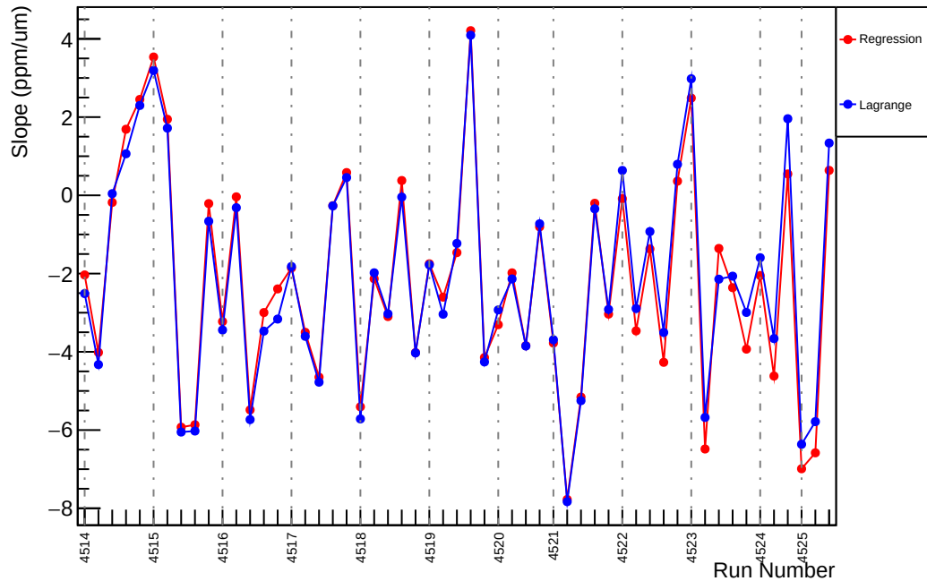
Slug64: Slope : us_dd_vs_evMon10 (ppm/um)
