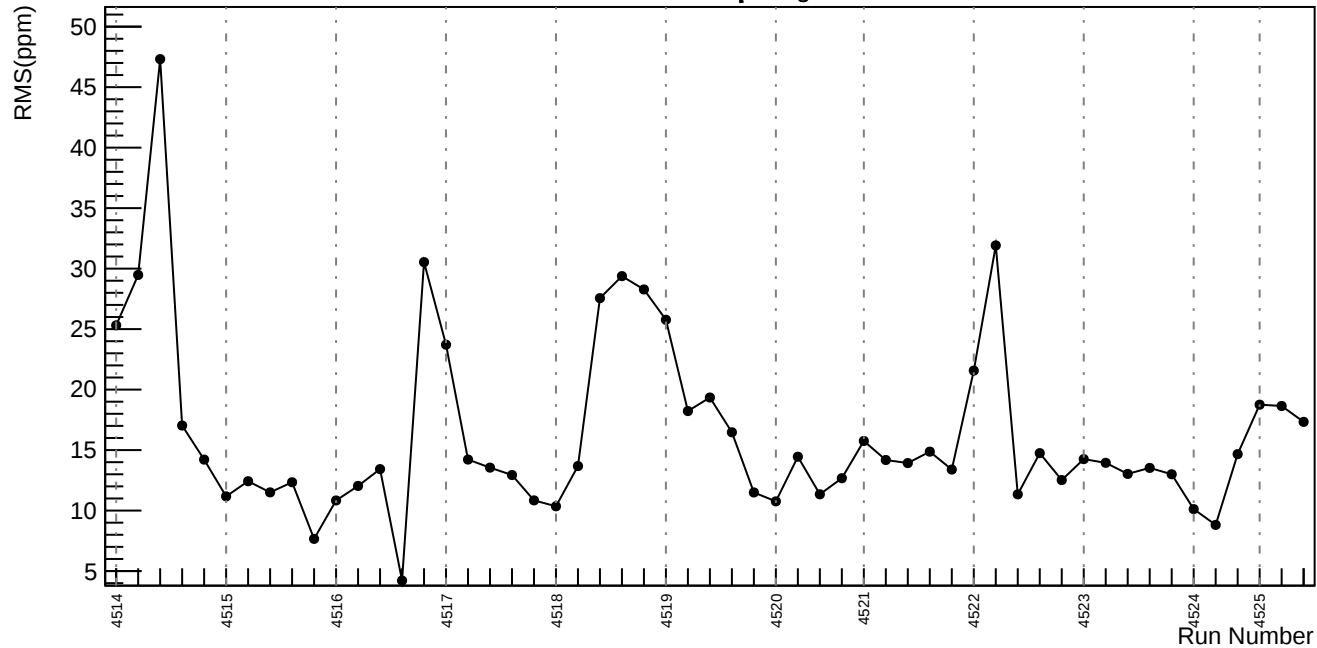
Slug64: asym_usl: \sqrt{\sigma_{\text{lagr}}^2 - \sigma_{\text{reg}}^2} (ppm)
